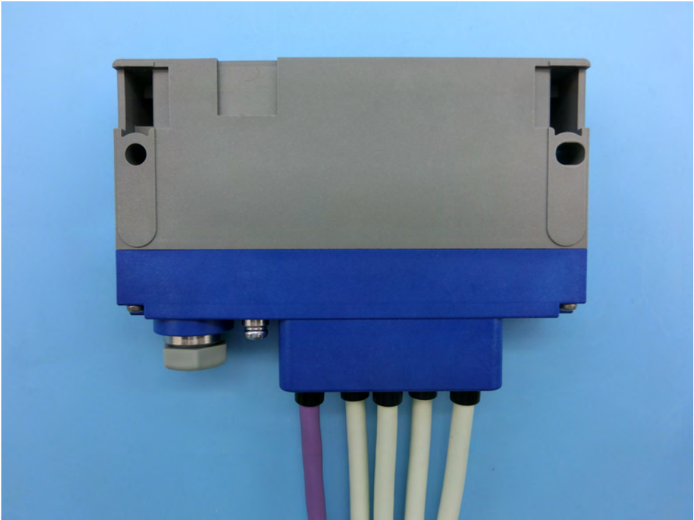
EX600-WLYB1 Back side
