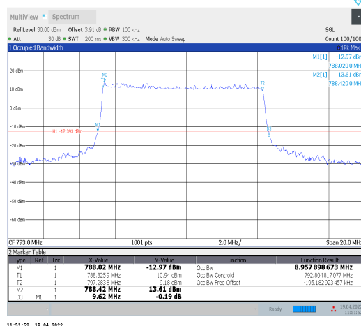
1-N14--15-10-H-3-DFT-16QAM-Outer_Full-50@0-An t0-8.958-9.620-≤10-PASS
