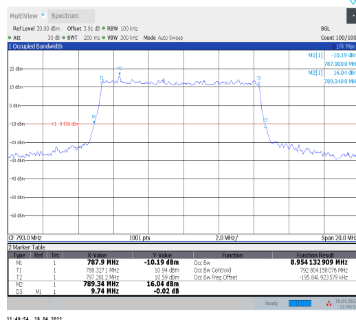
1-N14--15-10-H-1-DFT-QPSK-Outer_Full-50@0-Ant 0-8.954-9.740≤10-PASS
