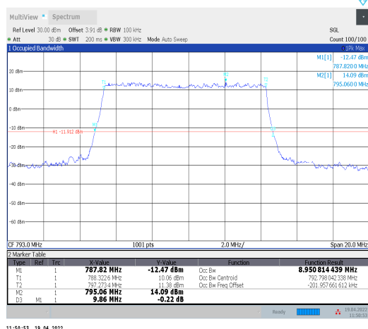
1-N14--15-10-H-2-DFT-PI2BPSK-Outer_Full-50@0- Ant0-8.951-9.860-≤10-PASS
