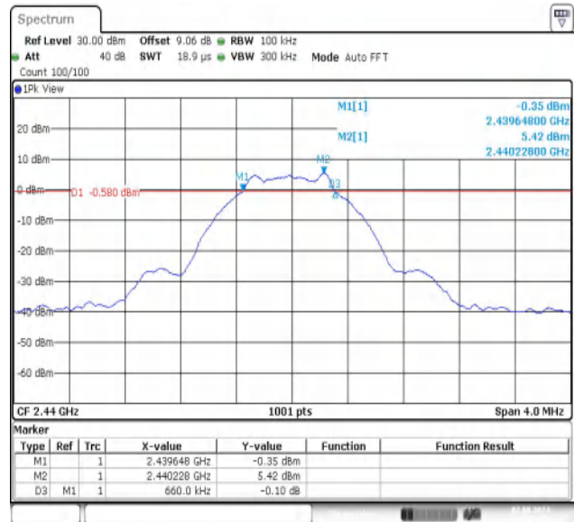
BLE_1M-Ant1-2440-PASS
