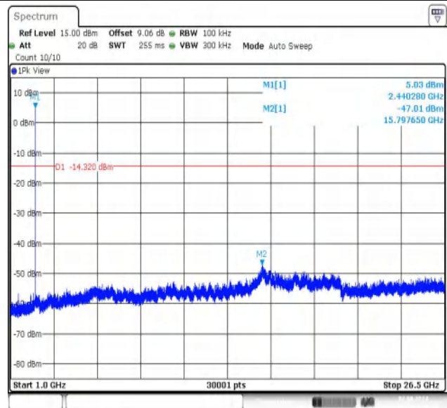
BLE_1M-Ant1-2440-1000~26500-PASS
