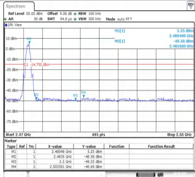
BLE_1M-Ant1-2480-PASS
