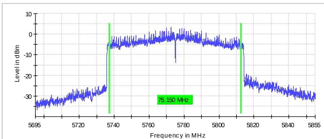
6 dB Bandwidth
