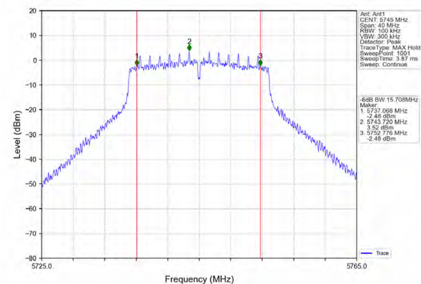
802.11ac(VHT20)_MCH_5785MHz_Ant1_NTNV
