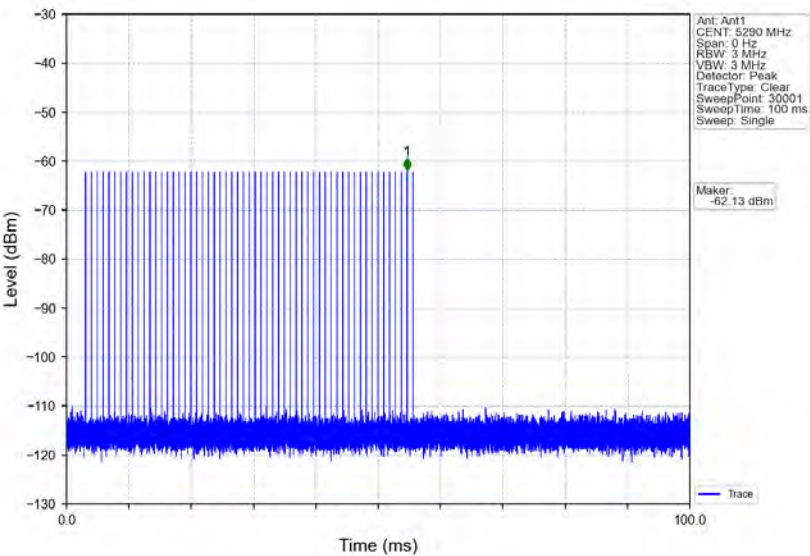
Signal Calibration_802.11ac(VHT80)_2A_5290MHz_RadarType2_Trial0
