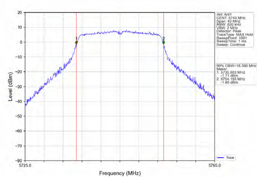
802.11ac(VHT20)_LCH_5745MHz_Ant1_NTNV
