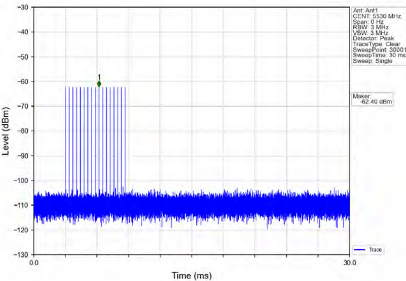
Signal Calibration_802.11ac(VHT80)_2C_5530MHz_RadarType4_Trial0
