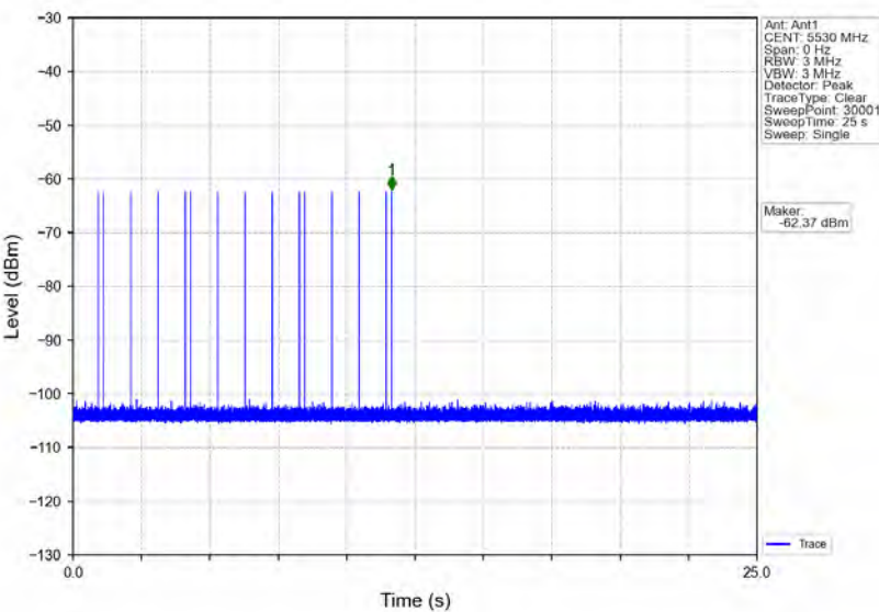
Signal Calibration_802.11ac(VHT80)_2C_5530MHz_RadarType6_Trial0
