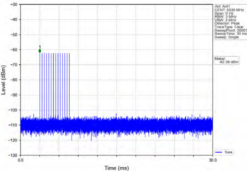
Signal Calibration_802.11ac(VHT80)_2C_5530MHz_RadarType5_Trial0
