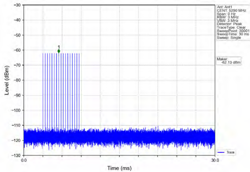
Signal Calibration_802.11ac(VHT80)_2A_5290MHz_RadarType4_Trial0
