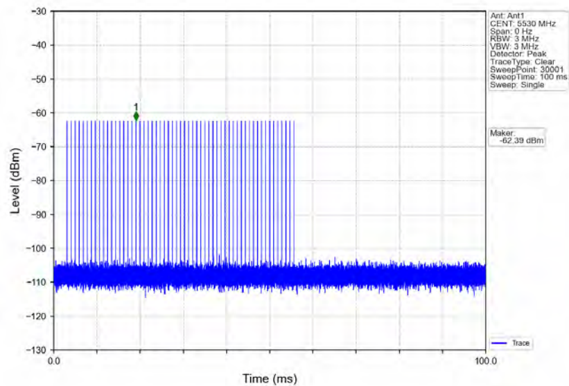
Signal Calibration_802.11ac(VHT80)_2C_5530MHz_RadarType2_Trial0
