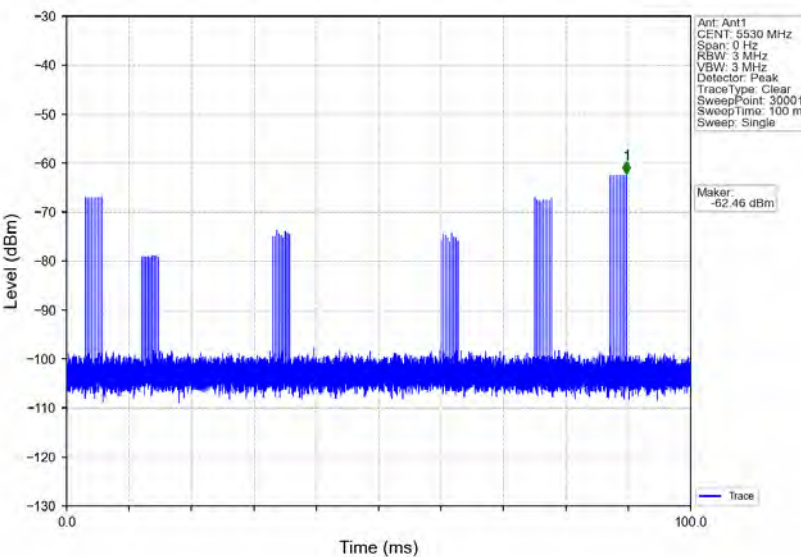
Signal Calibration_802.11ac(VHT80)_2C_5530MHz_RadarType6_Trial0
