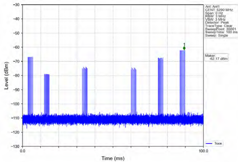
Signal Calibration_802.11ac(VHT80)_2A_5290MHz_RadarType6_Trial0
