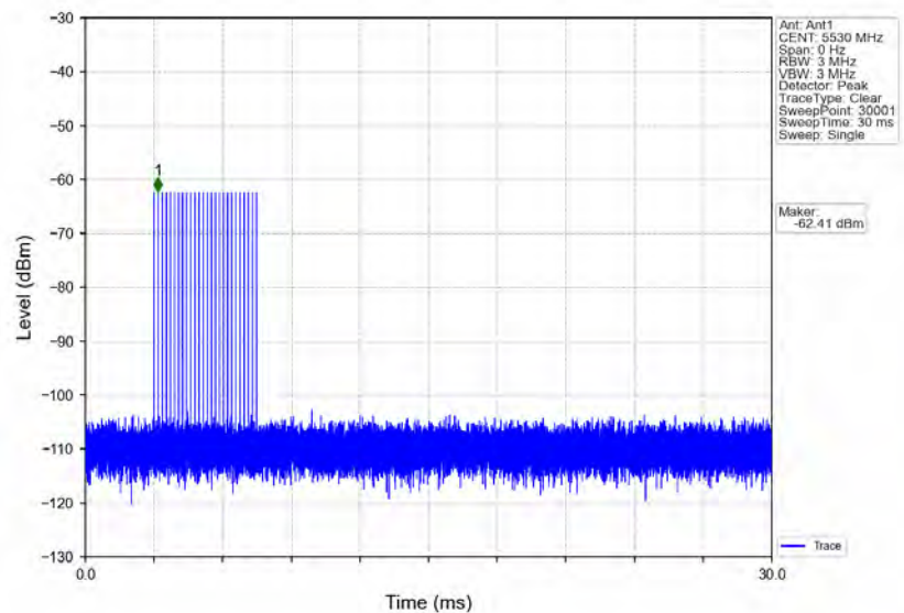
Signal Calibration_802.11ac(VHT80)_2C_5530MHz_RadarType3_Trial0
