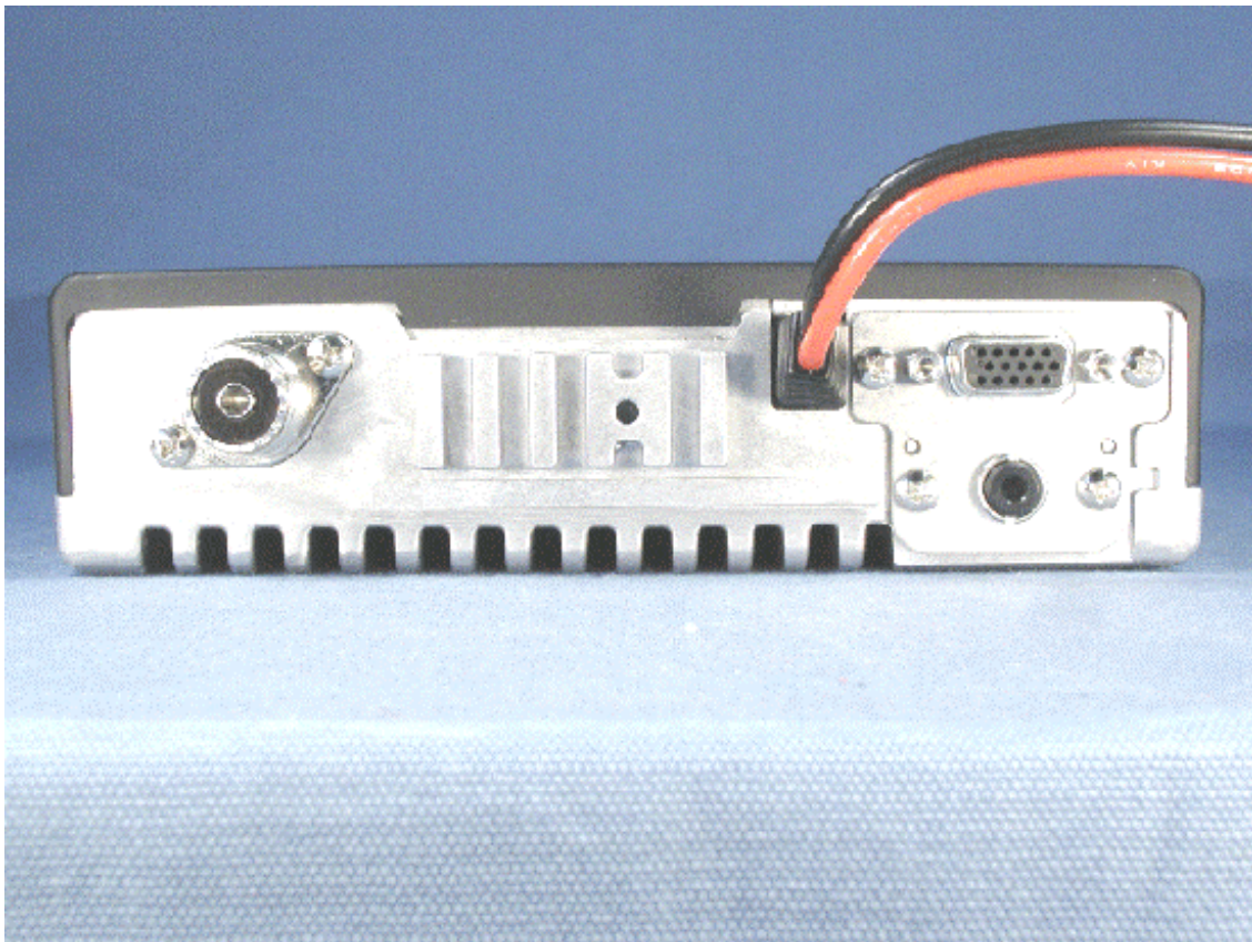
Rear view
