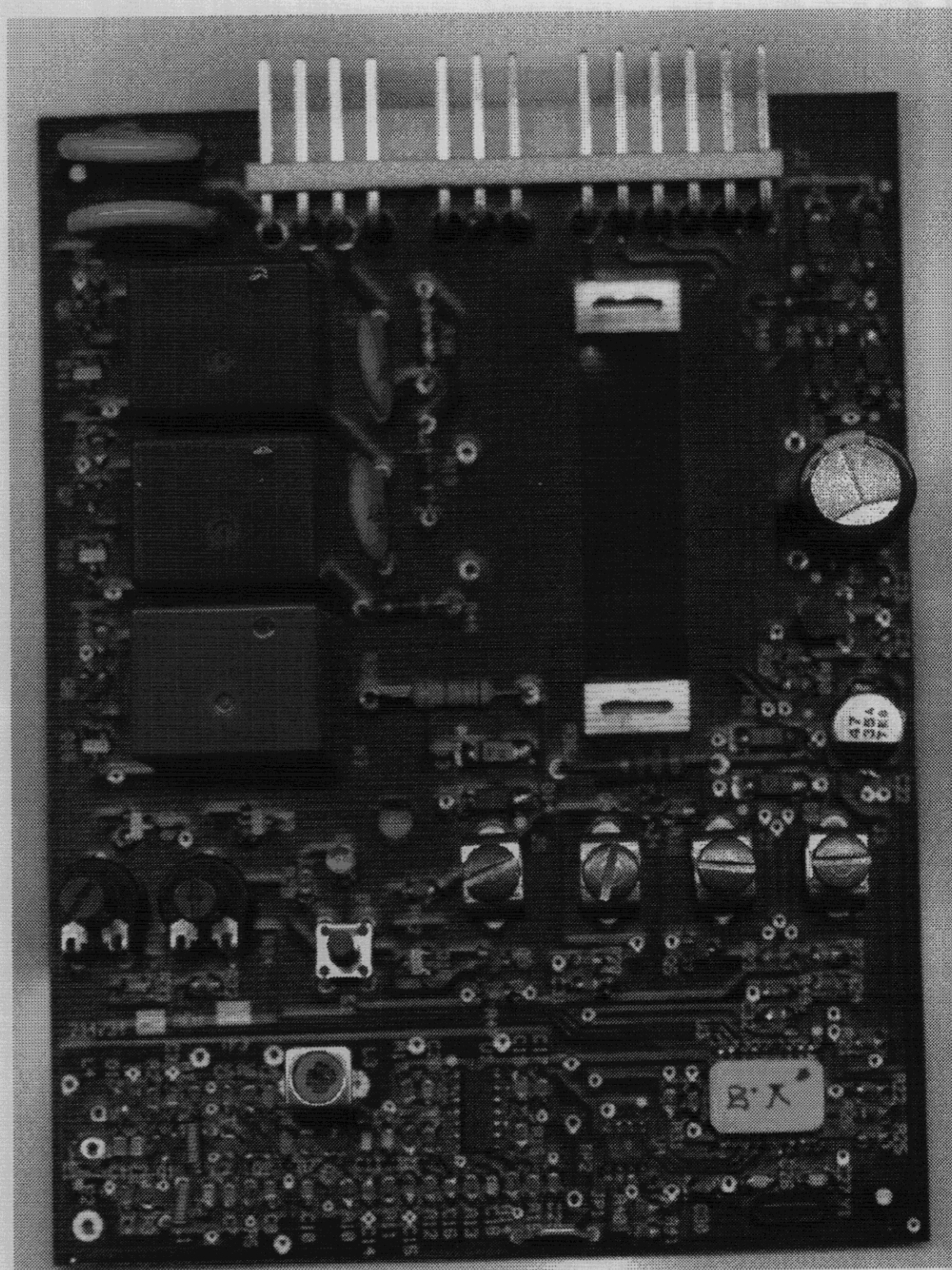
FCC ID: EF4 AAE00407 PCB COMPONENT SIDE POWER TRANSFORMER REMOVED FOR PICTURE CLARITY
