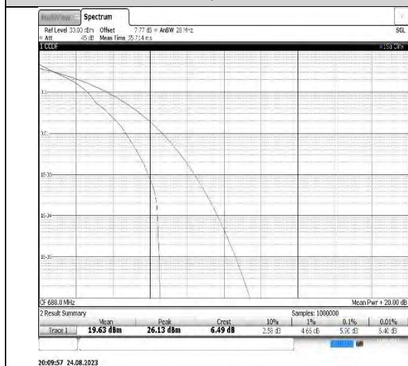
Band71-20MHz-16QAM-133222-1RB#0
