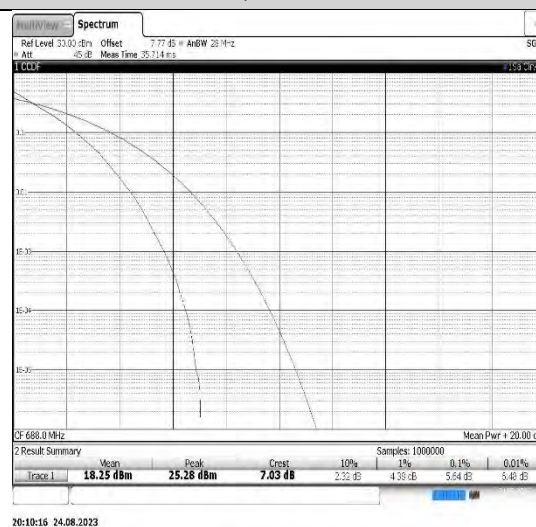
Band71-20MHz-16QAM-133222-100RB#0
