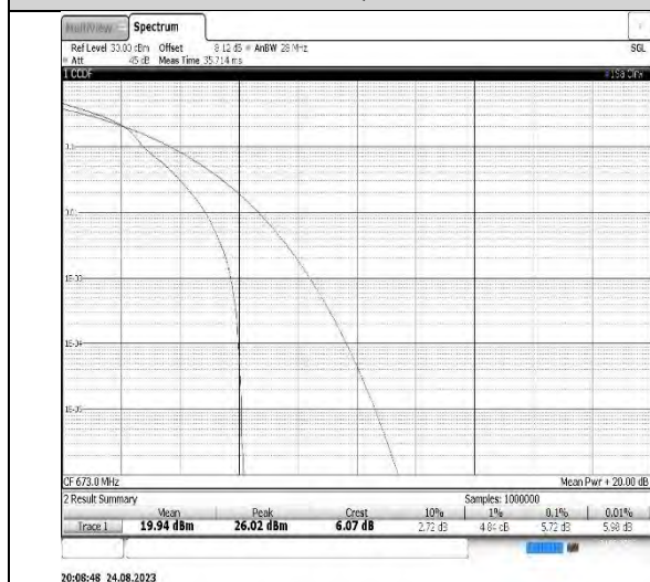
Band71-20MHz-16QAM-133322-1RB#0
