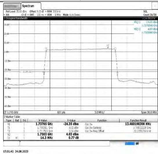
Band66-20MHz-16QAM-132322-100RB#0
