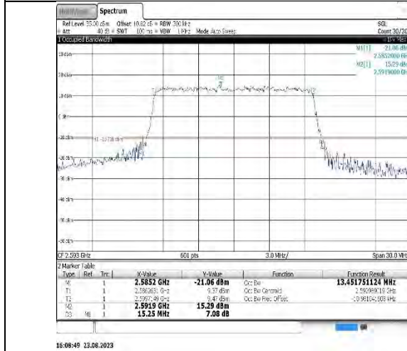
Band41-20MHz-QPSK-40620-100RB#0-PASS
