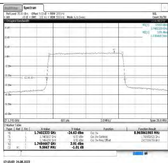
Band66-15MHz-16QAM-132322-75RB#0
