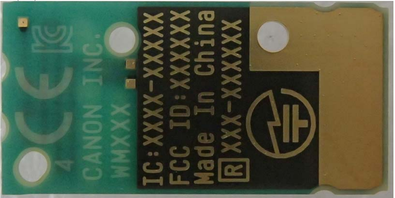
EUT(Rear)
