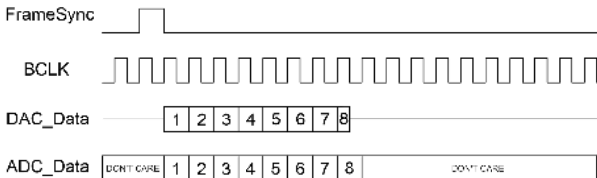
Figure 9: PCM Interface (Short Frame Sync)
