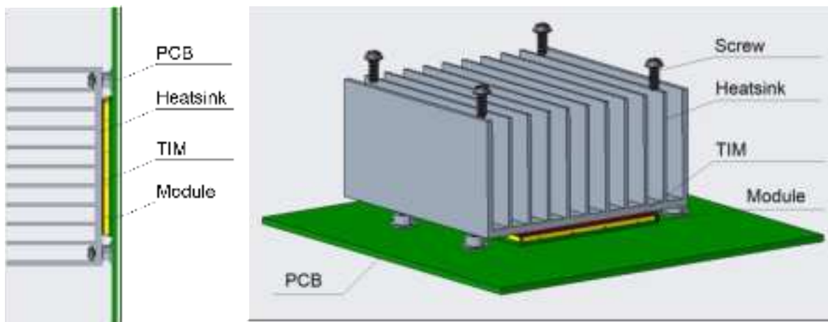
Figure 20: Placement and Fixing of the Heatsink
