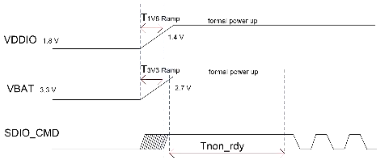
Figure 4: Power-up Timing
