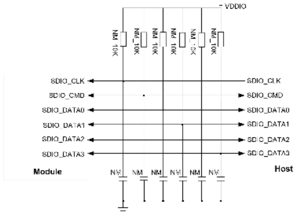
Figure 6: SDIO Interface Connection
