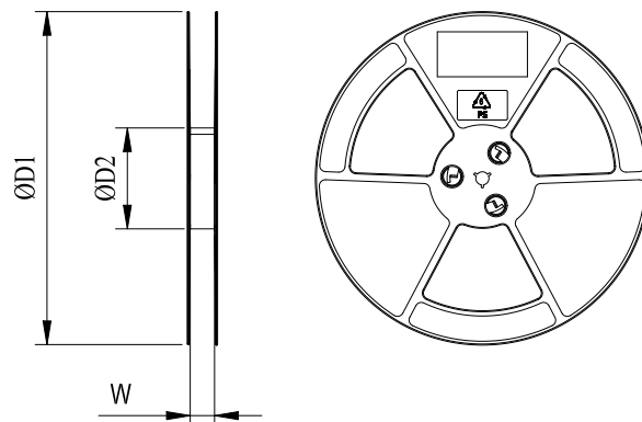
Figure 27: Plastic Reel Dimension Drawing
