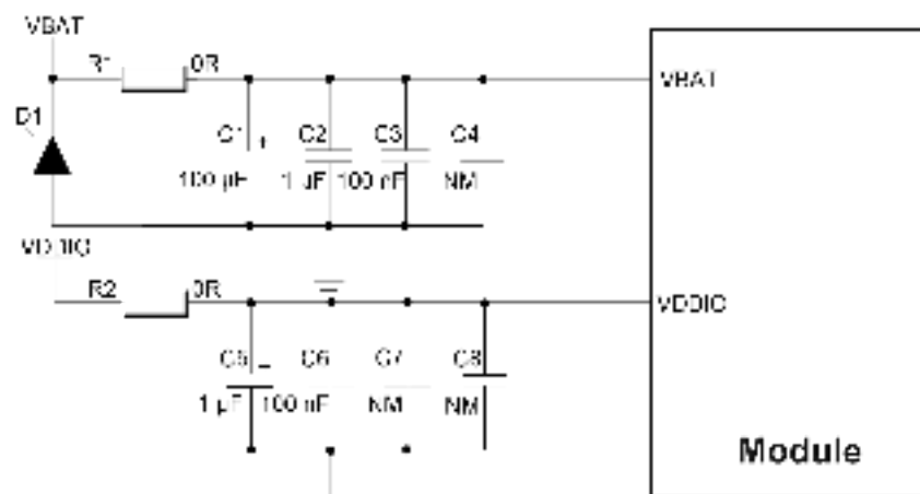
Figure 3: Reference Circuit of Power Supply
