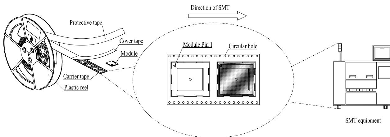
Figure 28: Mounting Direction
