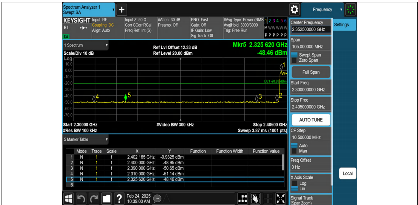
2DH5-Ant1-Hop_2402-PASS
