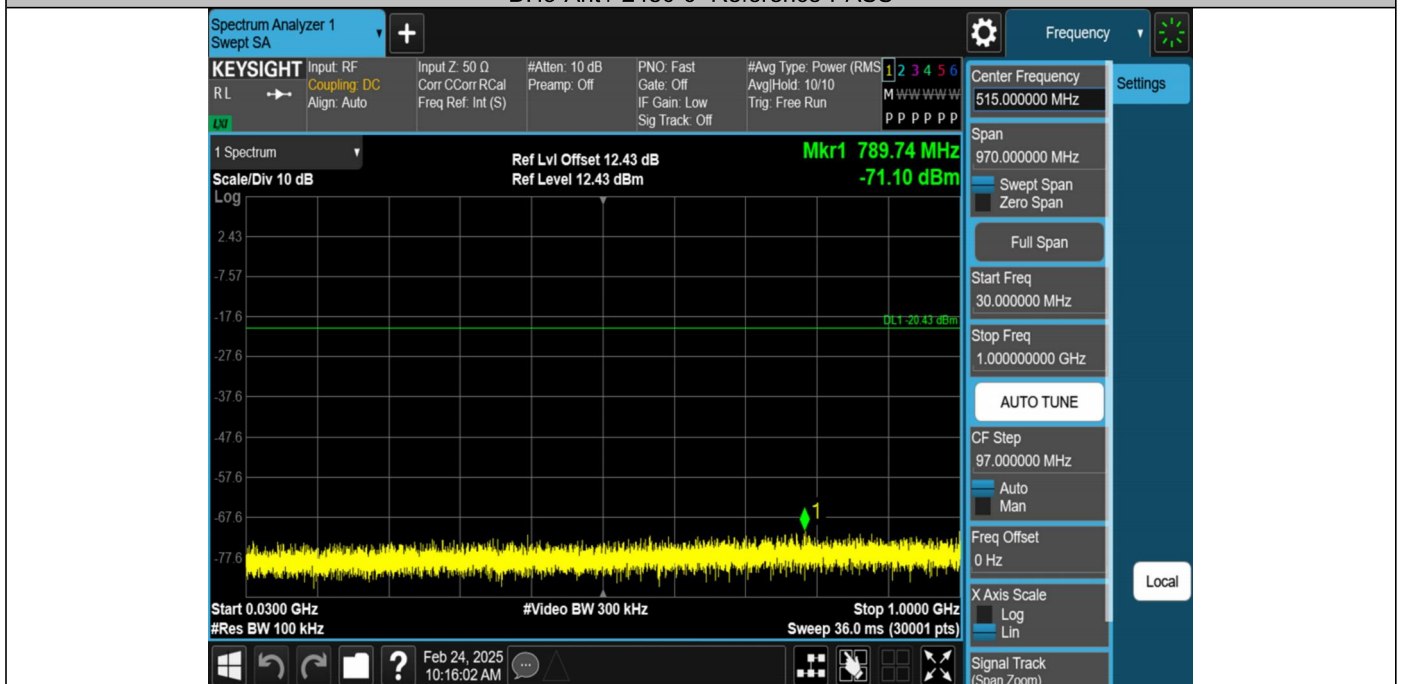
DH5-Ant1-2480-30~1000-PASS
