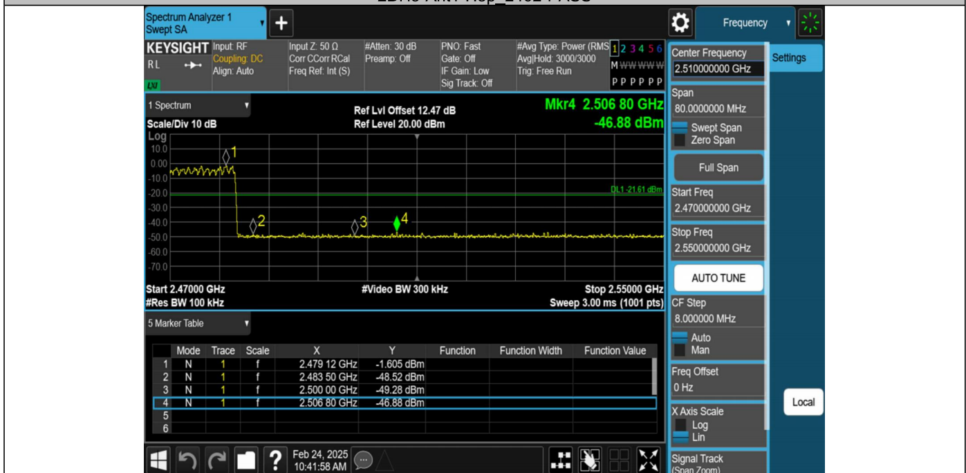
2DH5-Ant1-Hop_2480-PASS
