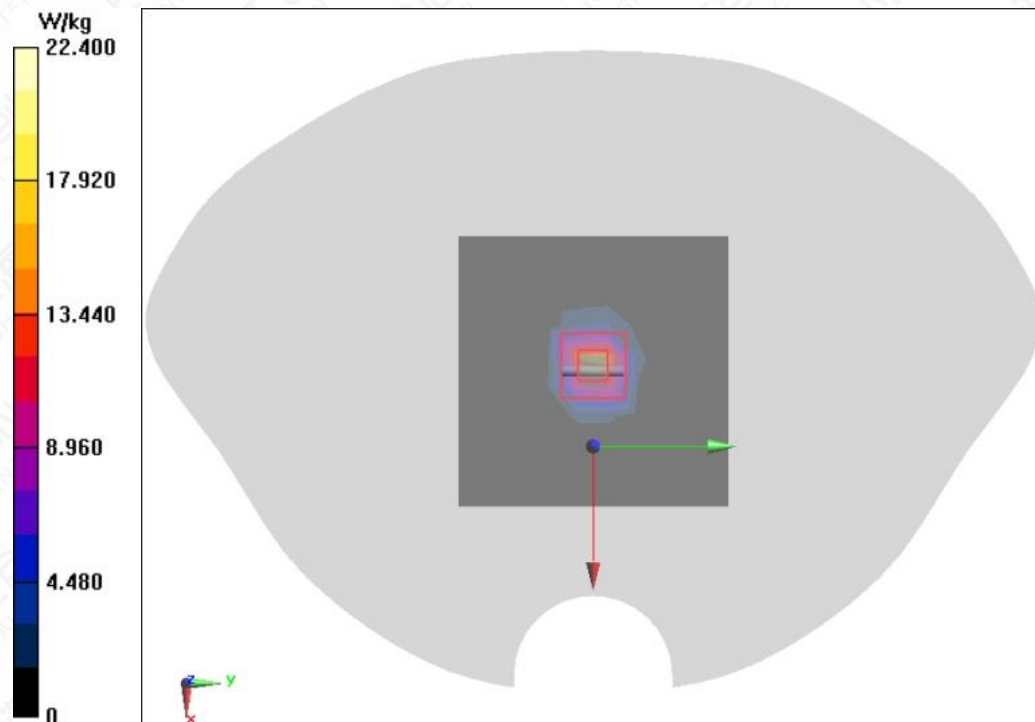
Figure A.2-5 System Check 5600MHz
