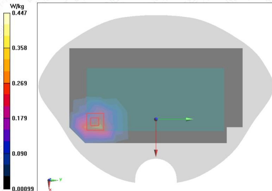
Figure A.1-9 Wi-Fi5G U-NII-1 802.11a Back Side Mode Low 10mm
