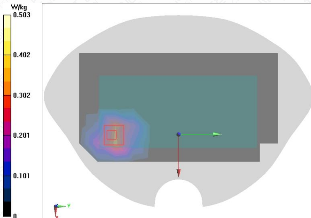
Figure A.1-12 Wi-Fi5G U-NII-2A 802.11a Back Side Mode High 10mm
