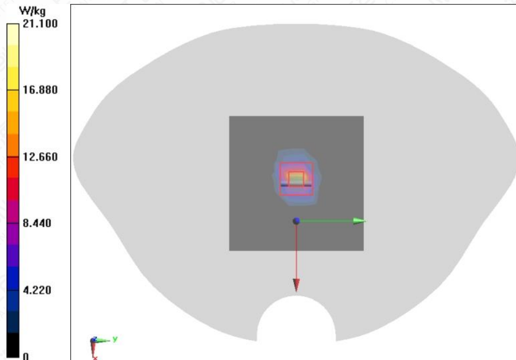
Figure A.2-6 System Check 5800MHz
