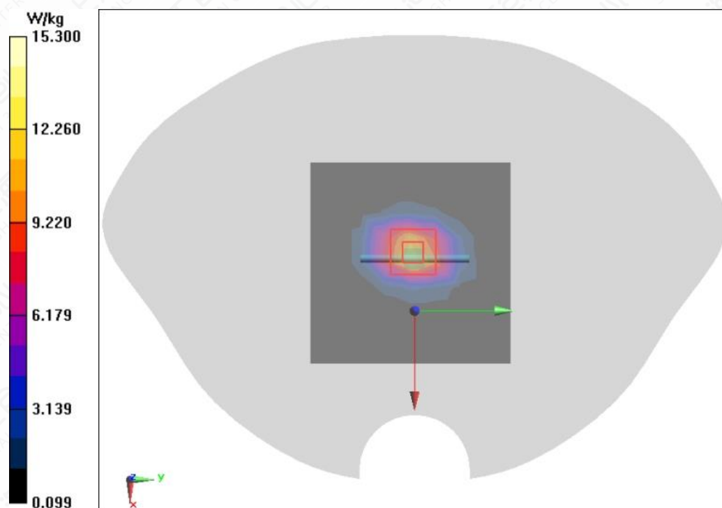
Figure A.2-2 System Check 2450MHz
