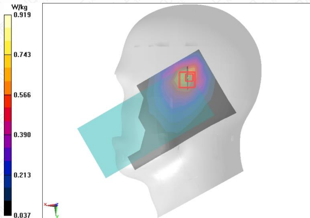
Figure A.1-1 Wi-Fi HaLow 1M Right Cheek Mode Low
