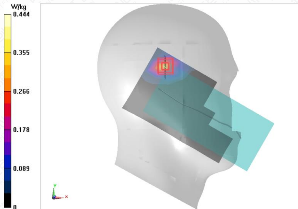
Figure A.1-11 Wi-Fi5G U-NII-2A 802.11a Left Touch Mode Low
