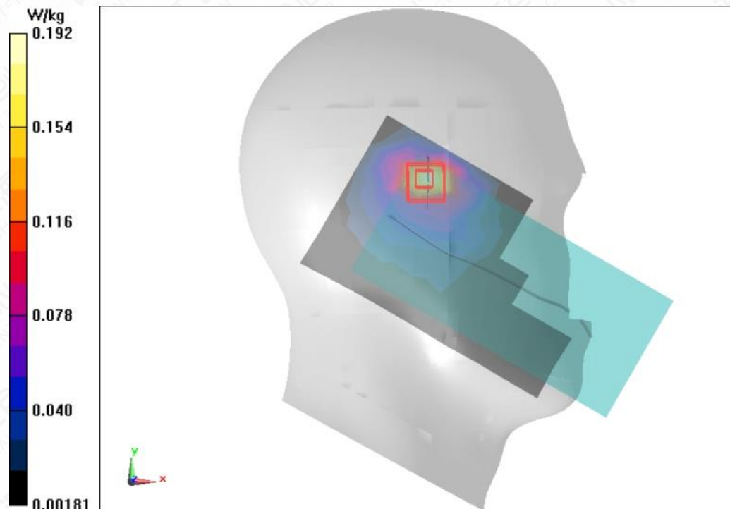
Figure A.1-20 BT DH5 Left Touch Mode Low
