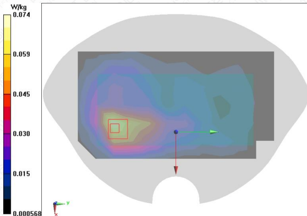
Figure A.1-21 BT DH5 Back Side Mode Low 10mm
