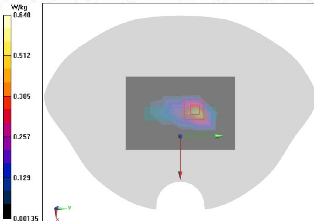
Figure A.1-23 BT DH5 Top Side Mode Low 0mm
