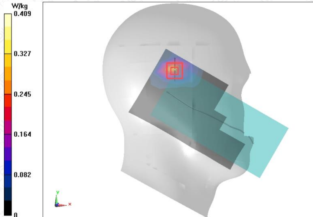
Figure A.1-8 Wi-Fi5G U-NII-1 802.11a Left Touch Mode High
