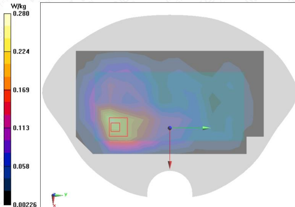
Figure A.1-5 Wi-Fi2.4G 802.11b Back Side Mode Low 10mm
