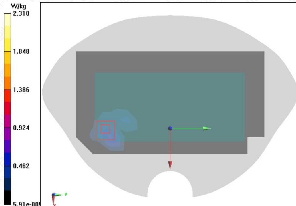
Figure A.1-13 Wi-Fi5G U-NII-2A 802.11a Back Side Mode High 0mm
