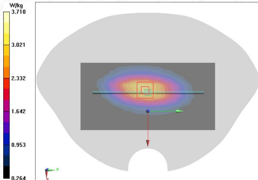
Figure A.2-1 System Check 900MHz
