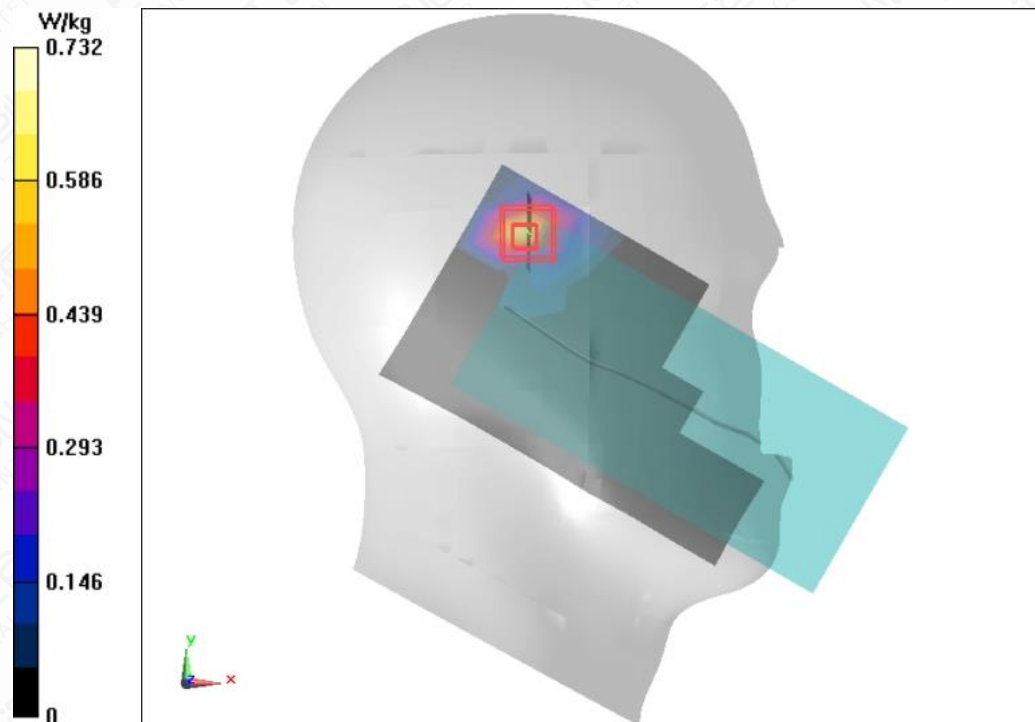
Figure A.1-14 Wi-Fi5G U-NII-2C 802.11n40 Left Touch Mode High
