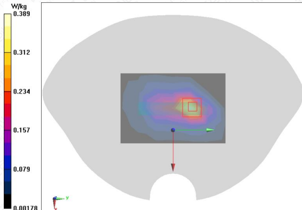
Figure A.1-6 Wi-Fi2.4G 802.11b Top Side Mode High 10mm
