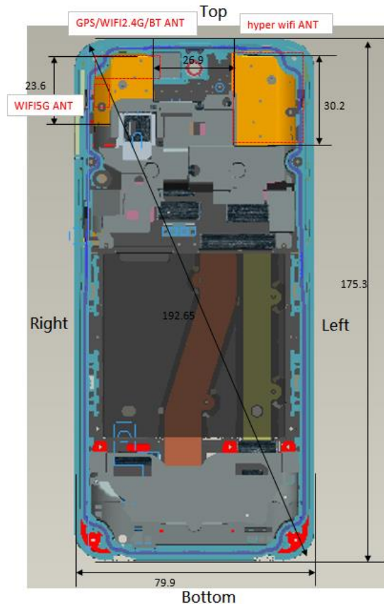
Figure 12.2-1 Antenna Locations (back view)
