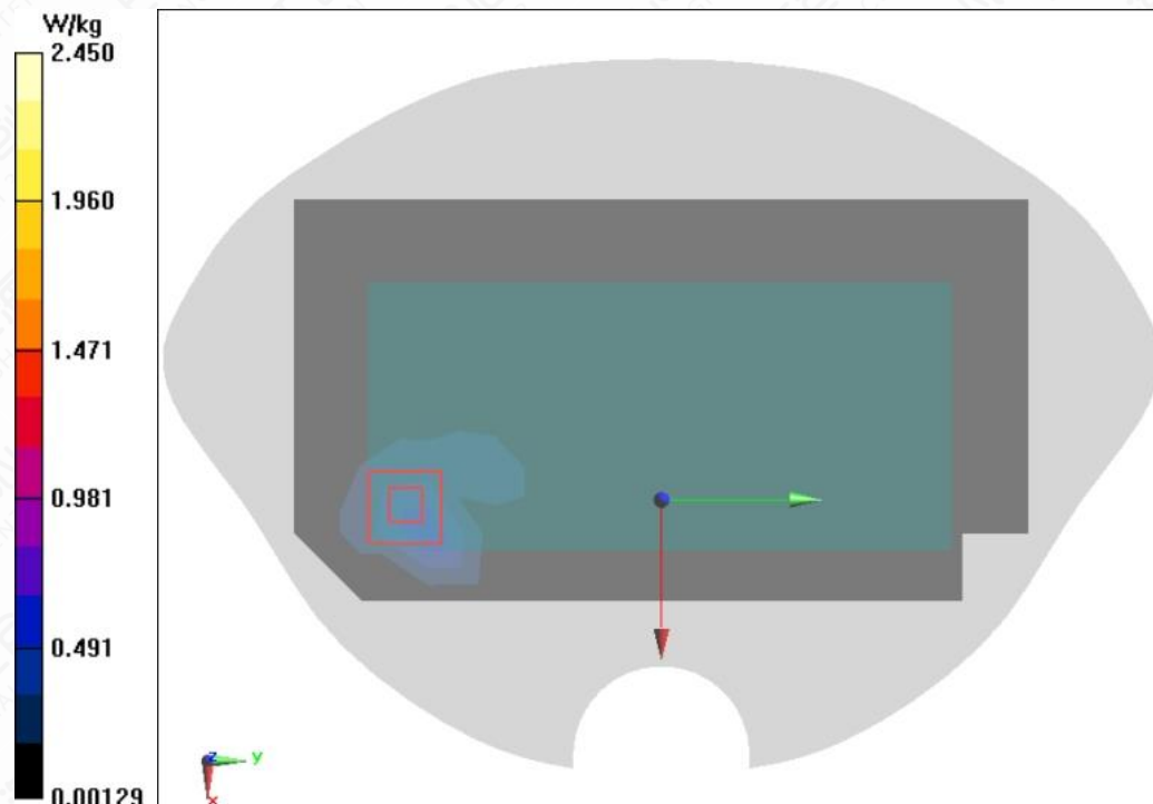
Figure A.1-10 Wi-Fi5G U-NII-1 802.11a Back Side Mode High 0mm
