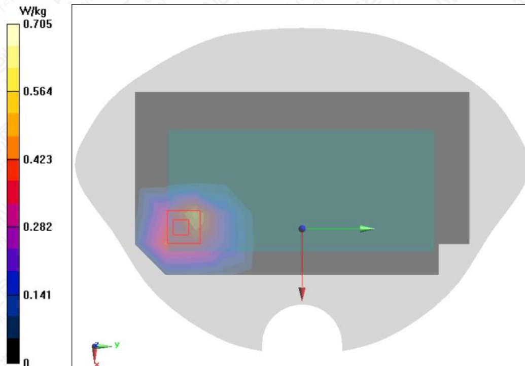
Figure A.1-15 Wi-Fi5G U-NII-2C 802.11n40 Back Side Mode High 10mm
