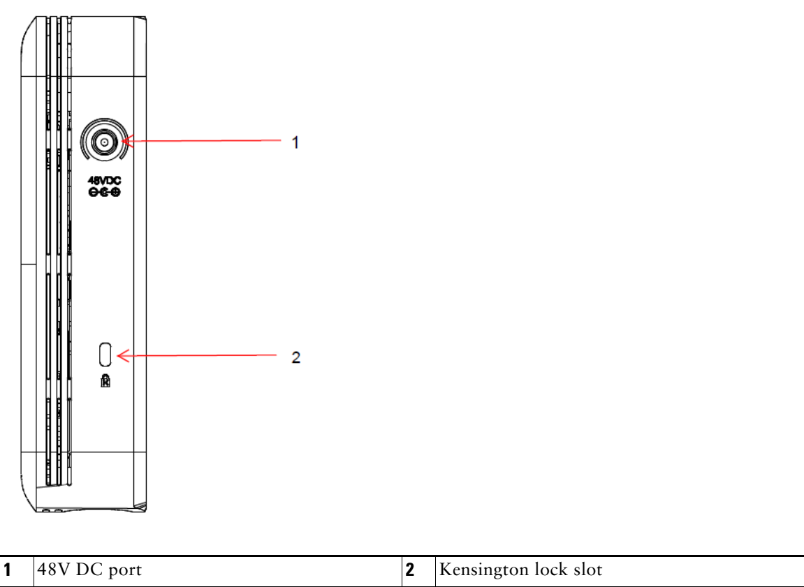
Figure 5 Access Point Ports and Connections on the Left of the AP
