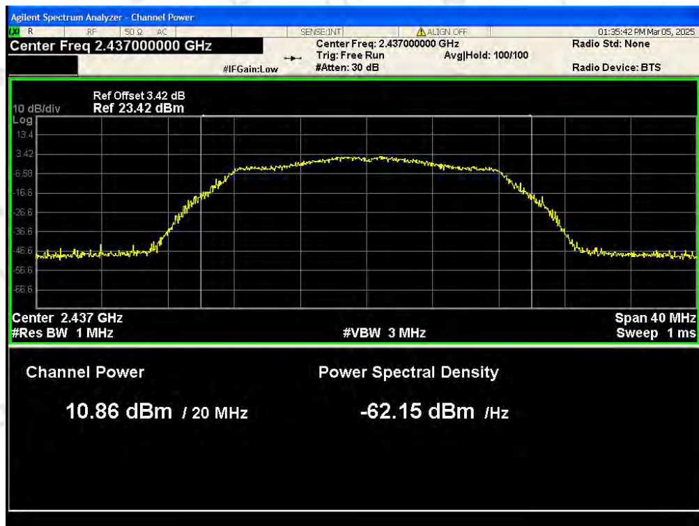
Power NVNT 802.11g 2437MHz Ant1
