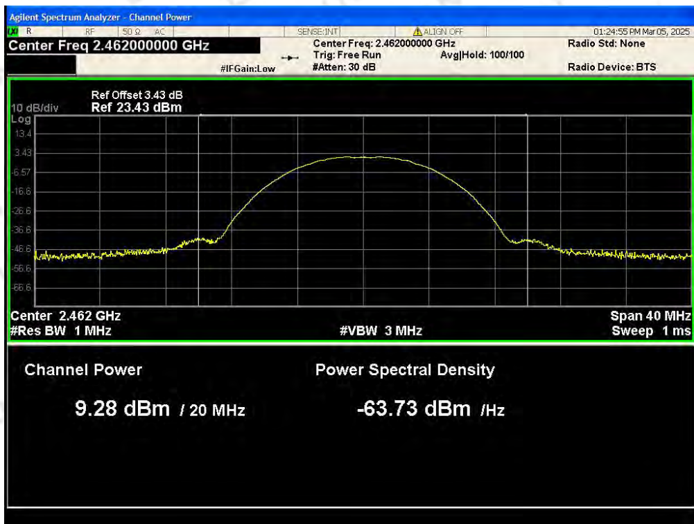
Power NVNT 802.11b 2462MHz Ant1
