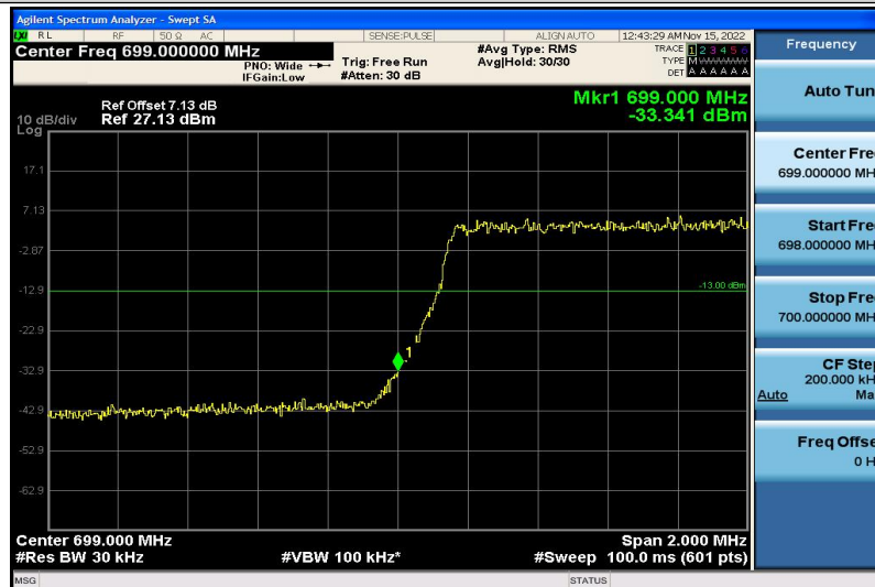
Band12-3MHz-16QAM-23025-15RB#0
