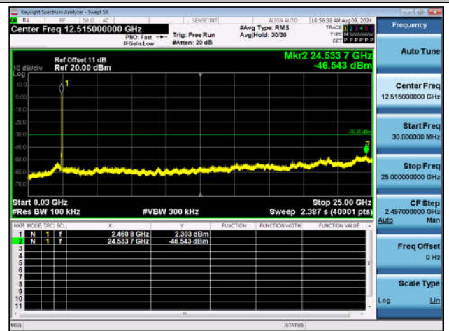
11AX20SISO-Ant1-2462-30~25000-PASS
