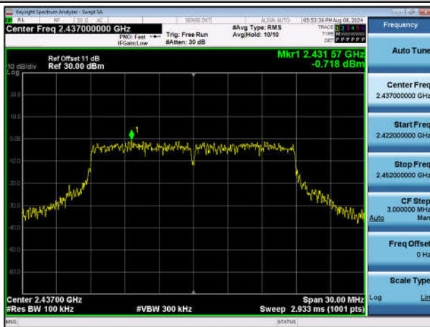
11N20SISO-Ant1-2437-0~Reference-PASS
