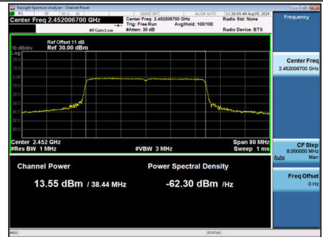
11AX40SISO-Ant1-2452-PASS
