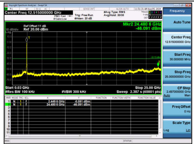
11AX40SISO-Ant1-2452-30~25000-PASS
