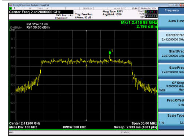
11AX20SISO-Ant1-2412-0~Reference-PASS
