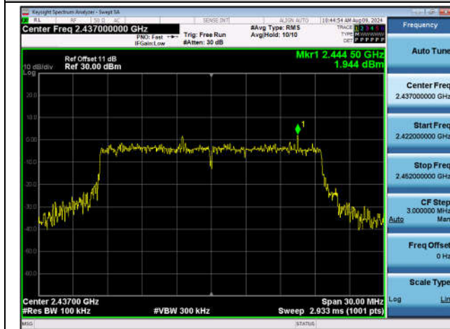
11AX20SISO-Ant1-2437-0~Reference-PASS
