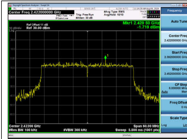
11AX40SISO-Ant1-2422-0~Reference-PASS
