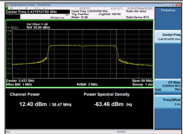
11AX40SISO-Ant1-2422-PASS
