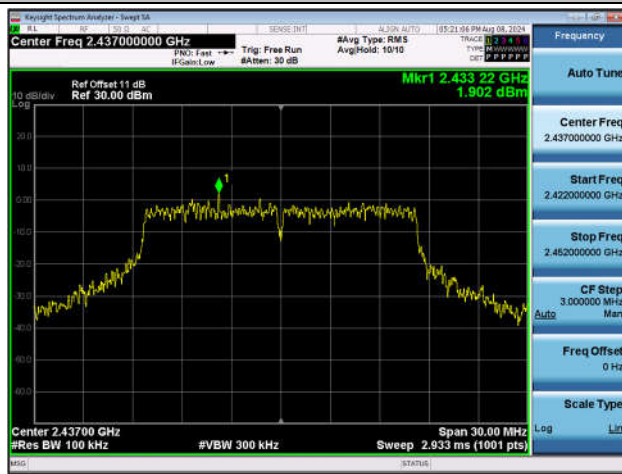
11G-Ant1-2437-0~Reference-PASS
