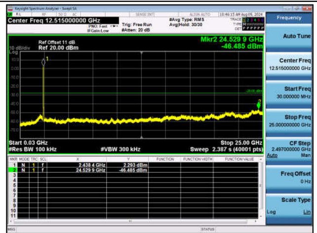
11AX20SISO-Ant1-2437-30~25000-PASS
