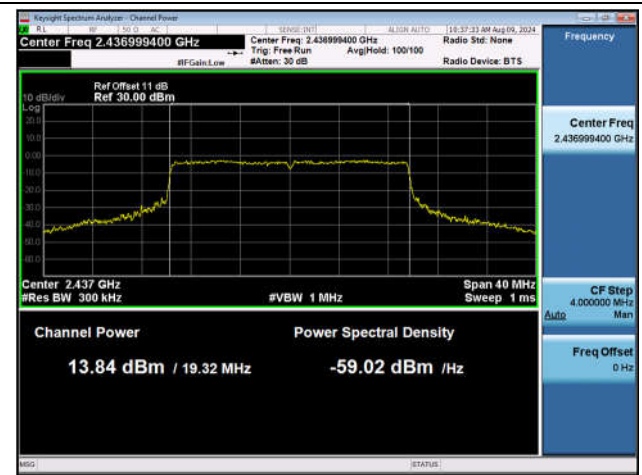
11AX20SISO-Ant1-2437-PASS
