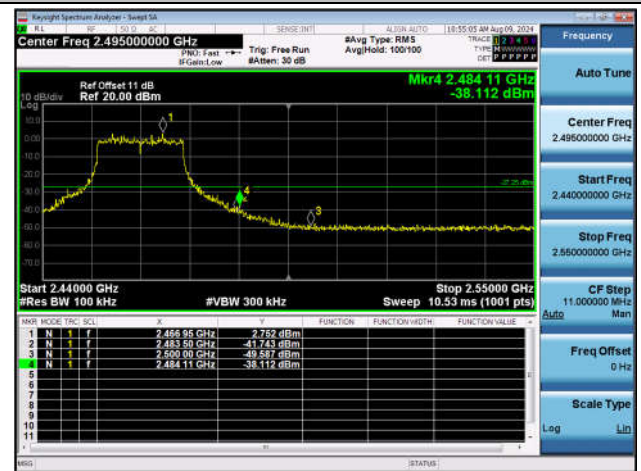
11AX20SISO-Ant1-2462-PASS
