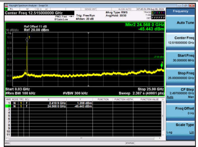
11AX20SISO-Ant1-2412-30~25000-PASS
