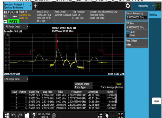
Emission Mask Band7 5MHz QPSK RB1 0 CH21100
