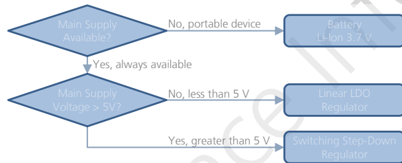
Figure 31: VCC supply concept selection
