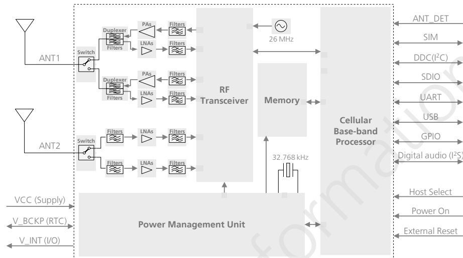
Figure 1: TOBY-L2 series block diagram
