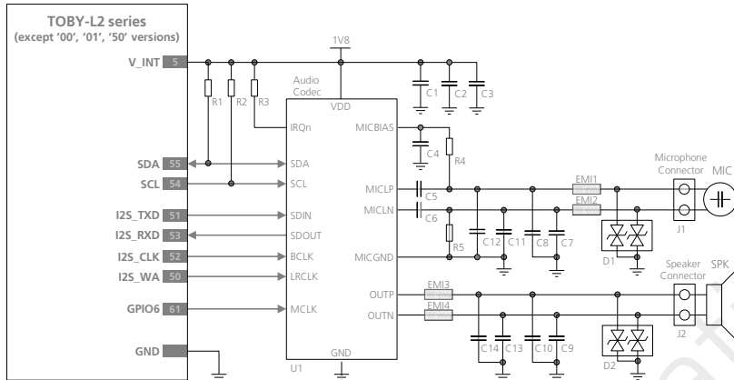
Figure 66: I²S interface application circuit with an external audio codec to provide voice capability
