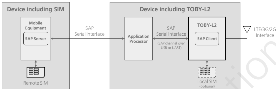
Figure 27: Remote SIM access via completely wired connection
