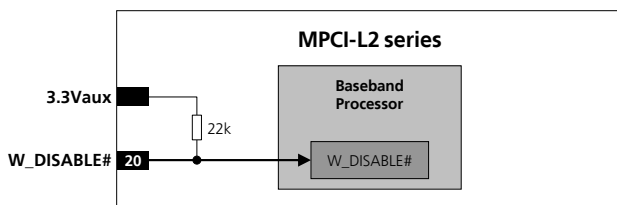
Figure 25: MPCI-L2 series modules W_DISABLE# input circuit description
