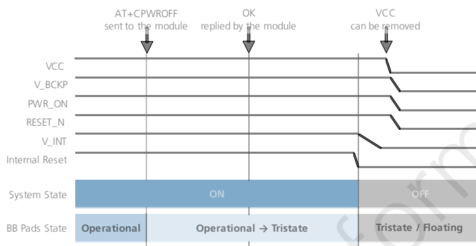
Figure 15: TOBY-L2 series power-off sequence description
