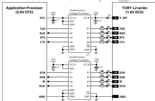
Figure 57: UART interface application circuit with complete V.24 link in DTE/DCE serial communication (3.0 V DTE)
