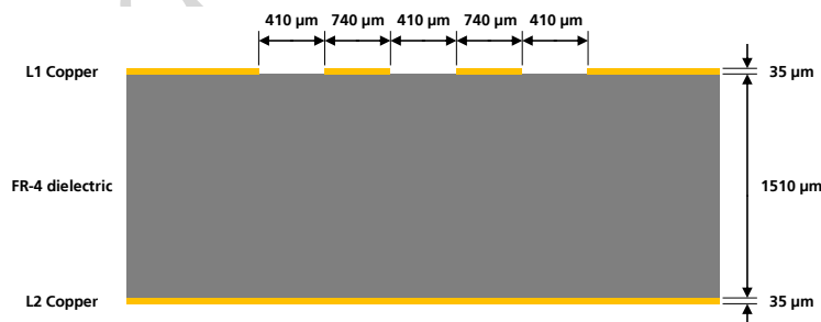
Figure 55: Example of USB line design, with Z_o close to 90 \Omega and Z_{cm} close to 30 \Omega , for the described 2-layer board layup
