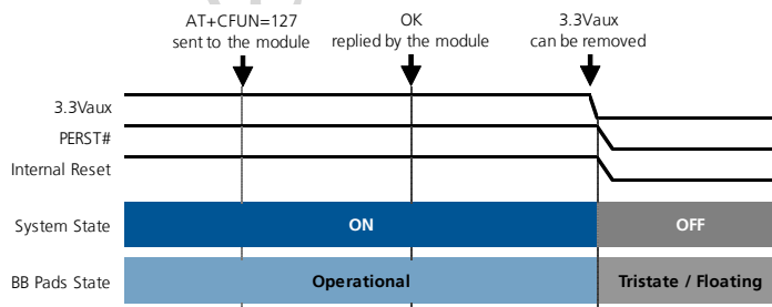
Figure 16: MPC-I-L2 series power-off procedure description
