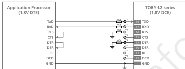
Figure 60: UART interface application circuit with partial V.24 link (3-wire) in the DTE/DCE serial communication (1.8V DTE)
