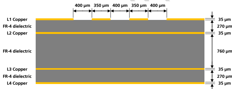
Figure 54: Example of USB line design, with Z_o close to 90 \Omega and Z_{cm} close to 30 \Omega , for the described 4-layer board layup
