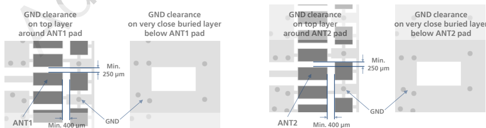
Figure 43: GND keep-out area on top layer around ANT1 / ANT2 pads and on very close buried layer below ANT1 / ANT2 pads
