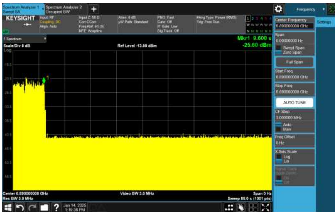
Plot 13: AWGN Signal Detection 320MHz
