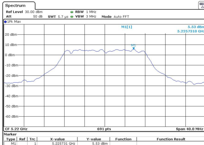
Channel: 44
