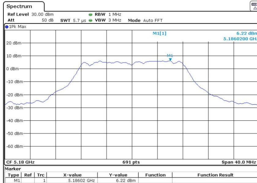
802.11a Channel: 36
