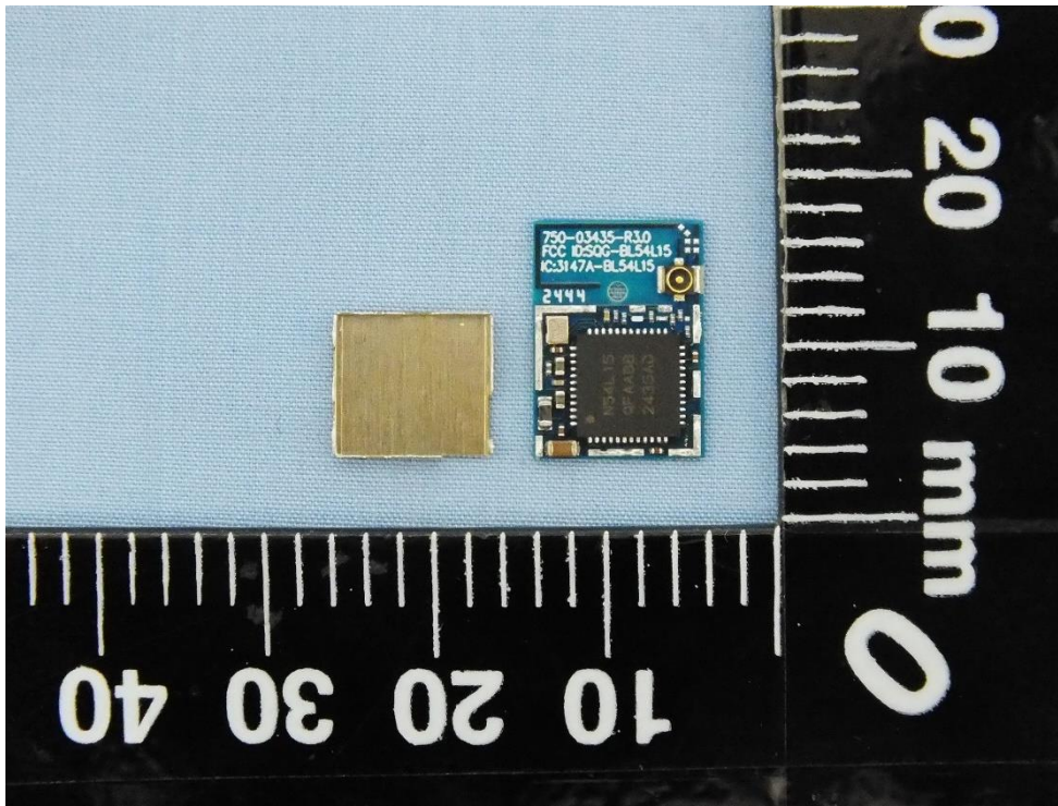
External Antenna
