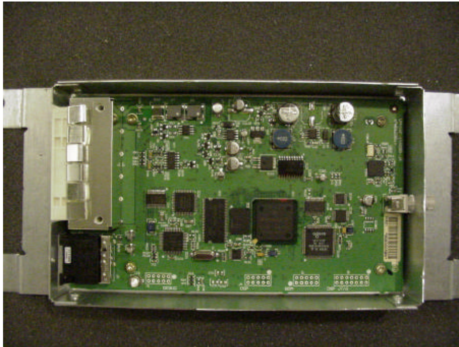
Picture 3 : EUT open case (top view to the PCB)
