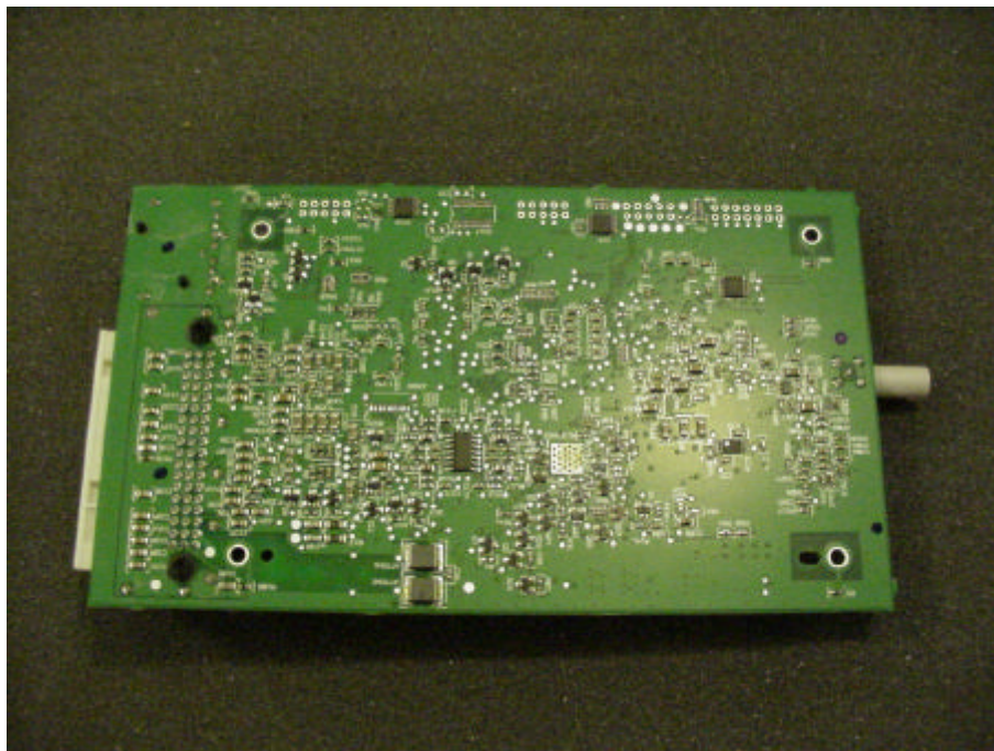
Picture 4 : Removed PCB (bottom view)
