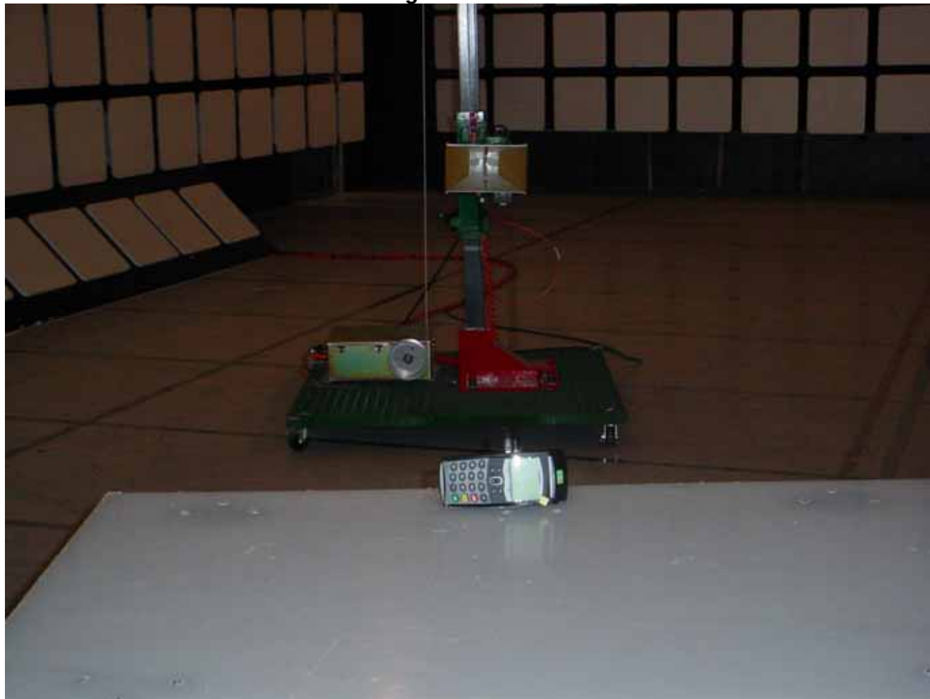
Transmitter Radiated Emissions @ 3 meters Orthogonal Position # 2
