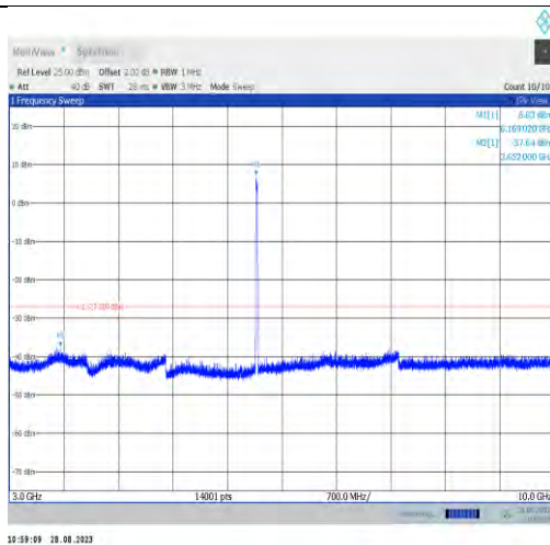
11ax20MIMO-Ant9-6175-3000~10000
