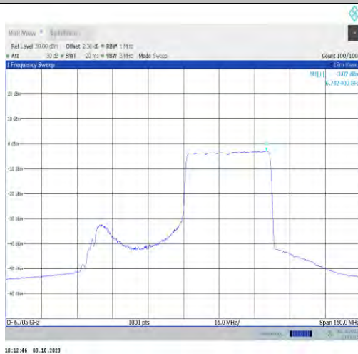
11ax80MIMO-Ant7-6705-PASS
