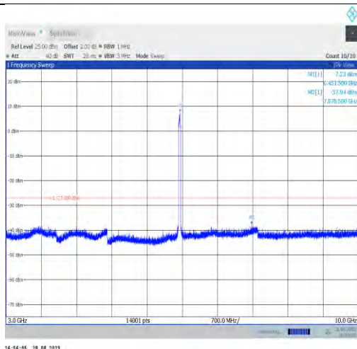
11ax40MIMO-Ant9-6445-3000~10000
