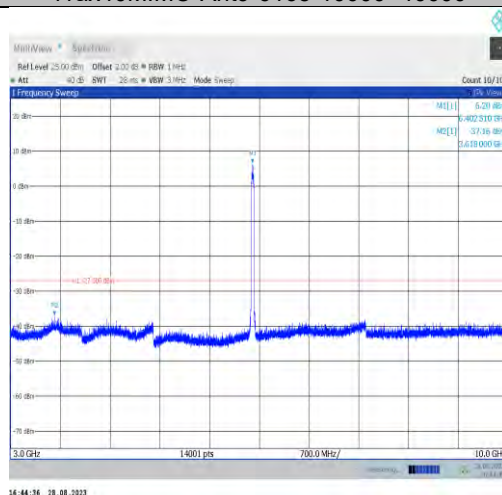
11ax40MIMO-Ant7-6405-3000~10000
