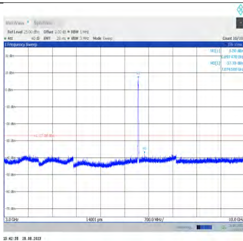
11ax20MIMO-Ant9-6895-3000~10000
