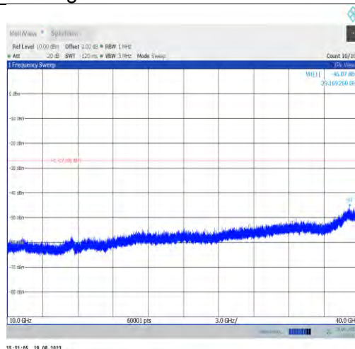
11ax20MIMO-Ant9-6855-10000~40000
