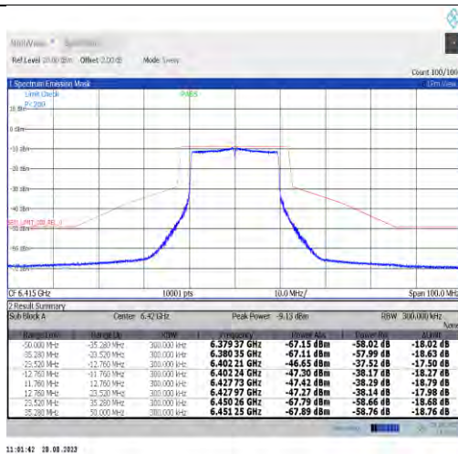
NTNV-11ax20MIMO-Ant7-6415-PASS
