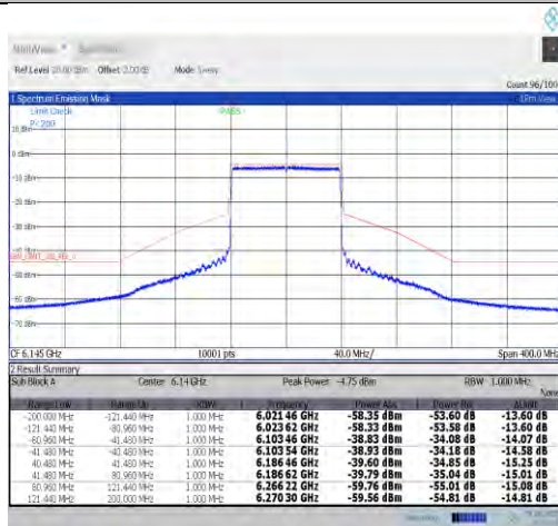
NTNV-11ax80MIMO-Ant7-6145-PASS
