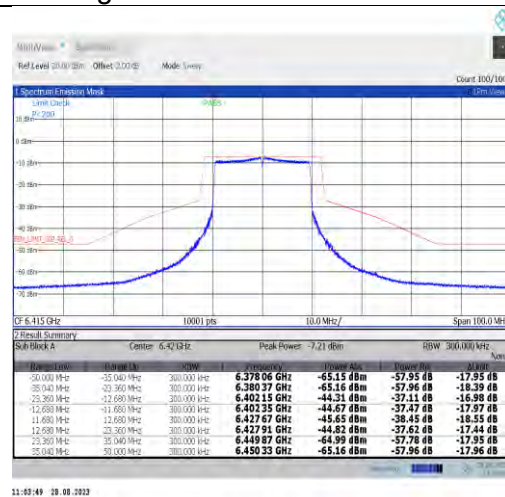
NTNV-11ax20MIMO-Ant9-6415-PASS
