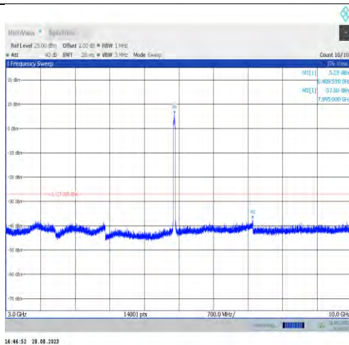
11ax40MIMO-Ant9-6405-3000~10000
