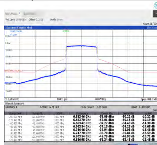
NTNV-11ax80MIMO-Ant9-6705-PASS
