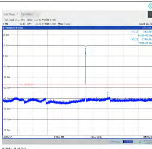
11ax20MIMO-Ant9-6855-3000~10000
