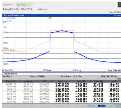
NTNV-11ax40MIMO-Ant7-6845-PASS
