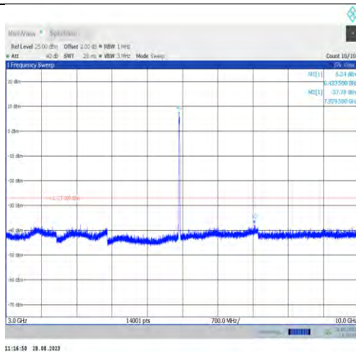
11ax20MIMO-Ant9-6435-3000~10000
