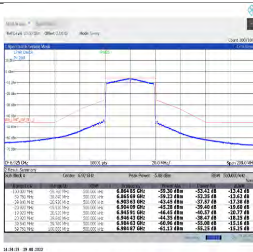
NTNV-11ax40MIMO-Ant7-6925-PASS
