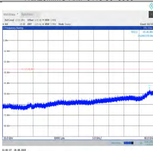
11ax20MIMO-Ant7-6415-10000~40000
