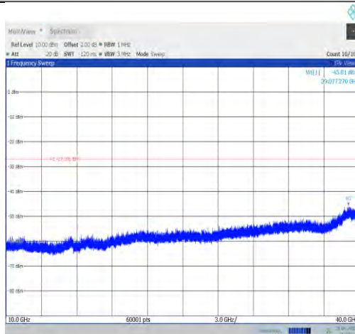
11ax40MIMO-Ant7-6165-10000~40000
