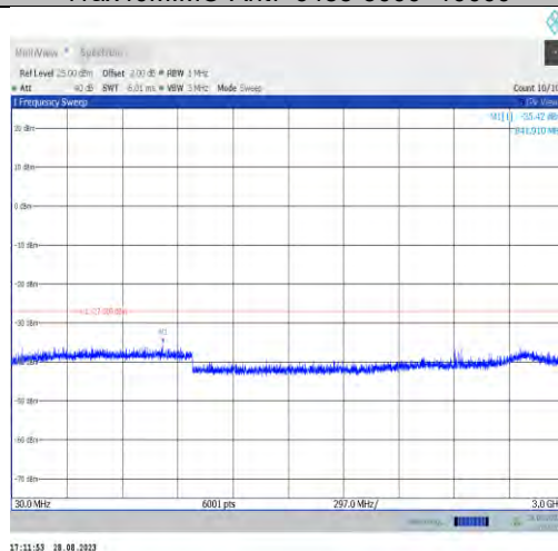
11ax40MIMO-Ant9-6485-30~3000
