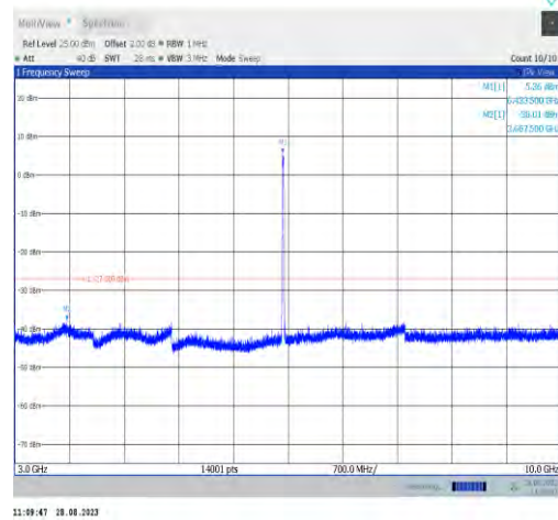
11ax20MIMO-Ant7-6435-3000~10000
