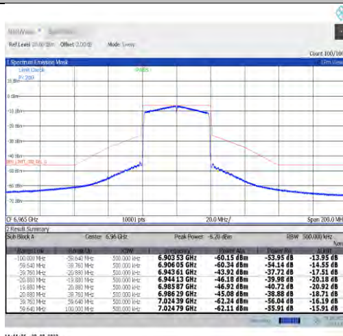
NTNV-11ax40MIMO-Ant7-6965-PASS
