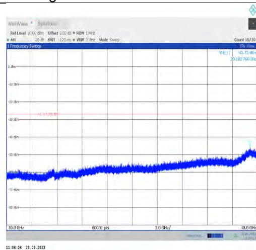
11ax20MIMO-Ant9-6415-10000~40000
