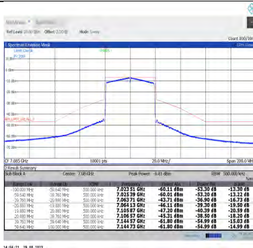
NTNV-11ax40MIMO-Ant7-7085-PASS
