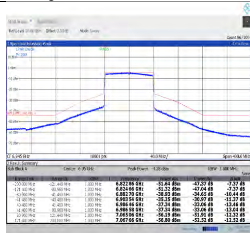
NTVN-11ax80MIMO-Ant9-6945-PASS
