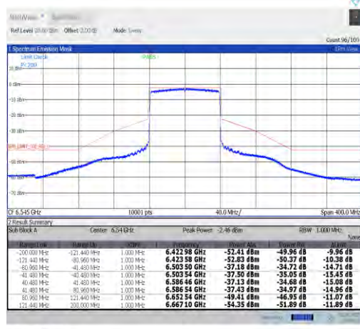
NTNV-11ax80MIMO-Ant9-6545-PASS
