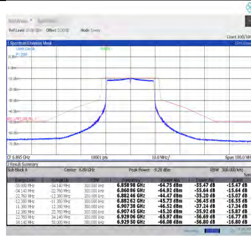
NTNV-11ax20MIMO-Ant9-6895-PASS
