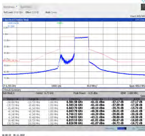
NTNV-11ax80MIMO-Ant7-6705-484Tone-RU66-PASS
