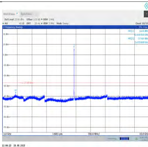
11ax20MIMO-Ant9-6415-3000~10000
