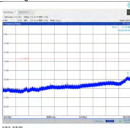
11ax20MIMO-Ant9-6515-10000~40000
