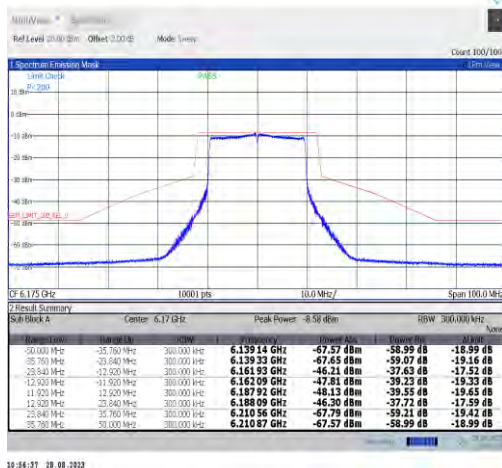
NTVN-11ax20MIMO-Ant7-6175-PASS
