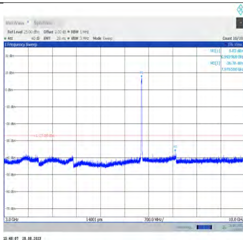
11ax20MIMO-Ant9-6995-3000~10000
