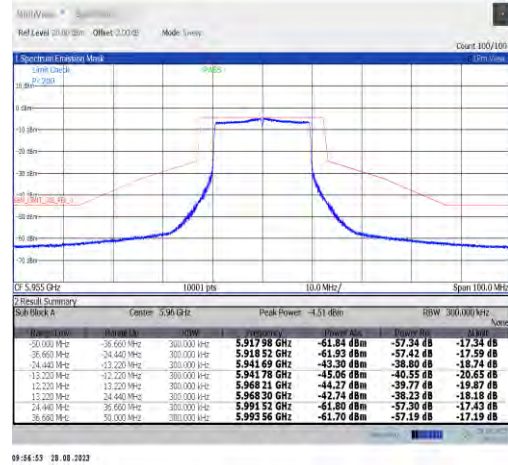
NTVN-11ax20MIMO-Ant9-5955-PASS
