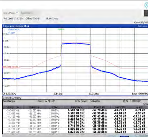
NTNV-11ax80MIMO-Ant7-6705-PASS
