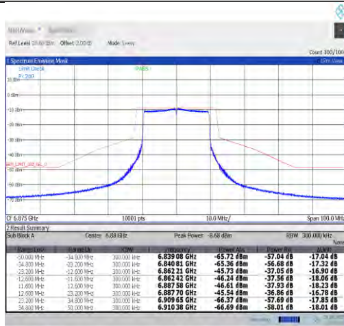
NTNV-11ax20MIMO-Ant7-6875-PASS
