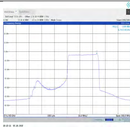
11ax80MIMO-Ant9-6705-PASS
