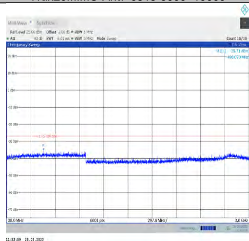
11ax20MIMO-Ant9-6515-30~3000
