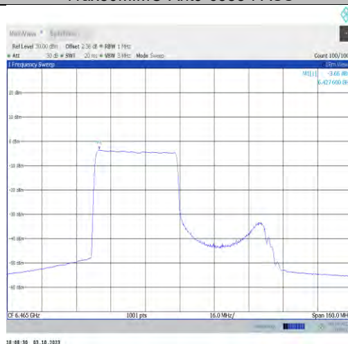
11ax80MIMO-Ant9-6465-PASS
