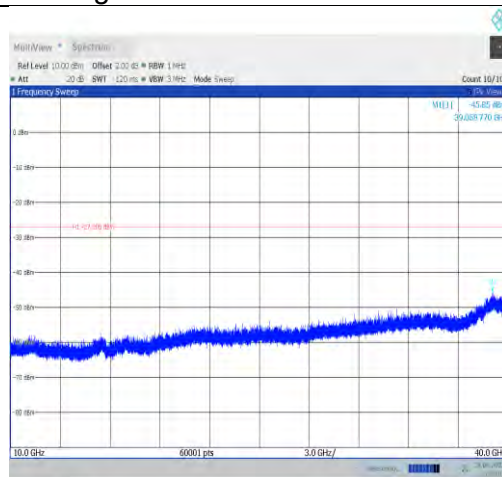
11ax20MIMO-Ant9-6695-10000~40000
