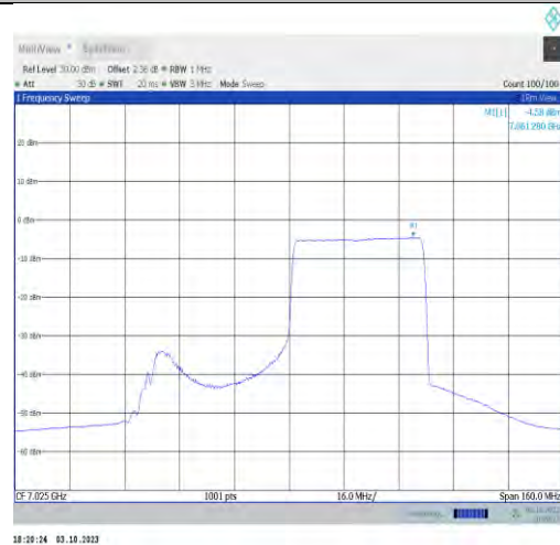
11ax80MIMO-Ant9-7025-PASS
