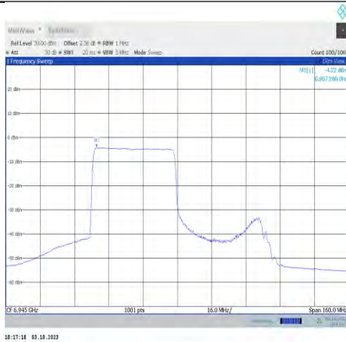
11ax80MIMO-Ant7-6945-PASS
