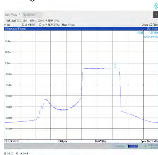
11ax80MIMO-Ant9-6865-PASS
