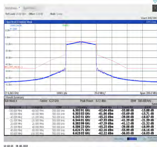
NTNV-11ax40MIMO-Ant9-6565-PASS
