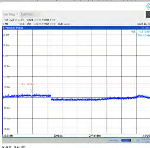
11ax40MIMO-Ant7-6405-30~3000
