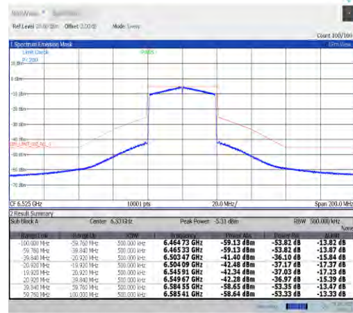
NTNV-11ax40MIMO-Ant9-6525-PASS
