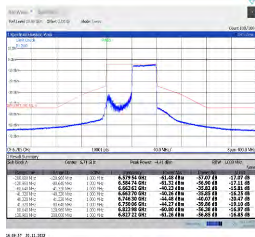
NTNV-11ax80MIMO-Ant9-6705-484Tone-RU66-PASS
