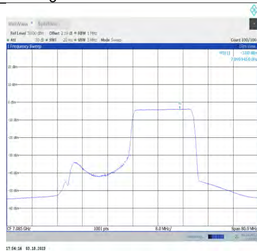
11ax40MIMO-Ant9-7085-PASS
