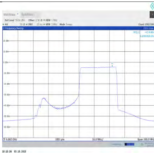
11ax80MIMO-Ant7-6865-PASS
