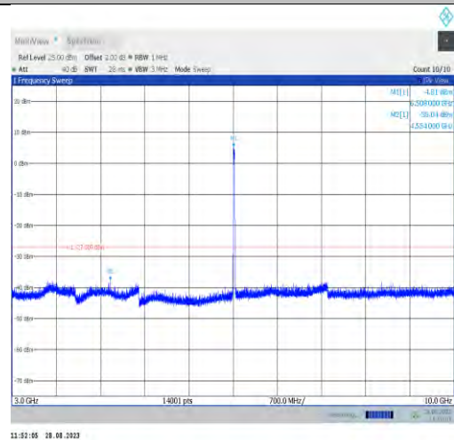
11ax20MIMO-Ant7-6515-3000~10000
