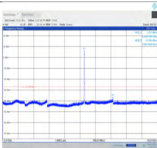
11ax20MIMO-Ant9-6695-3000~10000
