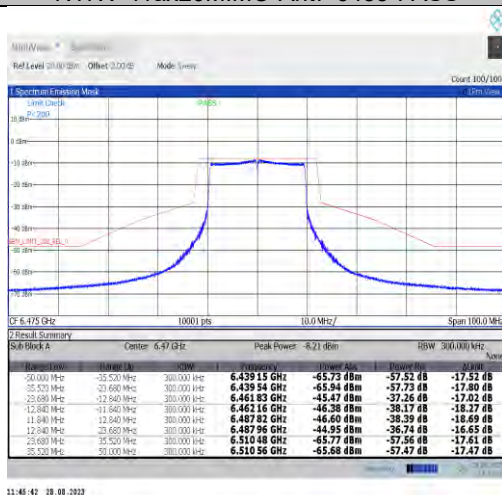
NTNV-11ax20MIMO-Ant7-6475-PASS
