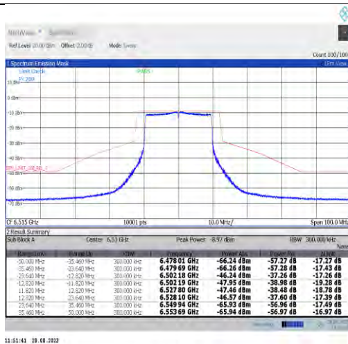
NTNV-11ax20MIMO-Ant7-6515-PASS
