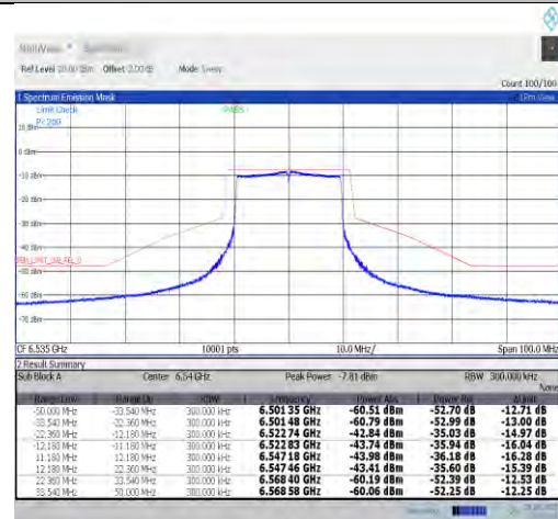
NTNV-11ax20MIMO-Ant9-6535-PASS
