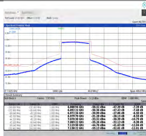
NTVN-11ax80MIMO-Ant9-7025-PASS
