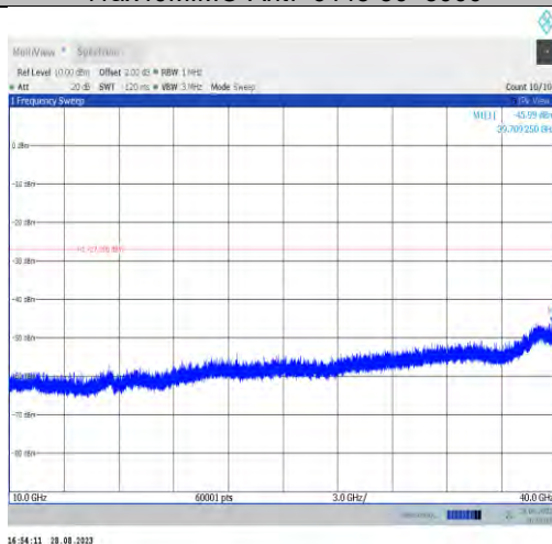
11ax40MIMO-Ant7-6445-10000~40000
