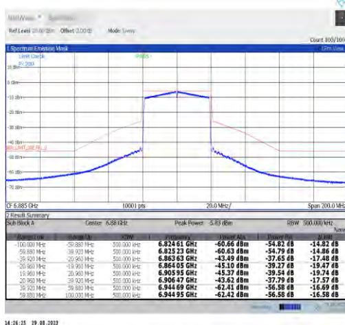
NTNV-11ax40MIMO-Ant7-6885-PASS
