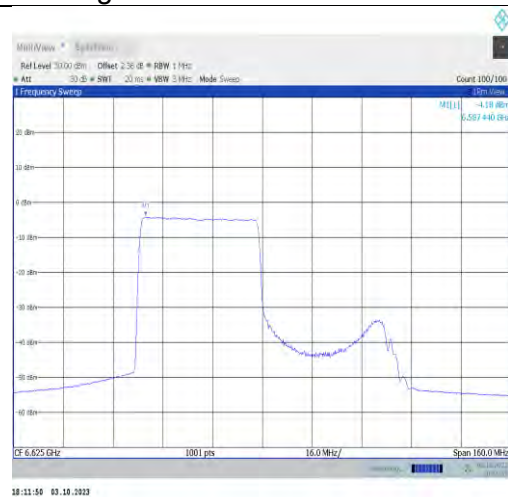
11ax80MIMO-Ant9-6625-PASS
