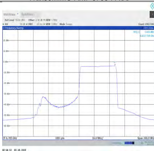
11ax80MIMO-Ant7-6785-PASS
