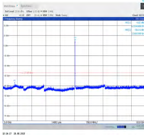
11ax20MIMO-Ant7-6535-3000~10000
