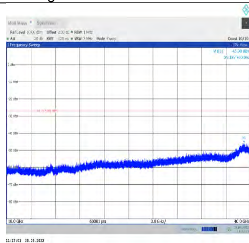
11ax20MIMO-Ant9-6435-10000~40000
