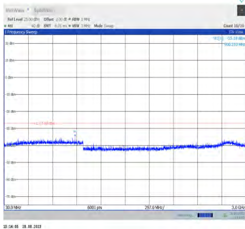
11ax20MIMO-Ant7-6535-30~3000
