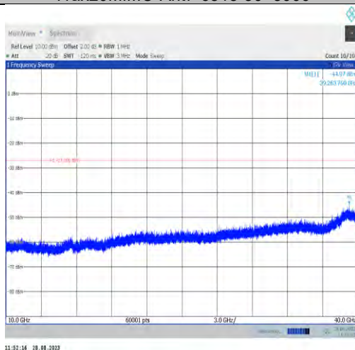
11ax20MIMO-Ant7-6515-10000~40000
