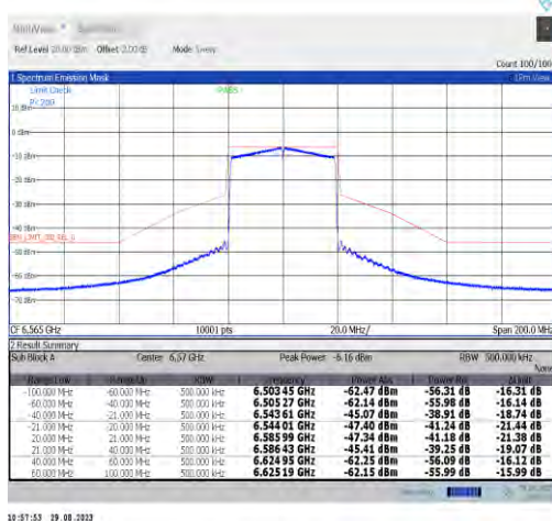
NTNV-11ax40MIMO-Ant7-6565-PASS
