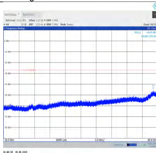
11ax20MIMO-Ant9-6995-10000~40000
