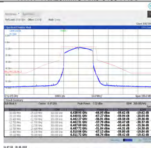
NTNV-11ax20MIMO-Ant9-6475-PASS
