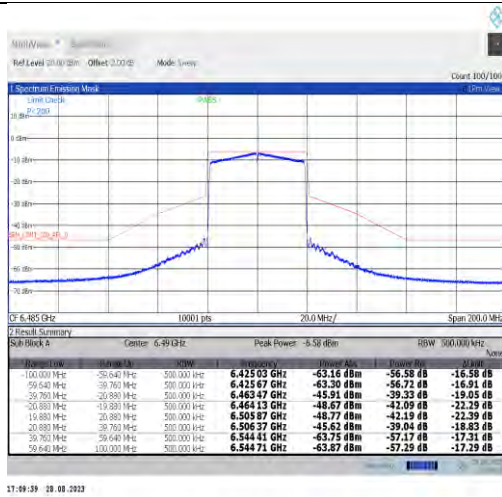
NTNV-11ax40MIMO-Ant7-6485-PASS
