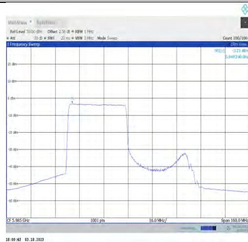
11ax80MIMO-Ant9-5985-PASS
