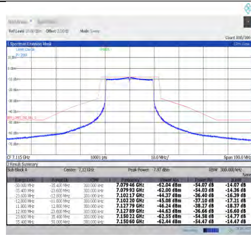
NTVN-11ax20MIMO-Ant9-7115-PASS
