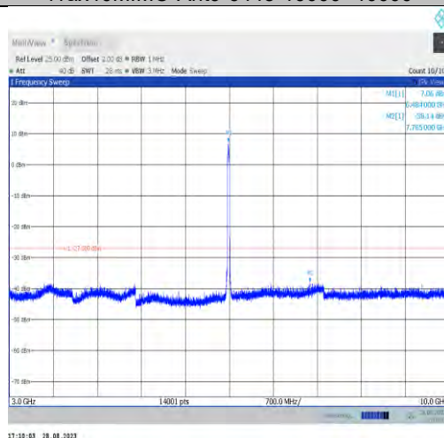
11ax40MIMO-Ant7-6485-3000~10000
