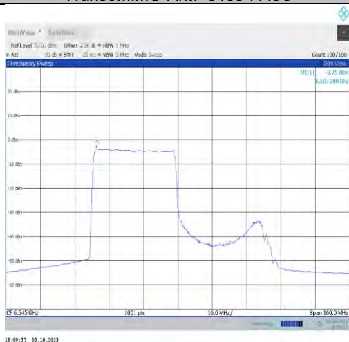
11ax80MIMO-Ant7-6545-PASS
