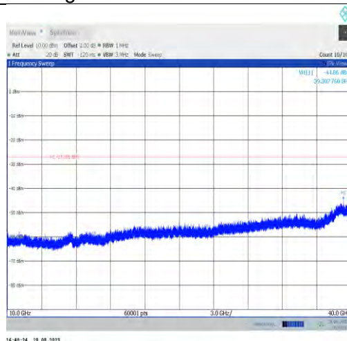
11ax40MIMO-Ant9-6165-10000~40000
