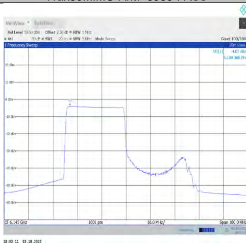
11ax80MIMO-Ant7-6145-PASS
