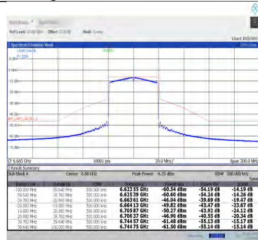
NTNV-11ax40MIMO-Ant9-6685-PASS
