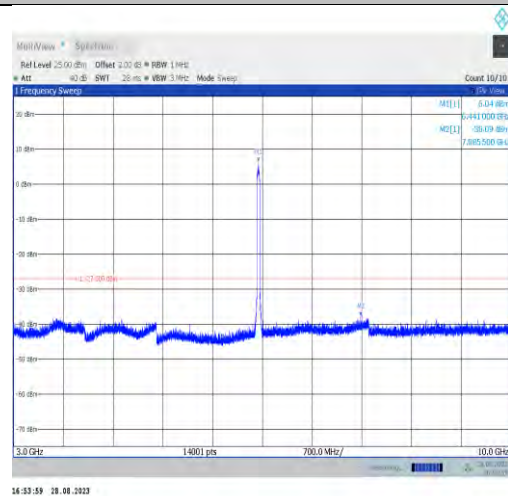
11ax40MIMO-Ant7-6445-3000~10000
