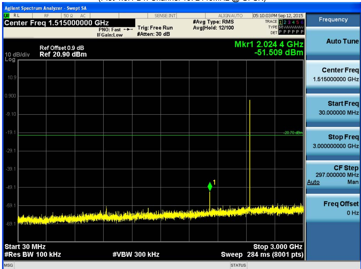
(Plot 4.6.1 B2: Channel 19: 2440MHz @ GFSK)
