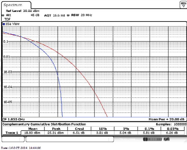
Band2-10MHz-16QAM-18650-25RB#0
