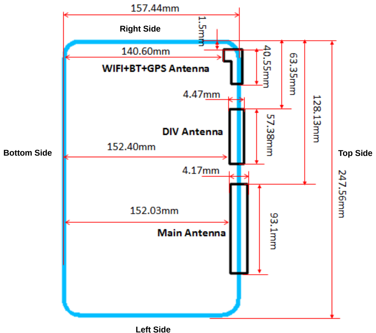
Picture 16: Antenna Locations (Back View)
