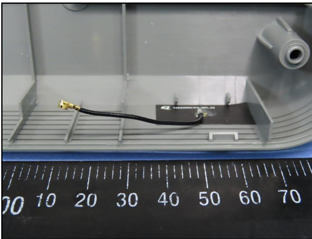
WLAN Antenna 1 (Model: Y4AXO00A1FA)
