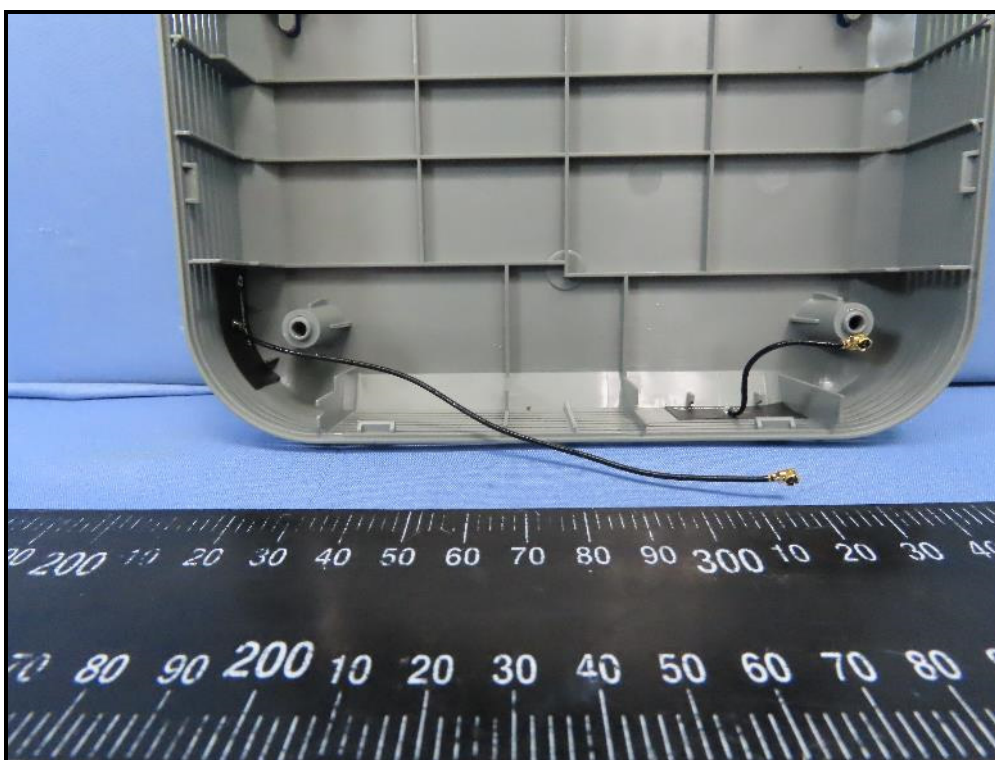
WLAN Antenna 2 (Model: Y4AXO00A1EA)
