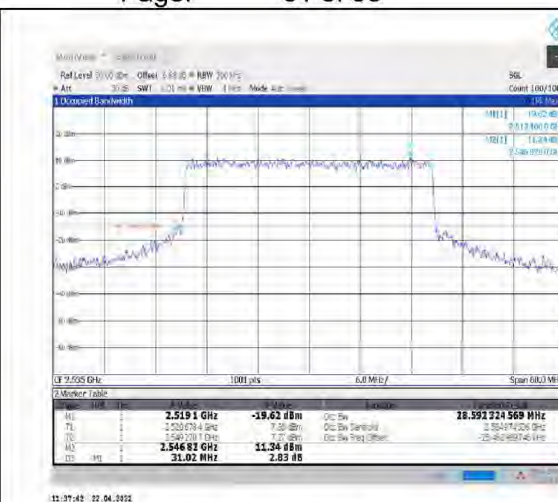
1-N7--15-30-M-6-CP-QPSK-Outer_Full-160@0- Ant1-28.595-31.020≤30-PASS
