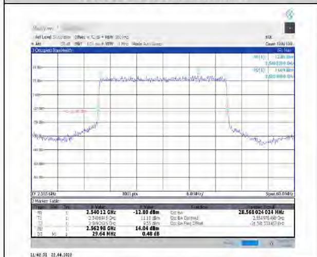
1-N7--15-30-H-2-DFT-PI2BPSK-Outer_Full-160@0- Ant1-28.568-29.640-≤30-PASS
