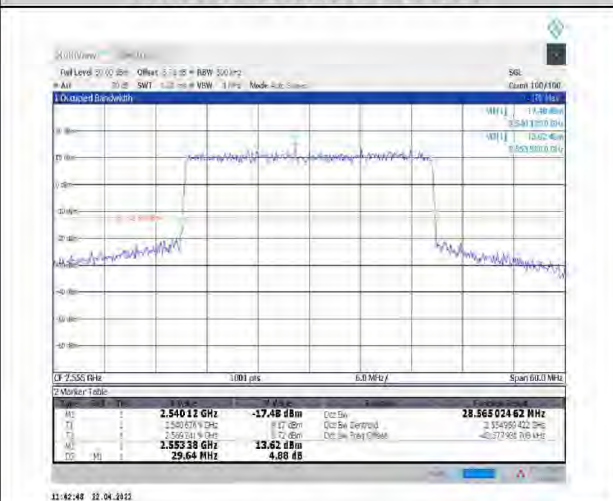
1-N7--15-30-H-3-DFT-16QAM-Outer_Full-160@0- Ant1-28.565-29.640-≤30-PASS
