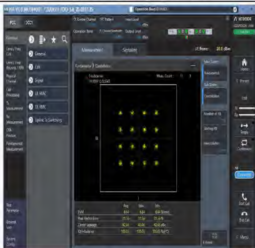
1-N7-PC3-15-40-M-7-CP-16QAM-Outer_Full-216@0-Ant1-see graph-PASS
