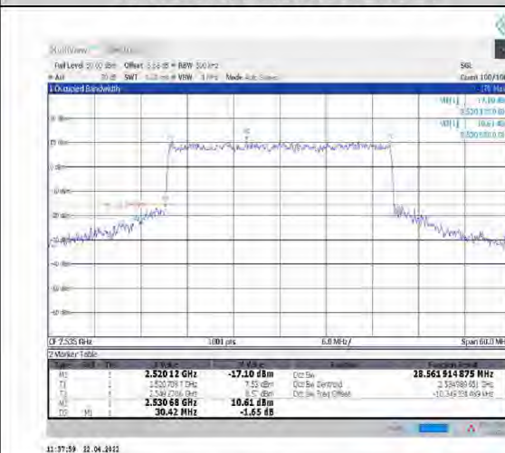
1-N7--15-30-M-8-CP-64QAM-Outer_Full-160@0- Ant1-28.563-30.420≤30-PASS
