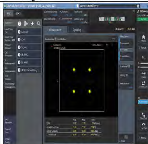
1-N7-PC3-15-40-M-6-CP-QPSK-Outer_Full-216@0-Ant1-see graph-PASS
