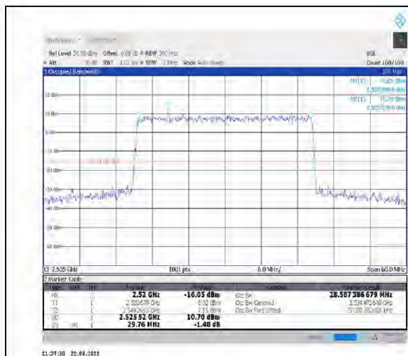
1-N7--15-30-M-5-DFT-256QAM-Outer_Full-160@0- Ant1-28.587-29.760-≤30-PASS
