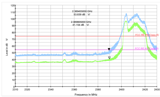
26-Tones 802.11ax HE20-Channel 1 Peak+ Average
