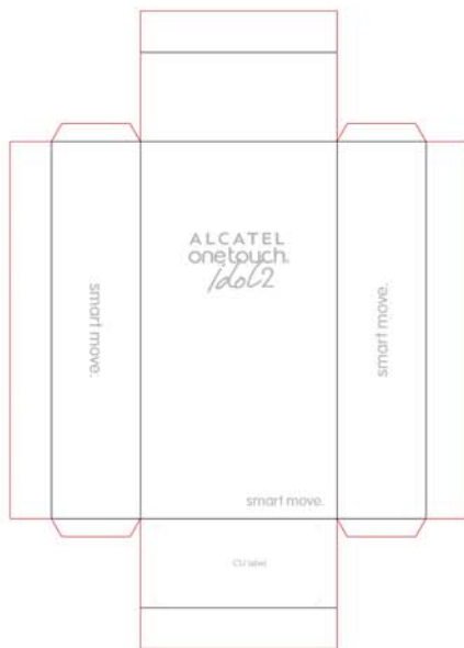
top side 182*95*43mm
