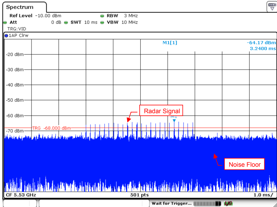
Radar Signal 2
