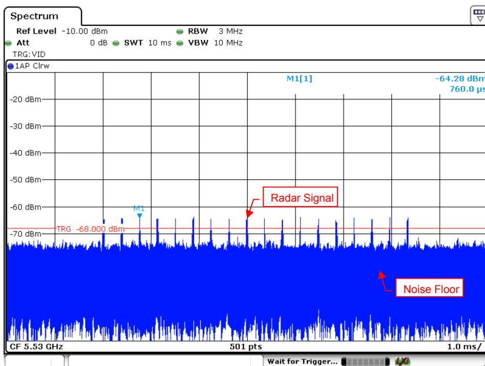
Radar Signal 2
