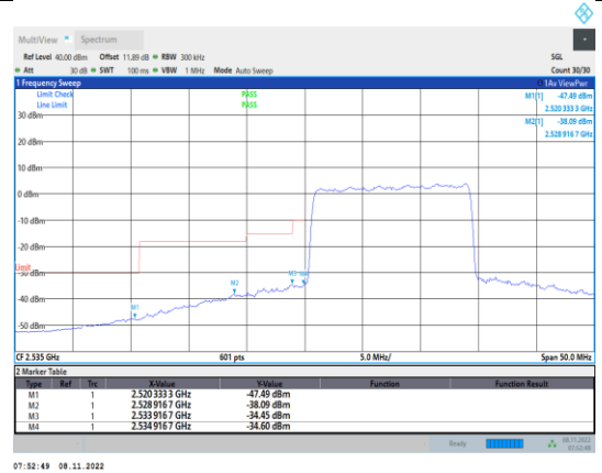
Band41-15MHz-16QAM-40115-75RB#0
