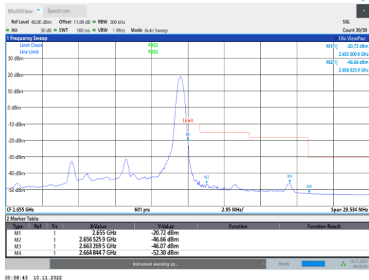
Band41-10MHz-16QAM-41190-1RB#49
