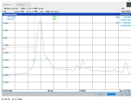
Band26-15MHz-16QAM-26765-1RB#0
