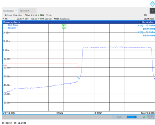
Band26-5MHz-QPSK-26715-25RB#0
