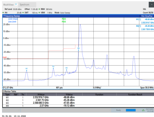
Band38-10MHz-QPSK-37800-1RB#0
