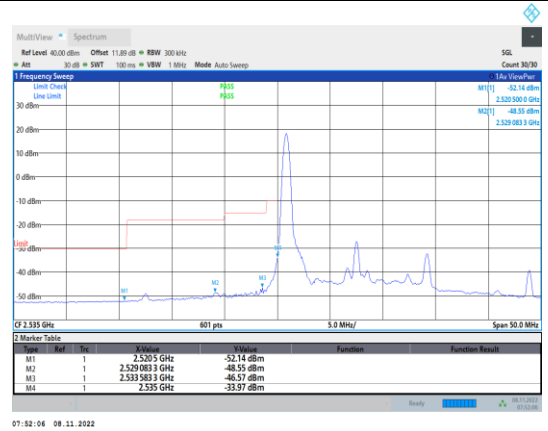
Band41-15MHz-16QAM-40115-1RB#0
