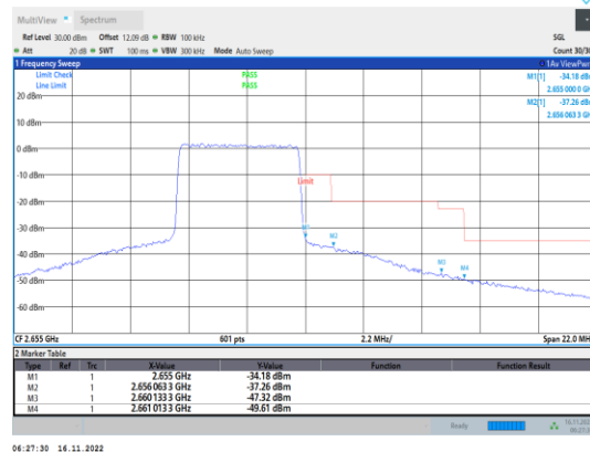
Band41-5MHz-64QAM-41215-25RB#0
