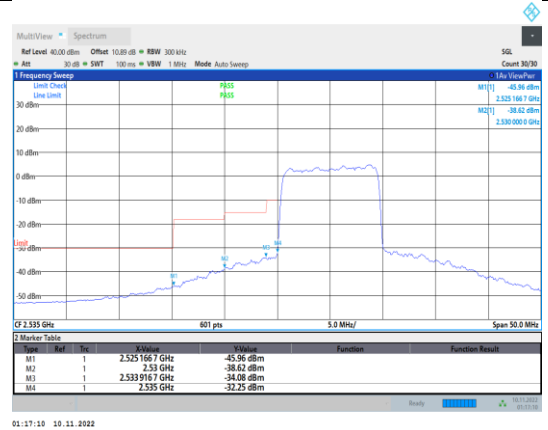
Band41-10MHz-16QAM-40090-50RB#0
