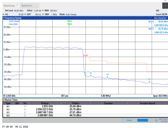
Band41-15MHz-16QAM-41165-75RB#0
