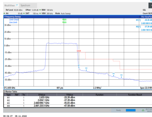
Band41-5MHz-QPSK-41215-25RB#0
