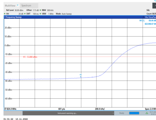
Band26-15MHz-16QAM-26865-75RB#0
