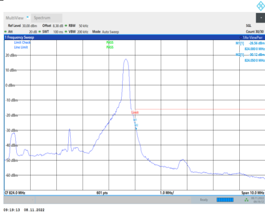
Band26-5MHz-QPSK-26765-1RB#24
