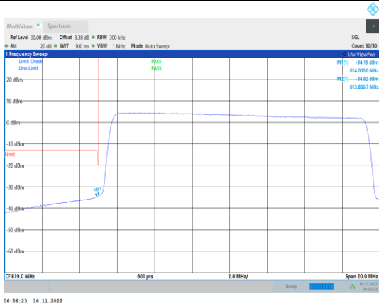
Band26-15MHz-64QAM-26765-75RB#0
