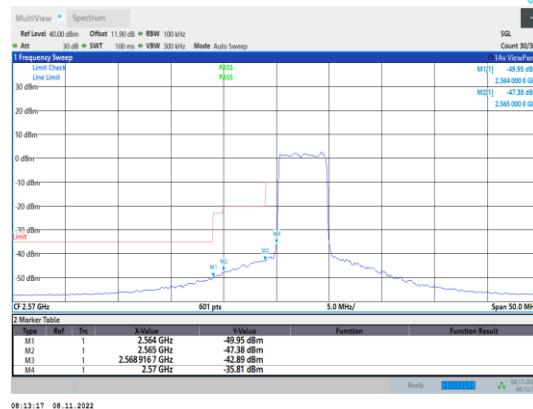
Band38-5MHz-16QAM-37775-25RB#0
