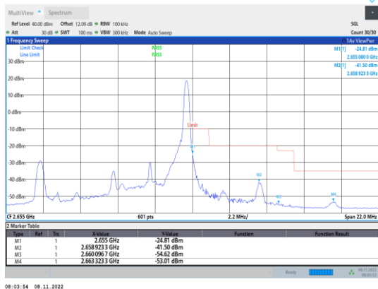
Band41-5MHz-QPSK-41215-1RB#24
