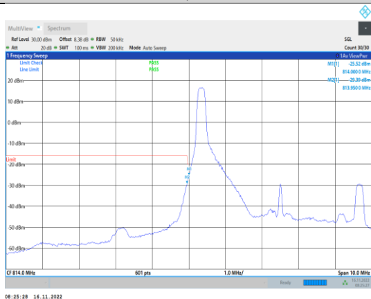
Band26-5MHz-64QAM-26715-1RB#0
