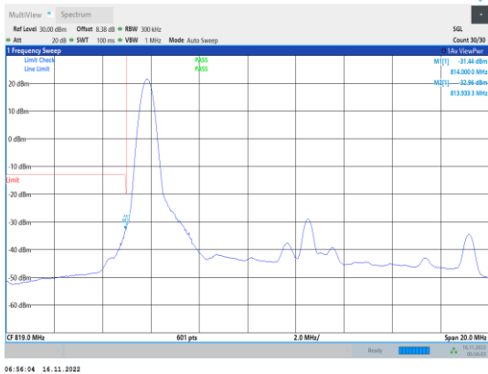
Band26-15MHz-64QAM-26765-1RB#0
