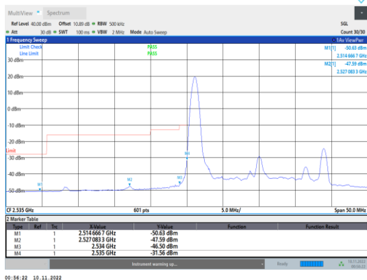
Band41-20MHz-QPSK-40140-1RB#0
