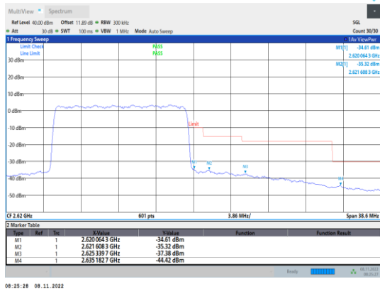
Band38-15MHz-16QAM-38175-75RB#0
