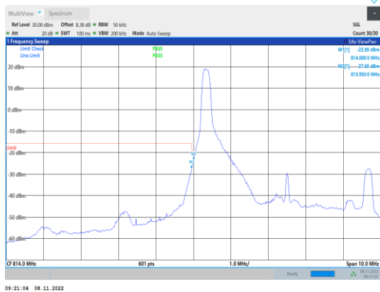
Band26-5MHz-QPSK-26715-1RB#0
