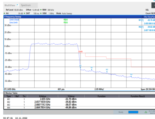
Band41-10MHz-64QAM-41190-50RB#0
