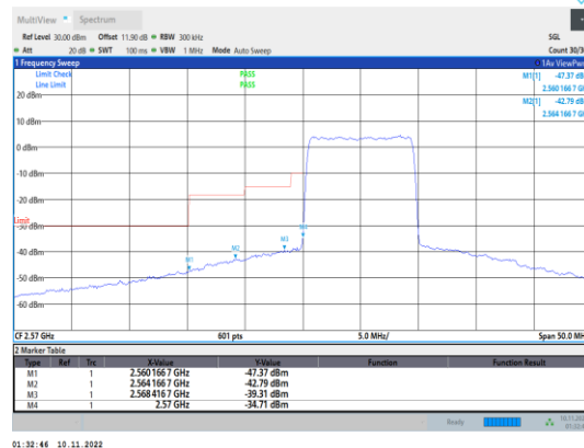
Band38-10MHz-16QAM-37800-50RB#0
