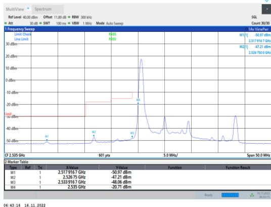
Band41-10MHz-64QAM-40090-1RB#0
