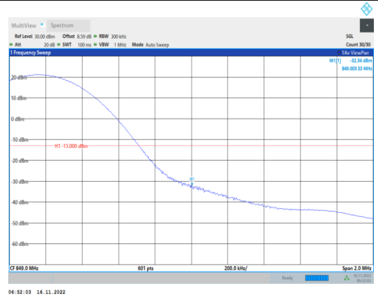
Band26-15MHz-64QAM-26965-1RB#74
