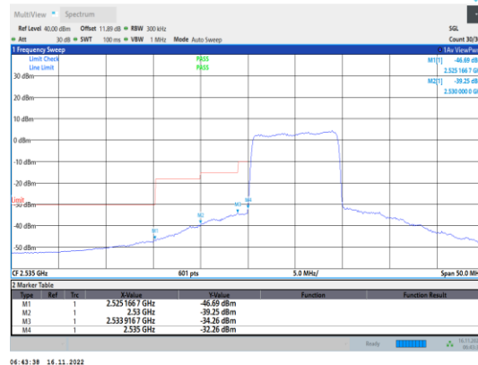
Band41-10MHz-64QAM-40090-50RB#0
