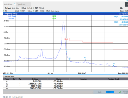
Band41-15MHz-64QAM-41165-1RB#74
