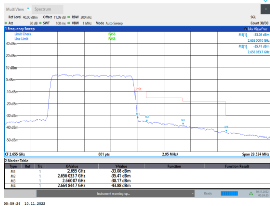
Band41-10MHz-16QAM-41190-50RB#0
