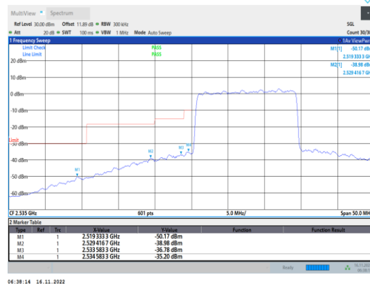
Band41-15MHz-64QAM-40115-75RB#0
