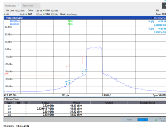
Band41-5MHz-16QAM-40065-25RB#0
