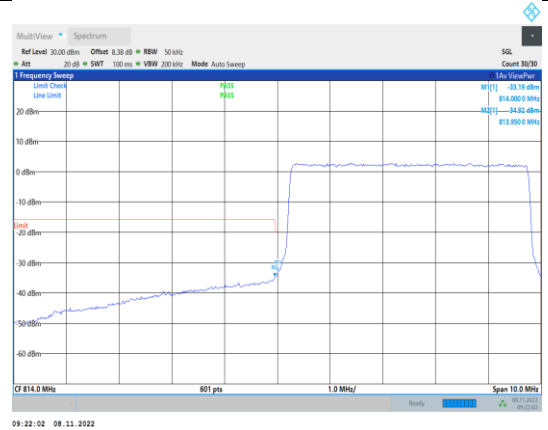
Band26-5MHz-16QAM-26715-25RB#0
