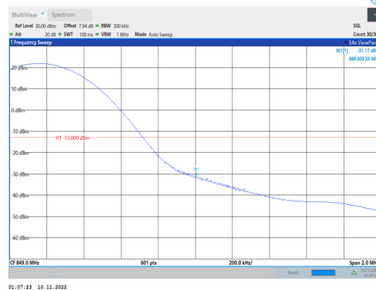
Band26-15MHz-16QAM-26965-1RB#74
