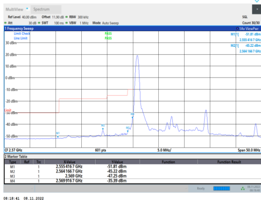
Band38-15MHz-QPSK-37825-1RB#0
