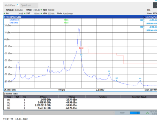
Band41-5MHz-64QAM-41215-1RB#24
