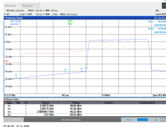
Band38-20MHz-16QAM-38150-100RB#0
