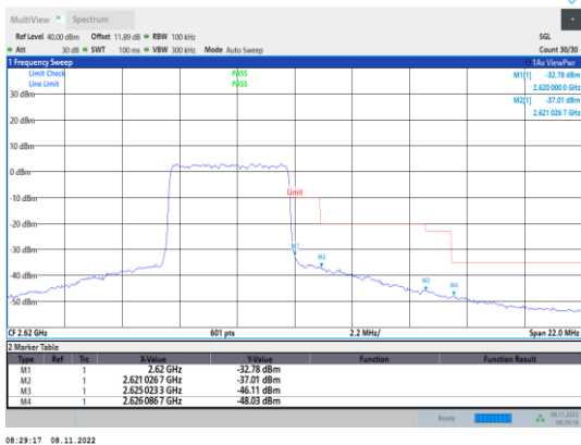
Band38-5MHz-16QAM-38225-25RB#0
