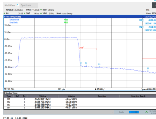
Band38-20MHz-64QAM-38150-100RB#0
