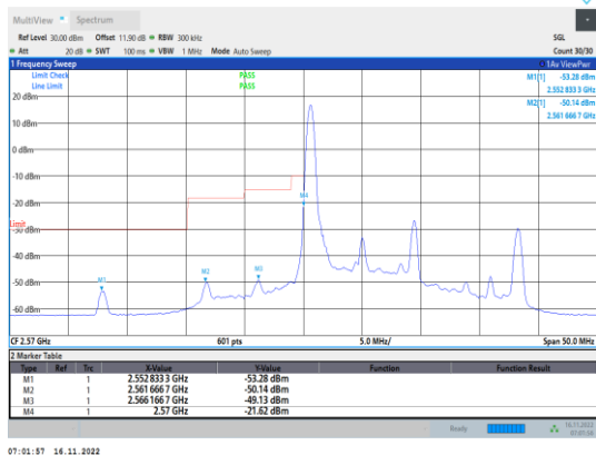
Band38-10MHz-64QAM-37800-1RB#0
