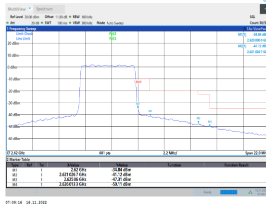
Band38-5MHz-64QAM-38225-25RB#0
