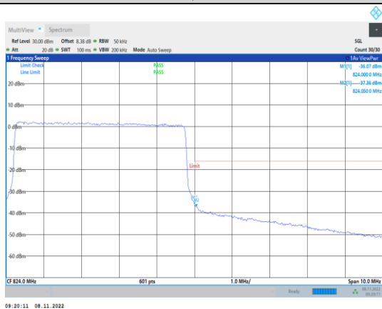
Band26-5MHz-16QAM-26765-25RB#0
