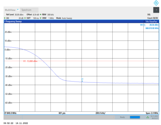
Band26-15MHz-64QAM-26965-75RB#0
