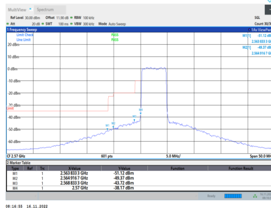
Band38-5MHz-64QAM-37775-25RB#0
