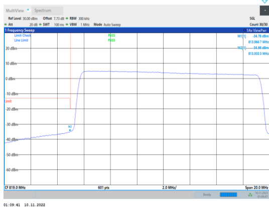
Band26-15MHz-16QAM-26765-75RB#0
