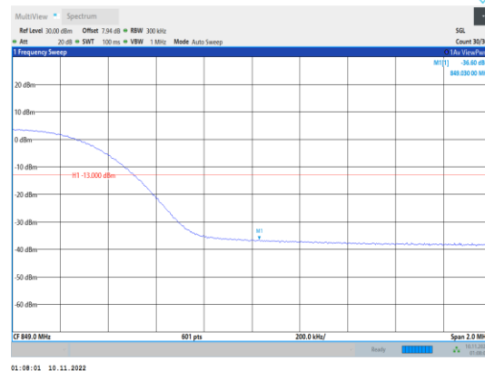
Band26-15MHz-16QAM-26965-75RB#0
