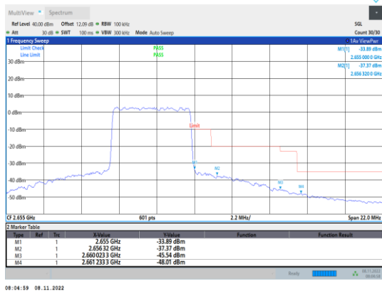
Band41-5MHz-16QAM-41215-25RB#0
