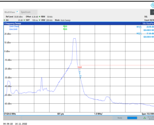
Band26-5MHz-64QAM-26765-1RB#24
