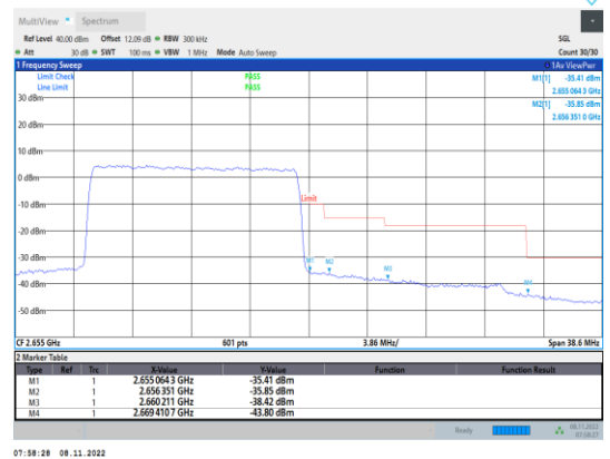
Band41-15MHz-QPSK-41165-75RB#0
