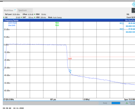
Band26-5MHz-64QAM-26765-25RB#0
