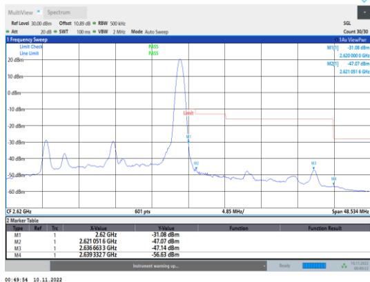
Band38-20MHz-16QAM-37850-1RB#0
