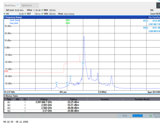
Band38-5MHz-16QAM-37775-1RB#0
