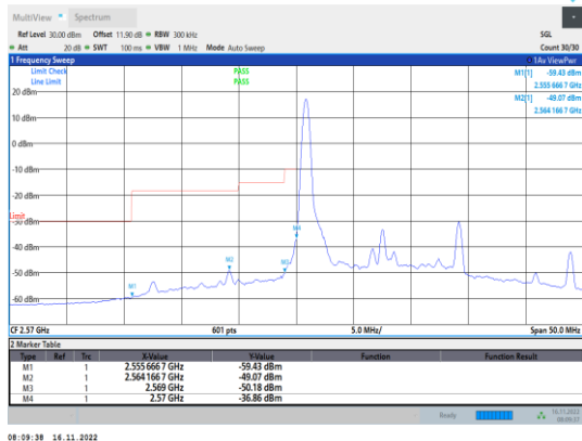
Band38-15MHz-64QAM-37825-1RB#0
