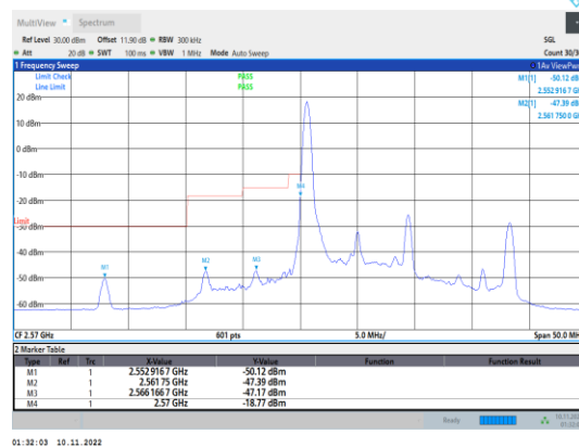
Band38-10MHz-16QAM-37800-1RB#0
