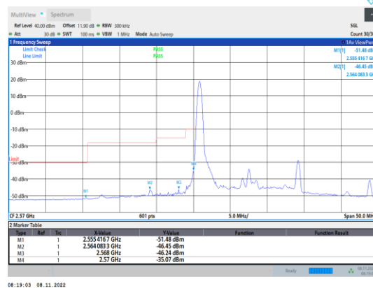
Band38-15MHz-QPSK-38175-1RB#0
