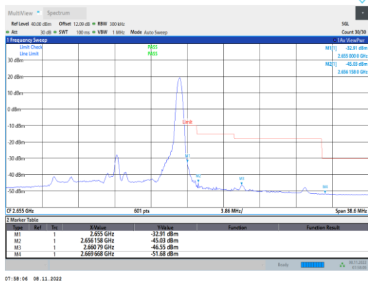
Band41-15MHz-16QAM-41165-1RB#74
