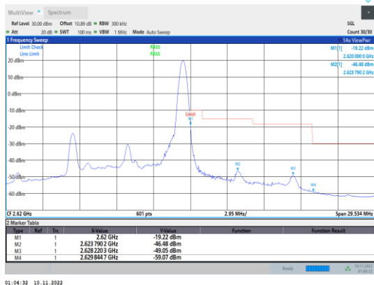
Band38-10MHz-QPSK-38200-1RB#49
