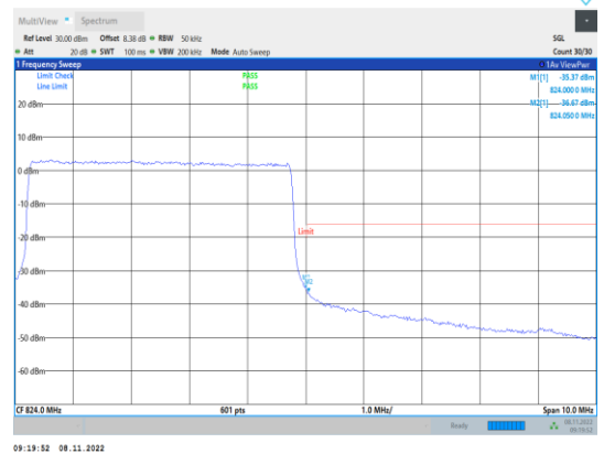
Band26-5MHz-QPSK-26765-25RB#0
