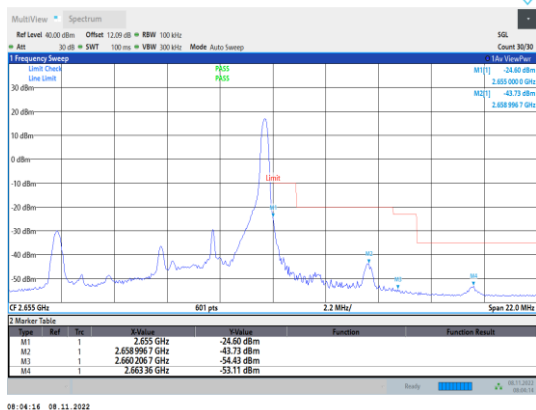
Band41-5MHz-16QAM-41215-1RB#24
