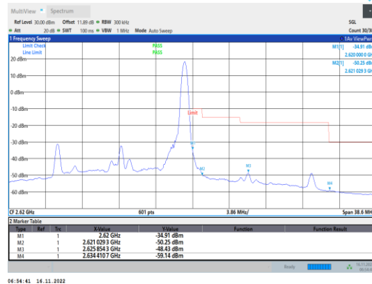
Band38-15MHz-64QAM-38175-1RB#74
