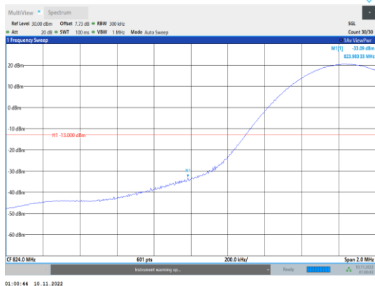
Band26-15MHz-16QAM-26865-1RB#0
