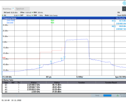
Band41-10MHz-QPSK-40090-50RB#0
