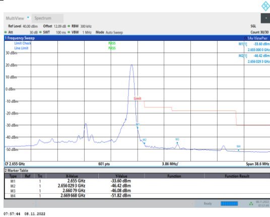
Band41-15MHz-QPSK-41165-1RB#74
