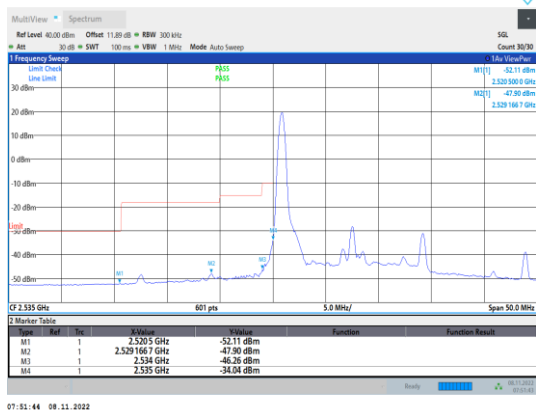
Band41-15MHz-QPSK-40115-1RB#0
