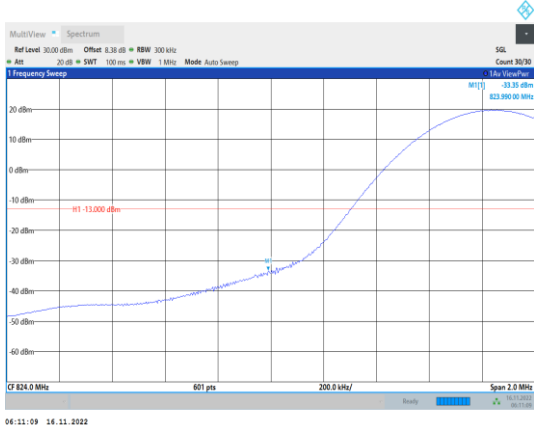
Band26-15MHz-64QAM-26865-1RB#0
