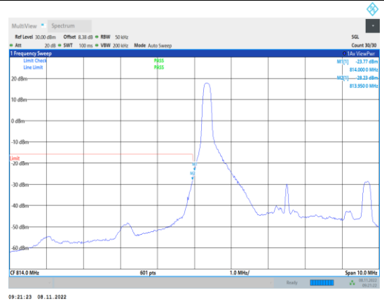
Band26-5MHz-16QAM-26715-1RB#0
