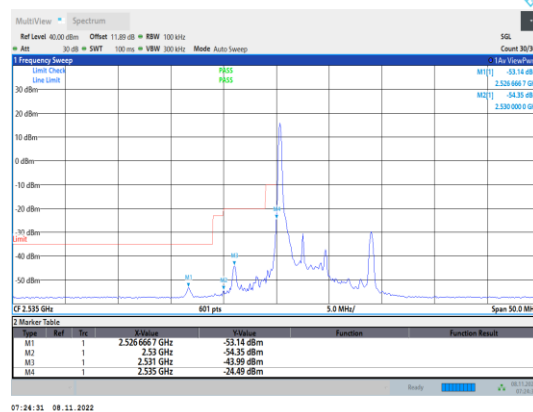
Band41-5MHz-16QAM-40065-1RB#0
