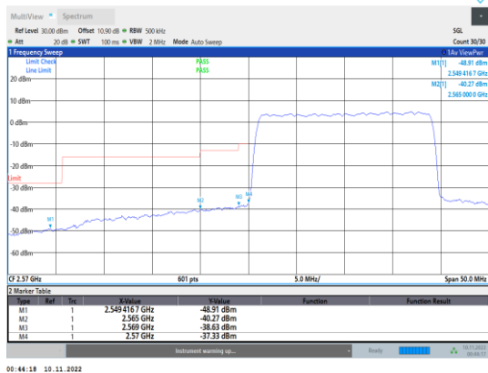
Band38-20MHz-QPSK-37850-100RB#0
