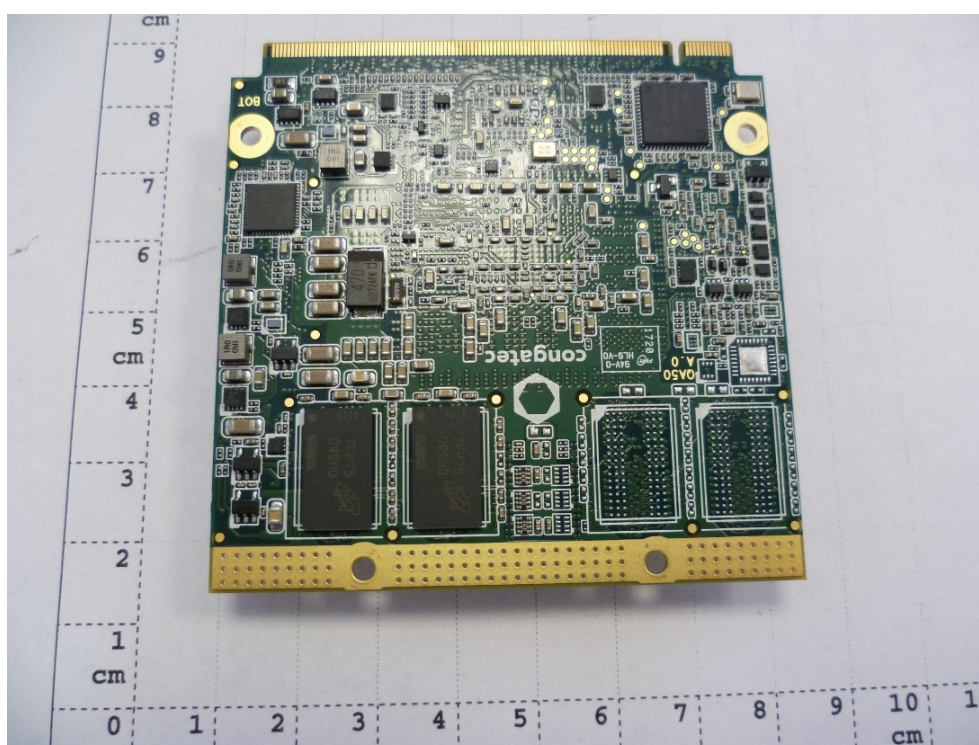
Figure 8: EUT digital pub bottom view
