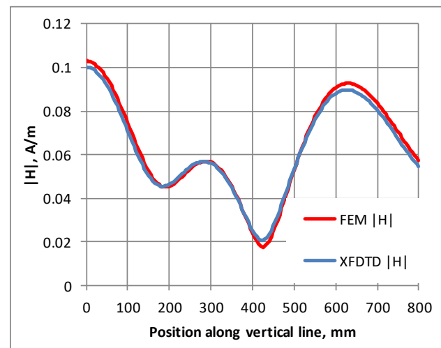
Magnetic field magnitude
