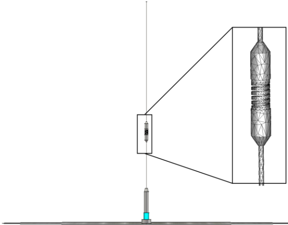
CST MWS (FEM) model of the HAE4011 antenna
