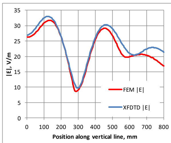
Electric field magnitude
