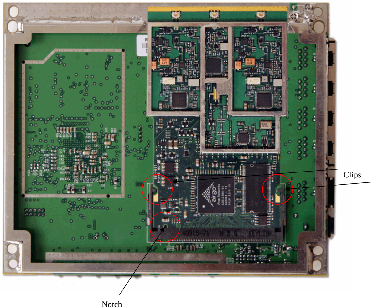
Figure 2 Radio Module Alignment
