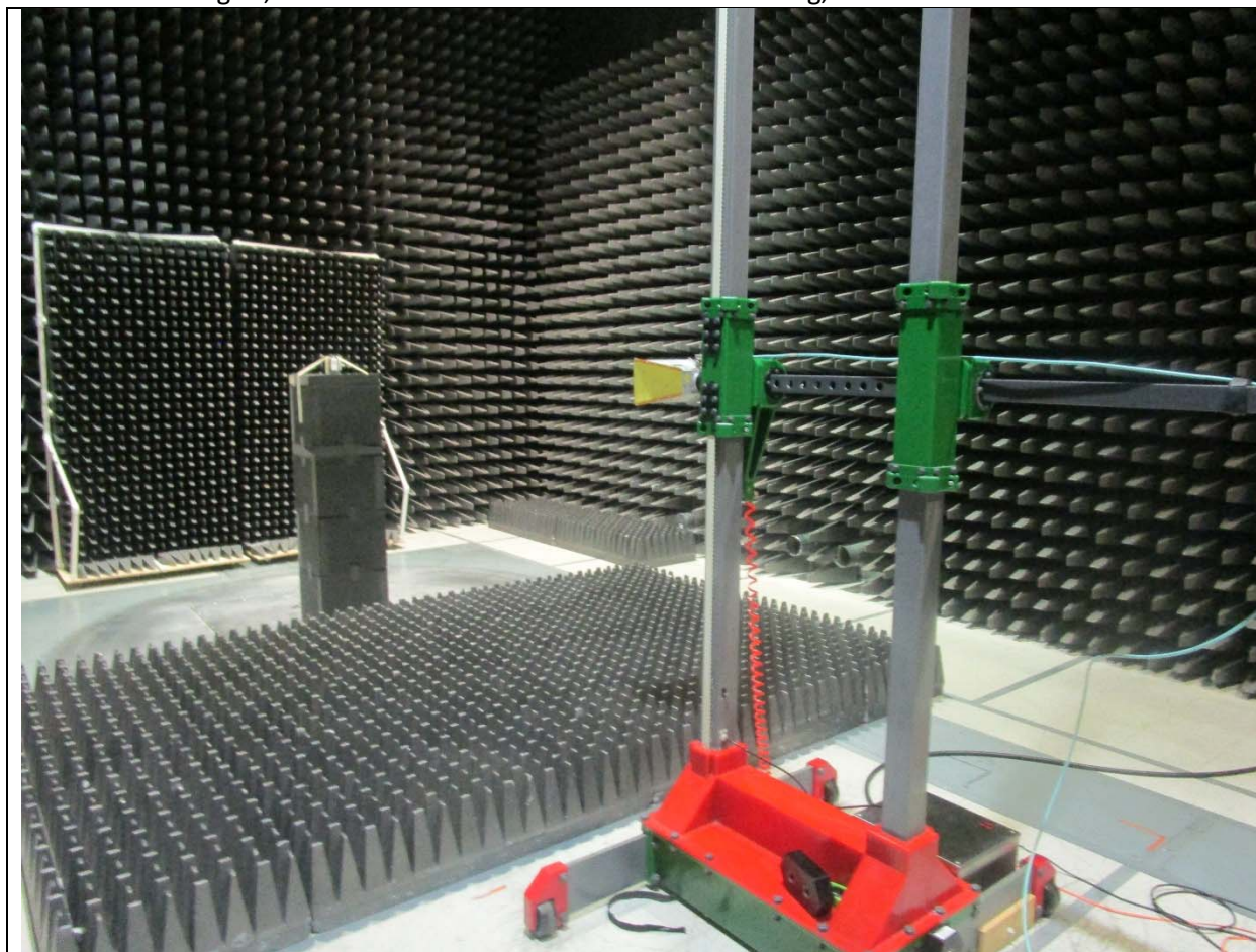
Radiated Emissions
