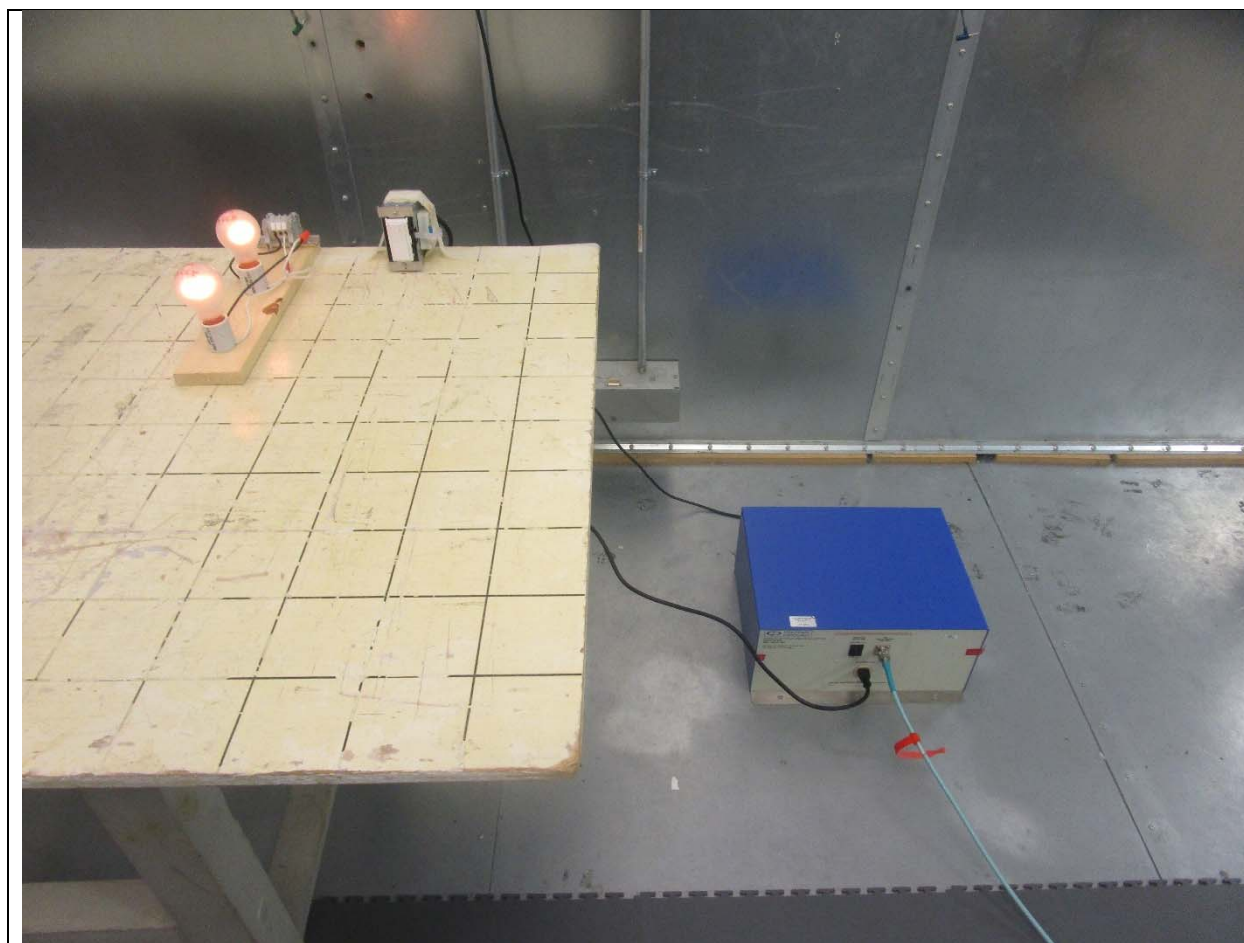
Conducted Emissions
