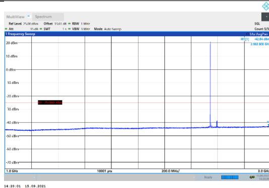
N41-30kHz-100MHz-DFT-QPSK-Mid-Edge_1RB_Left-1000-3000-PASS
