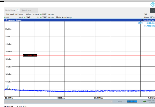
N41-30kHz-40MHz-DFT-QPSK-Low-Edge_1RB_Left-30-1000-PASS
