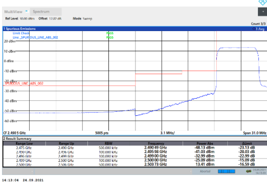
N7-15kHz-5MHz-CP-QPSK-Low-Outer_Full---PASS
