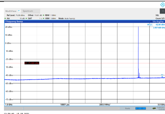
N41-30kHz-30MHz-DFT-QPSK-High-Edge_1RB_Left-1000-3000-PASS
