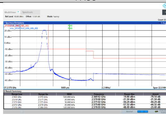
N7-15kHz-20MHz-CP-QPSK-High-Edge_1RB_Right---PASS
