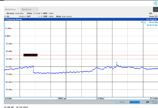
N41-30kHz-30MHz-DFT-QPSK-Mid-Edge_1RB_Left-3000-27000-PASS
