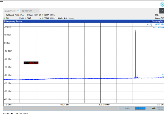
N41-30kHz-60MHz-DFT-QPSK-High-Edge_1RB_Left-1000-3000-PASS
