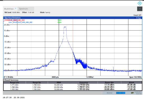
N66-15kHz-20MHz-DFT-QPSK-High-Edge_1RB_Right---PASS
