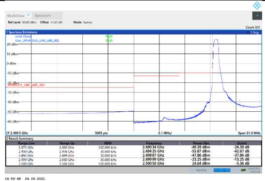
N7-15kHz-15MHz-DFT-QPSK-Low-Edge_1RB_Left--PASS
