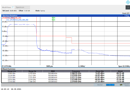
N7-15kHz-5MHz-DFT-QPSK-High-Outer_Full---PASS
