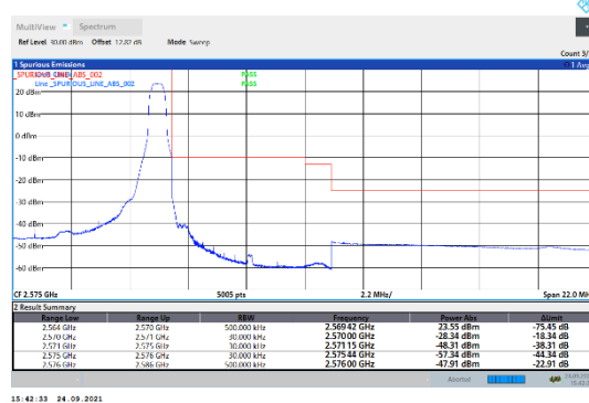
N7-15kHz-20MHz-DFT-QPSK-High-Edge_1RB_Right--PASS
