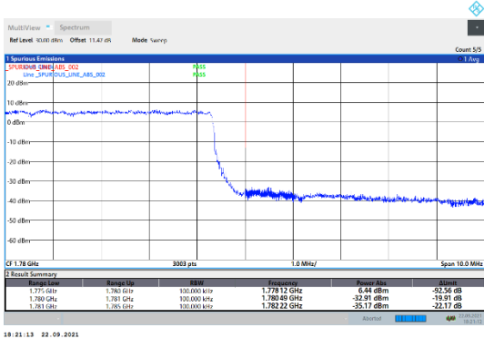
N66-15kHz-10MHz-DFT-QPSK-High-Outer_Full---PASS
