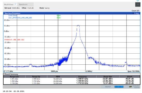
N66-15kHz-15MHz-CP-QPSK-Low-Edge_1RB_Left---PASS
