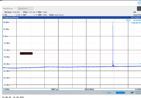
N41-30kHz-30MHz-DFT-QPSK-Mid-Edge_1RB_Left-1000-3000-PASS
