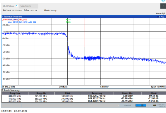
N5-15kHz-15MHz-DFT-QPSK-High-Outer_Full---PASS
