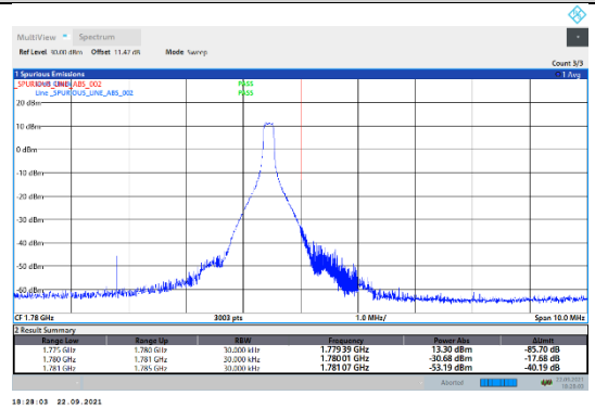
N66-15kHz-20MHz-CP-QPSK-High-Edge_1RB_Right---PASS
