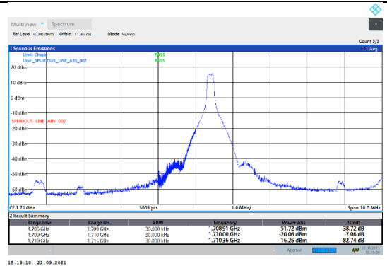
N66-15kHz-10MHz-DFT-QPSK-Low-Edge_1RB_Left---PASS
