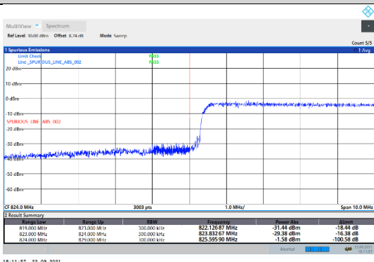
N5-15kHz-20MHz-CP-QPSK-Low-Outer_Full---PASS
