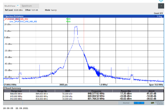
N5-15kHz-15MHz-DFT-QPSK-High-Edge_1RB_Right--PASS
