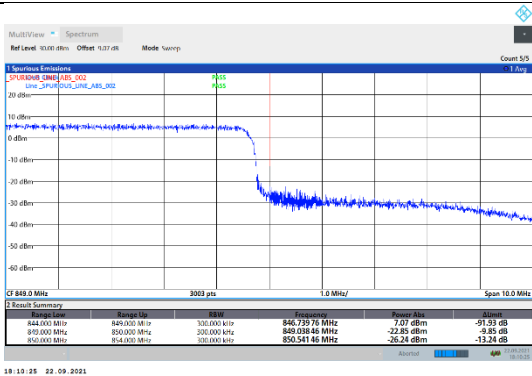
N5-15kHz-15MHz-CP-QPSK-High-Outer_Full---PASS
