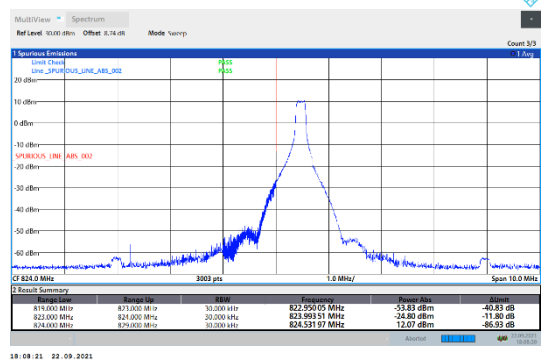
N5-15kHz-15MHz-CP-QPSK-Low-Edge_1RB_Left--PASS
