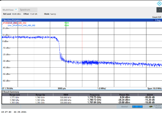
N66-15kHz-20MHz-DFT-QPSK-High-Outer_Full---PASS
