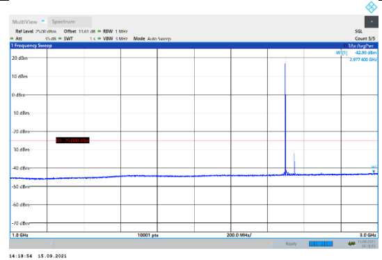
N41-30kHz-100MHz-DFT-QPSK-Low-Edge_1RB_Left-1000-3000-PASS
