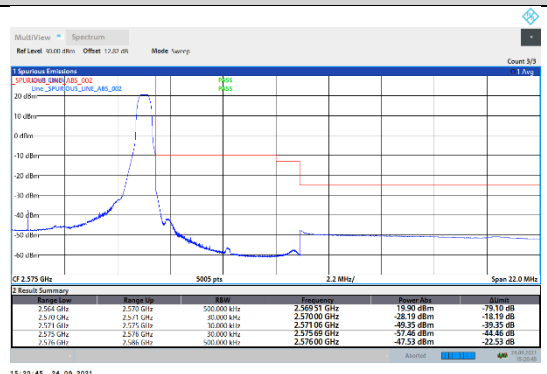
N7-15kHz-15MHz-CP-QPSK-High-Edge_1RB_Right--PASS
