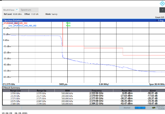
N7-15kHz-15MHz-CP-QPSK-High-Outer_Full---PASS
