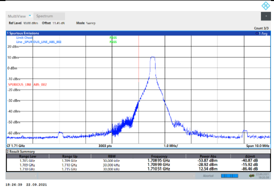
N66-15kHz-20MHz-CP-QPSK-Low-Edge_1RB_Left---PASS
