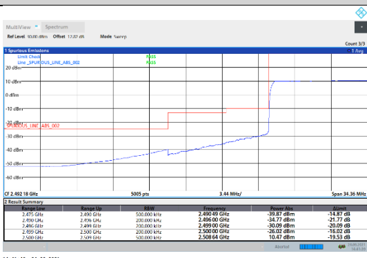
N7-15kHz-10MHz-CP-QPSK-Low-Outer_Full---PASS
