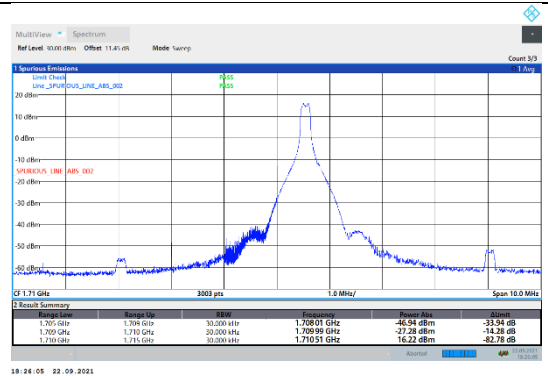
N66-15kHz-20MHz-DFT-QPSK-Low-Edge_1RB_Left---PASS
