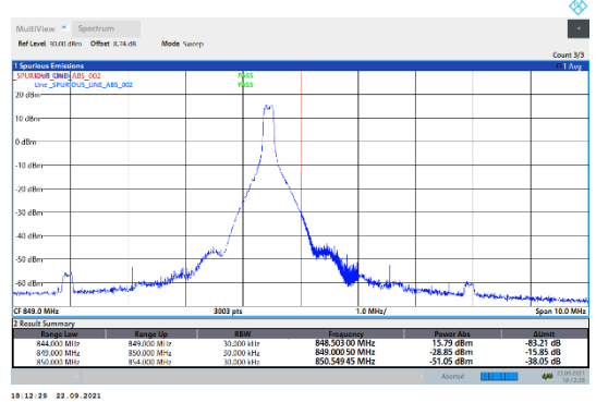
N5-15kHz-20MHz-DFT-QPSK-High-Edge_1RB_Right--PASS
