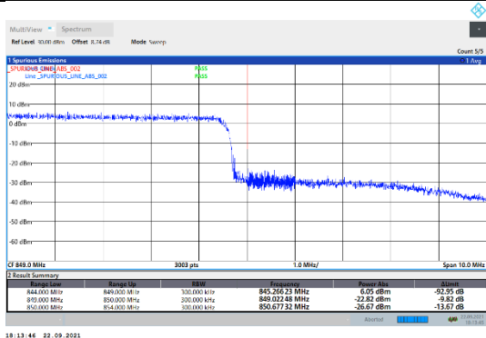
N5-15kHz-20MHz-CP-QPSK-High-Outer_Full---PASS
