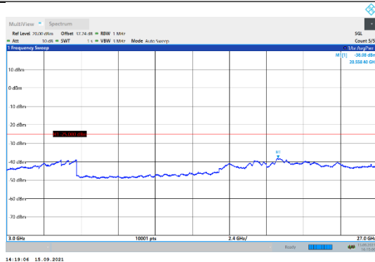
N41-30kHz-100MHz-DFT-QPSK-Low-Edge_1RB_Left-3000-27000-PASS
