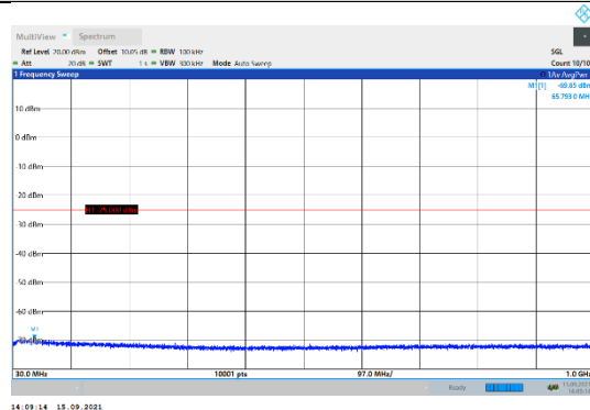
N41-30kHz-60MHz-DFT-QPSK-Mid-Edge_1RB_Left-30-1000-PASS
