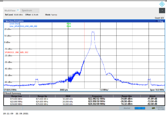
N5-15kHz-20MHz-DFT-QPSK-Low-Edge_1RB_Left--PASS
