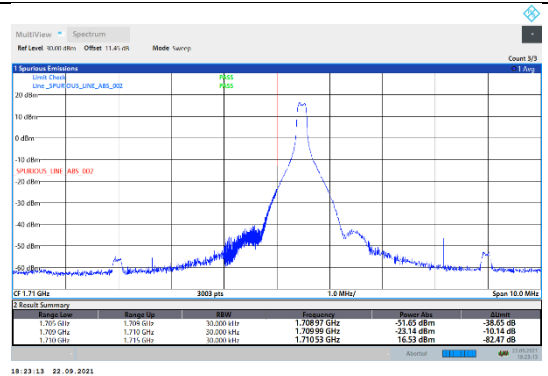
N66-15kHz-15MHz-DFT-QPSK-Low-Edge_1RB_Left---PASS
