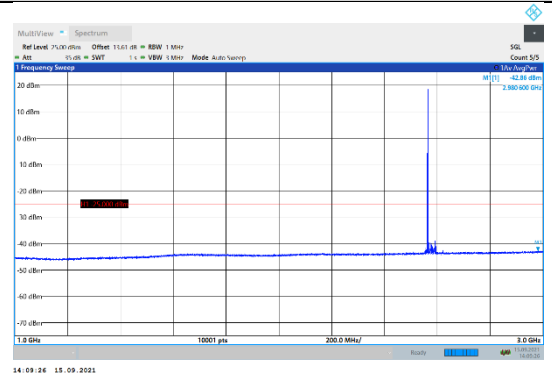
N41-30kHz-60MHz-DFT-QPSK-Mid-Edge_1RB_Left-1000-3000-PASS
