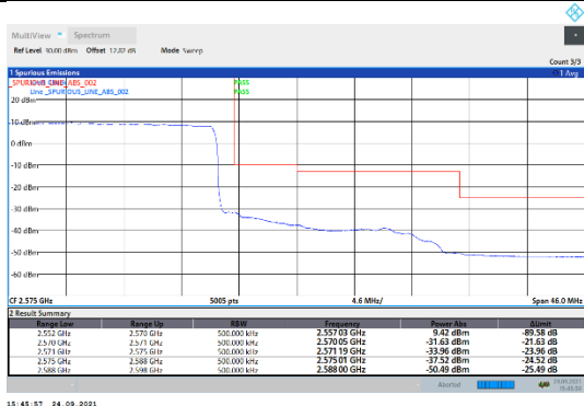
N7-15kHz-20MHz-DFT-QPSK-High-Outer_Full---PASS
