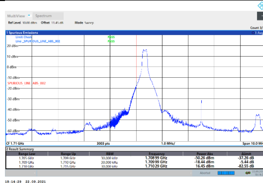
N66-15kHz-5MHz-DFT-QPSK-Low-Edge_1RB_Left--PASS
