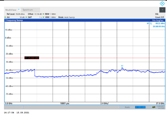
N41-30kHz-90MHz-DFT-QPSK-High-Edge_1RB_Left-3000-27000-PASS
