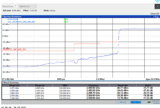
N7-15kHz-10MHz-DFT-QPSK-Low-Outer_Full---PASS
