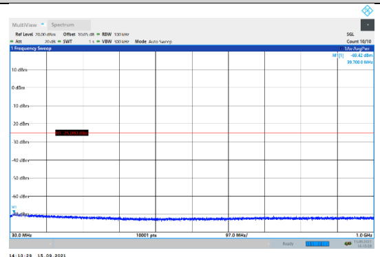
N41-30kHz-60MHz-DFT-QPSK-High-Edge_1RB_Left-30-1000-PASS
