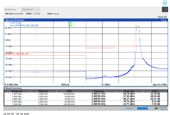
N7-15kHz-5MHz-CP-QPSK-Low-Edge_1RB_Left---PASS
