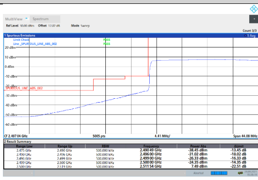
N7-15kHz-20MHz-CP-QPSK-Low-Outer_Full---PASS
