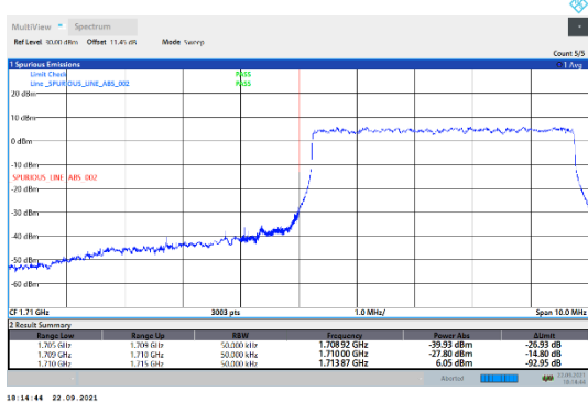
N66-15kHz-5MHz-DFT-QPSK-Low-Outer_Full---PASS
