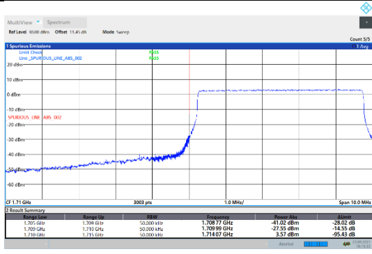
N66-15kHz-5MHz-CP-QPSK-Low-Outer_Full---PASS
