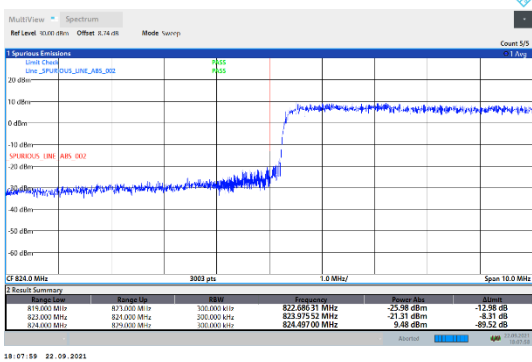
N5-15kHz-15MHz-DFT-QPSK-Low-Outer_Full---PASS
