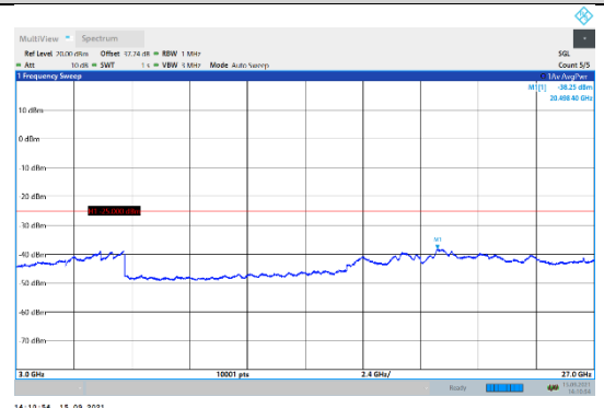
N41-30kHz-60MHz-DFT-QPSK-High-Edge_1RB_Left-3000-27000-PASS
