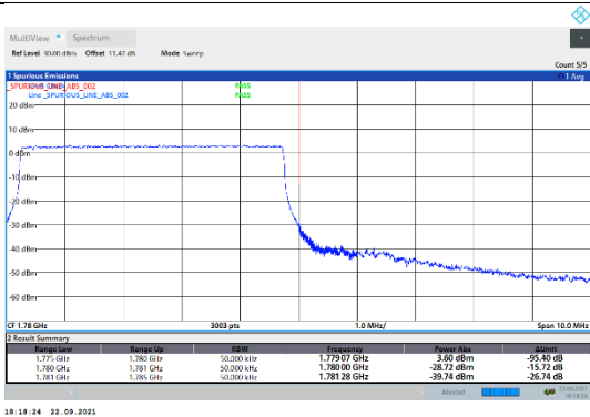
N66-15kHz-5MHz-CP-QPSK-High-Outer_Full---PASS
