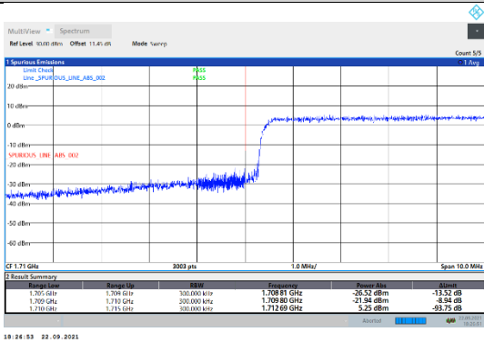
N66-15kHz-20MHz-CP-QPSK-Low-Outer_Full---PASS
