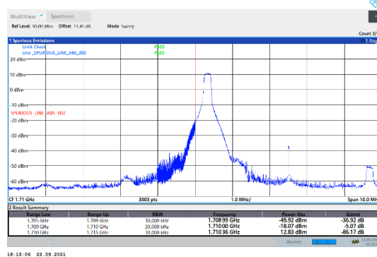
N66-15kHz-5MHz-CP-QPSK-Low-Edge_1RB_Left--PASS
