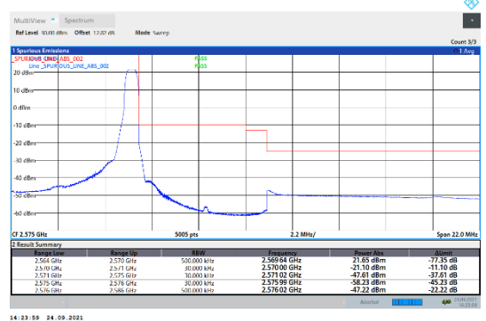
N7-15kHz-5MHz-CP-QPSK-High-Edge_1RB_Right---PASS
