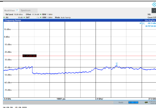
N41-30kHz-60MHz-DFT-QPSK-Mid-Edge_1RB_Left-3000-27000-PASS
