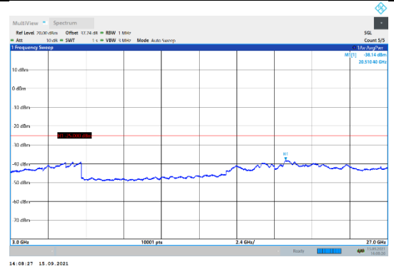
N41-30kHz-60MHz-DFT-QPSK-Low-Edge_1RB_Left-3000-27000-PASS
