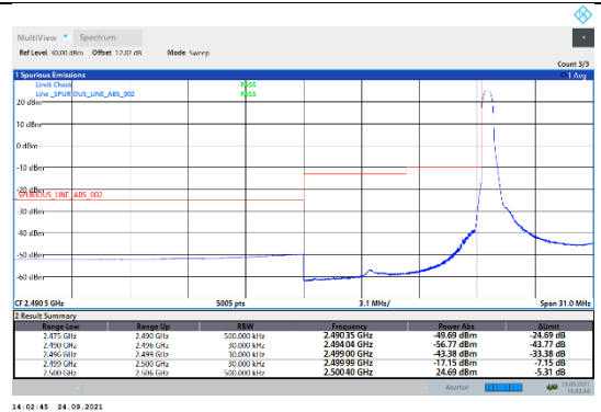
N7-15kHz-5MHz-DFT-QPSK-Low-Edge_1RB_Left---PASS
