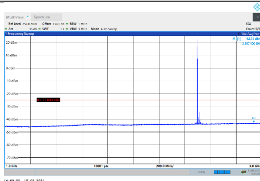
N41-30kHz-40MHz-DFT-QPSK-Low-Edge_1RB_Left-1000-3000-PASS
