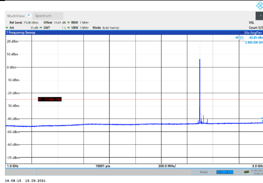
N41-30kHz-60MHz-DFT-QPSK-Low-Edge_1RB_Left-1000-3000-PASS
