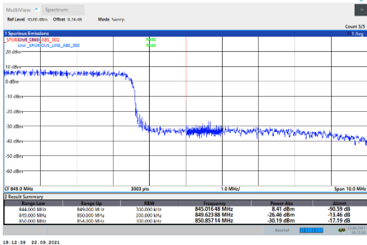
N5-15kHz-20MHz-DFT-QPSK-High-Outer_Full---PASS
