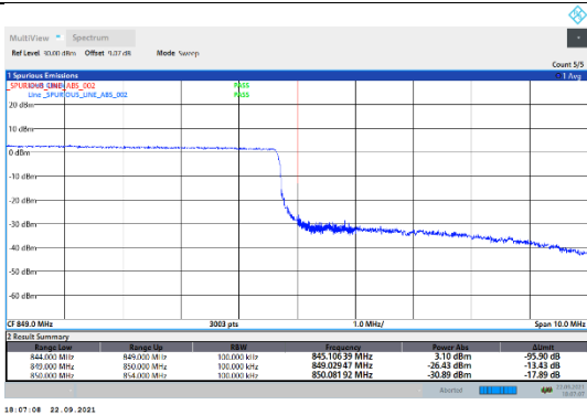
N5-15kHz-10MHz-CP-QPSK-High-Outer_Full---PASS
