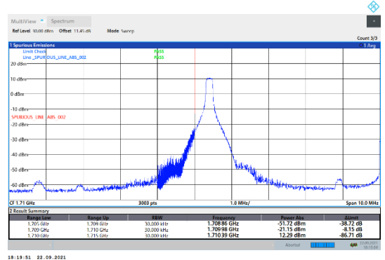
N66-15kHz-10MHz-CP-QPSK-Low-Edge_1RB_Left---PASS
