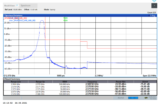
N7-15kHz-15MHz-DFT-QPSK-High-Edge_1RB_Right--PASS
