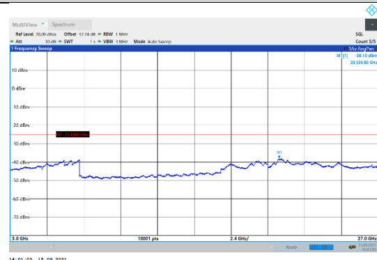
N41-30kHz-40MHz-DFT-QPSK-Low-Edge_1RB_Left-3000-27000-PASS
