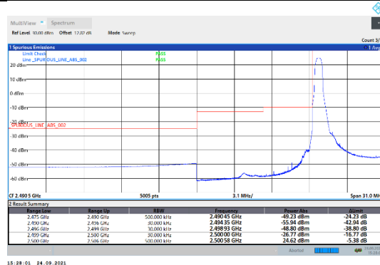
N7-15kHz-20MHz-DFT-QPSK-Low-Edge_1RB_Left--PASS
