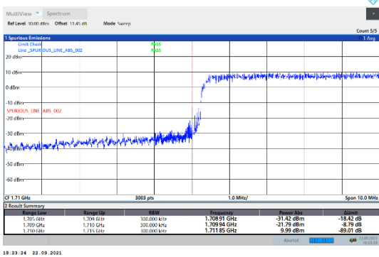
N66-15kHz-15MHz-DFT-QPSK-Low-Outer_Full---PASS
