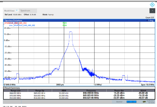
N5-15kHz-20MHz-CP-QPSK-High-Edge_1RB_Right--PASS
