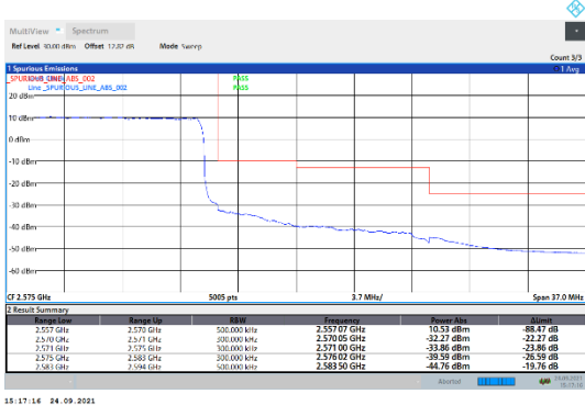
N7-15kHz-15MHz-DFT-QPSK-High-Outer_Full---PASS
