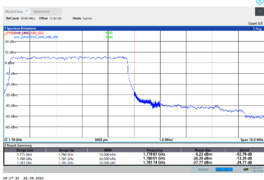
N66-15kHz-5MHz-DFT-QPSK-High-Outer_Full---PASS
