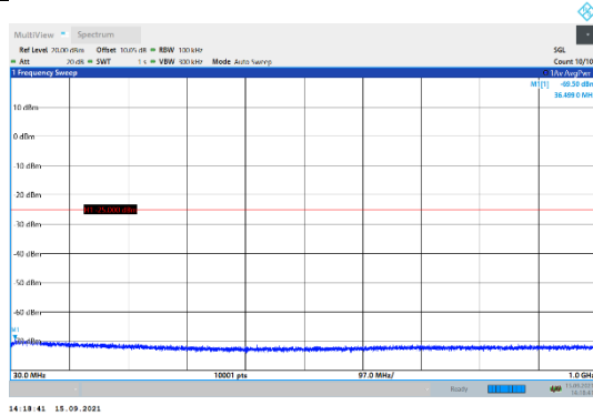
N41-30kHz-100MHz-DFT-QPSK-Low-Edge_1RB_Left-30-1000-PASS
