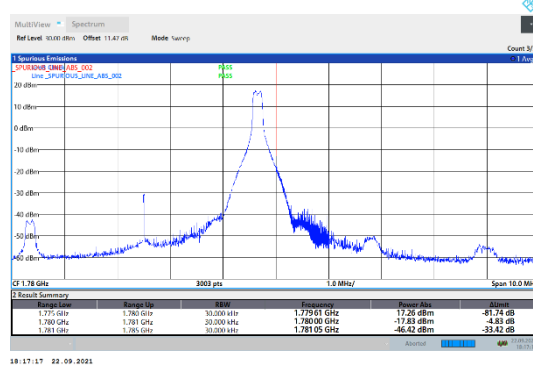
N66-15kHz-5MHz-DFT-QPSK-High-Edge_1RB_Right--PASS
