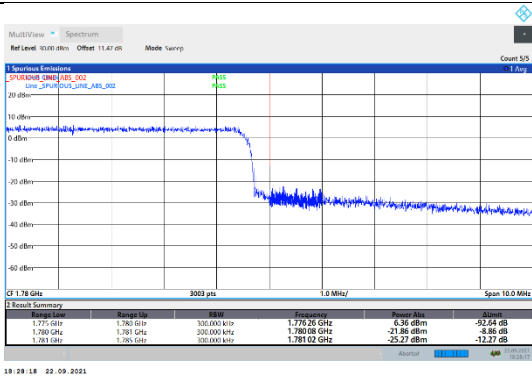
N66-15kHz-20MHz-CP-QPSK-High-Outer_Full---PASS
