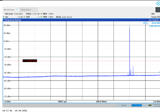
N41-30kHz-90MHz-DFT-QPSK-High-Edge_1RB_Left-1000-3000-PASS
