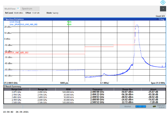
N7-15kHz-15MHz-CP-QPSK-Low-Edge_1RB_Left--PASS
