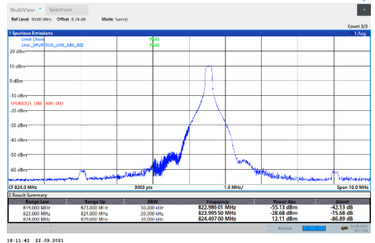
N5-15kHz-20MHz-CP-QPSK-Low-Edge_1RB_Left--PASS
