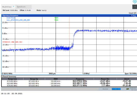
N5-15kHz-20MHz-DFT-QPSK-Low-Outer_Full---PASS
