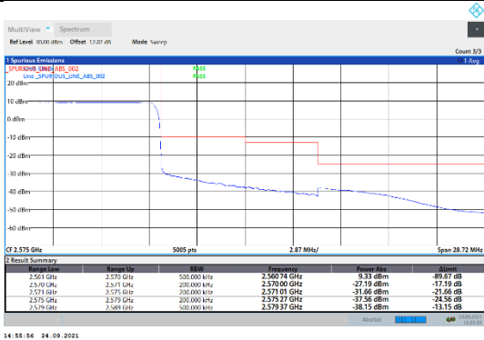
N7-15kHz-10MHz-CP-QPSK-High-Outer_Full---PASS
