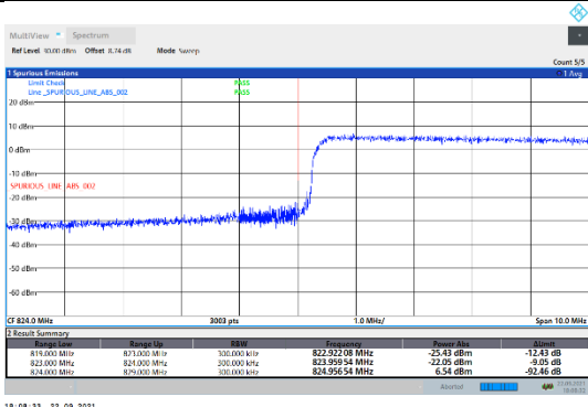
N5-15kHz-15MHz-CP-QPSK-Low-Outer_Full---PASS
