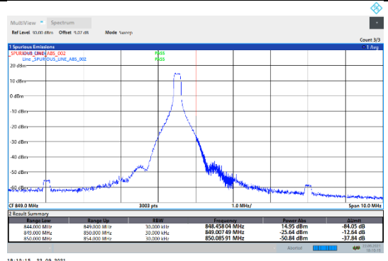
N5-15kHz-15MHz-CP-QPSK-High-Edge_1RB_Right--PASS
