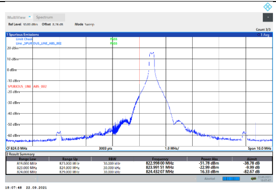
N5-15kHz-15MHz-DFT-QPSK-Low-Edge_1RB_Left--PASS
