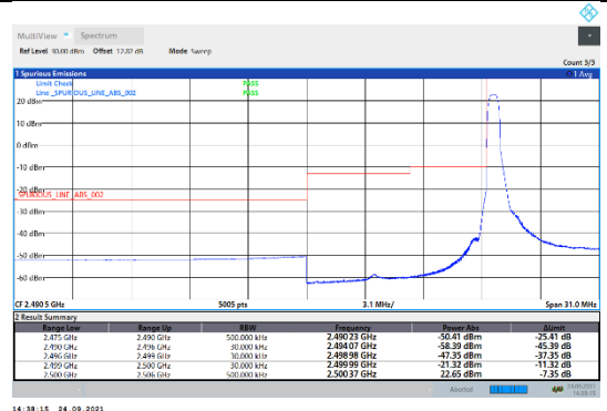
N7-15kHz-10MHz-CP-QPSK-Low-Edge_1RB_Left--PASS
