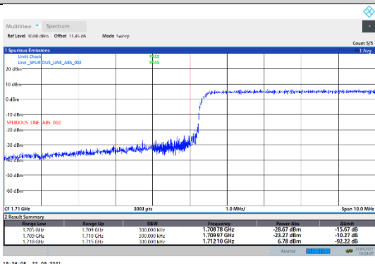
N66-15kHz-15MHz-CP-QPSK-Low-Outer_Full---PASS
