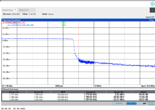
N66-15kHz-10MHz-CP-QPSK-High-Outer_Full---PASS
