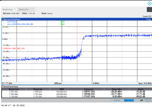
N66-15kHz-20MHz-DFT-QPSK-Low-Outer_Full---PASS
