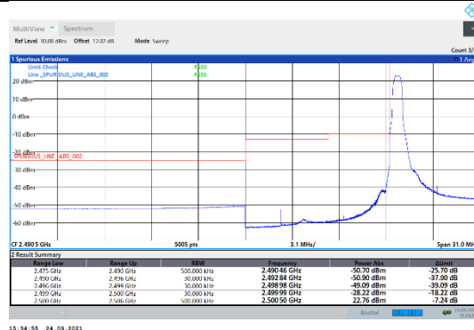
N7-15kHz-20MHz-CP-QPSK-Low-Edge_1RB_Left---PASS
