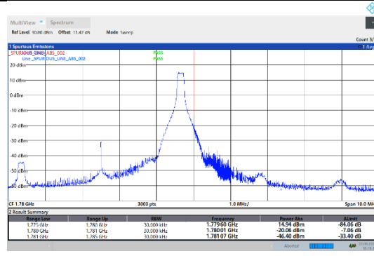
N66-15kHz-5MHz-CP-QPSK-High-Edge_1RB_Right--PASS
