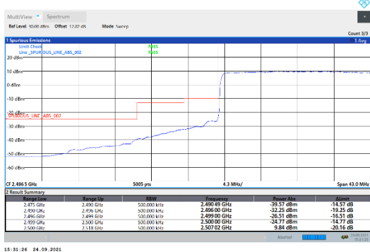
N7-15kHz-20MHz-DFT-QPSK-Low-Outer_Full---PASS
