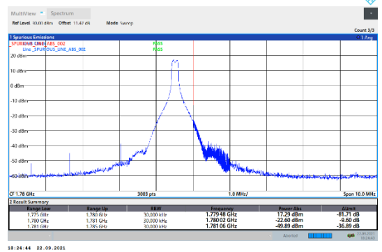
N66-15kHz-15MHz-DFT-QPSK-High-Edge_1RB_Right---PASS
