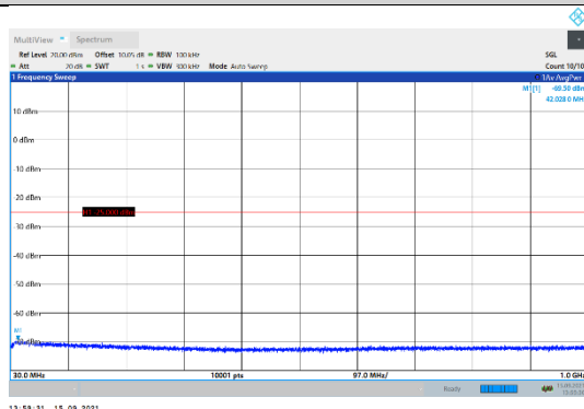
N41-30kHz-30MHz-DFT-QPSK-High-Edge_1RB_Left-30-1000-PASS
