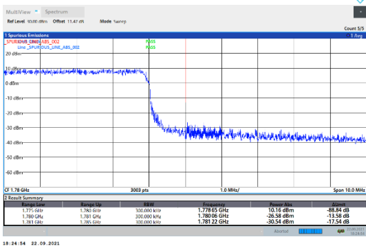
N66-15kHz-15MHz-DFT-QPSK-High-Outer_Full---PASS
