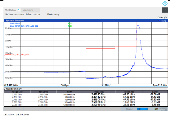
N7-15kHz-10MHz-DFT-QPSK-Low-Edge_1RB_Left--PASS
