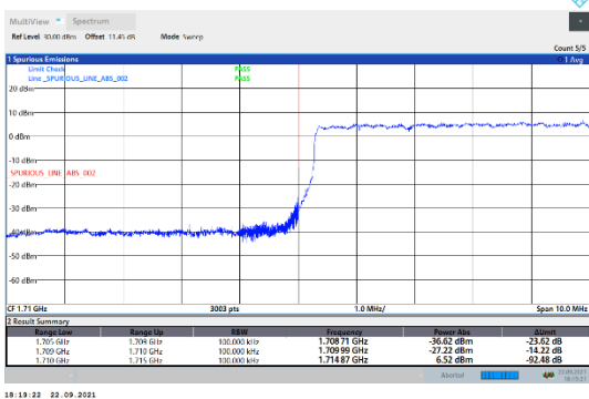
N66-15kHz-10MHz-DFT-QPSK-Low-Outer_Full---PASS
