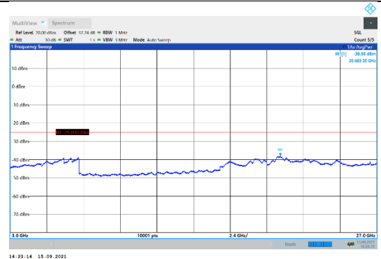
N41-30kHz-100MHz-DFT-QPSK-Mid-Edge_1RB_Left-3000-27000-PASS
