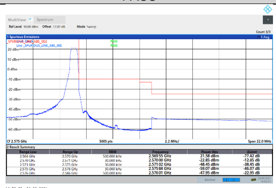
N7-15kHz-10MHz-CP-QPSK-High-Edge_1RB_Right--PASS
