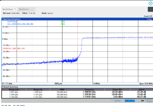
N66-15kHz-10MHz-CP-QPSK-Low-Outer_Full---PASS
