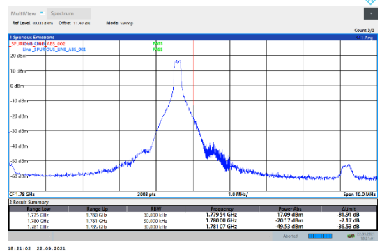
N66-15kHz-10MHz-DFT-QPSK-High-Edge_1RB_Right---PASS
