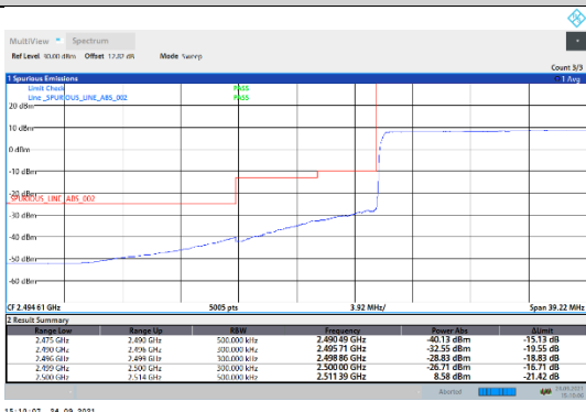
N7-15kHz-15MHz-CP-QPSK-Low-Outer_Full---PASS
