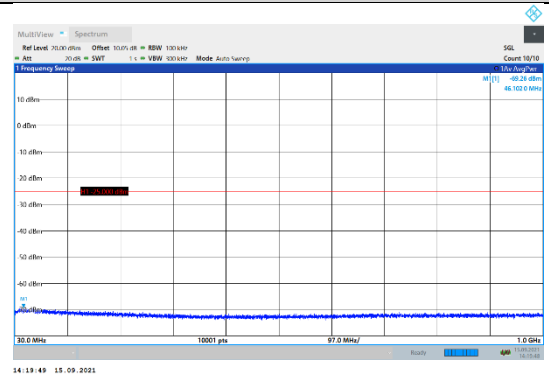
N41-30kHz-100MHz-DFT-QPSK-Mid-Edge_1RB_Left-30-1000-PASS
