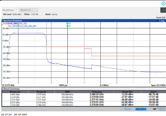
N7-15kHz-5MHz-CP-QPSK-High-Outer_Full---PASS
