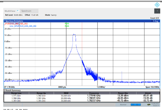
N66-15kHz-15MHz-CP-QPSK-High-Edge_1RB_Right---PASS
