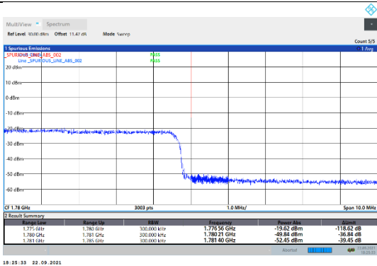
N66-15kHz-15MHz-CP-QPSK-High-Outer_Full---PASS
