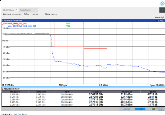
N7-15kHz-10MHz-DFT-QPSK-High-Outer_Full---PASS
