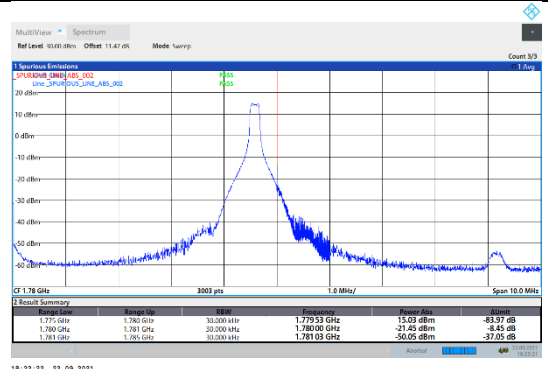
N66-15kHz-10MHz-CP-QPSK-High-Edge_1RB_Right---PASS
