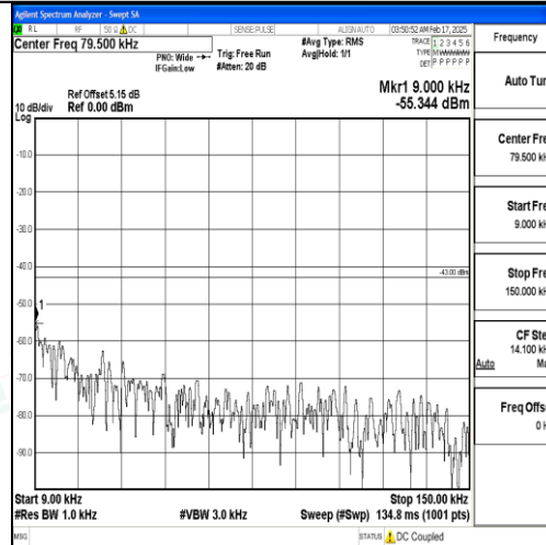
Band25_10MHz_16QAM_26640_1RB#0_0.009~0.15_0.009~0.15
