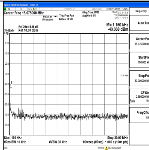
Band25_10MHz_16QAM_26640_1RB#0_0.15~30_0.15~30
