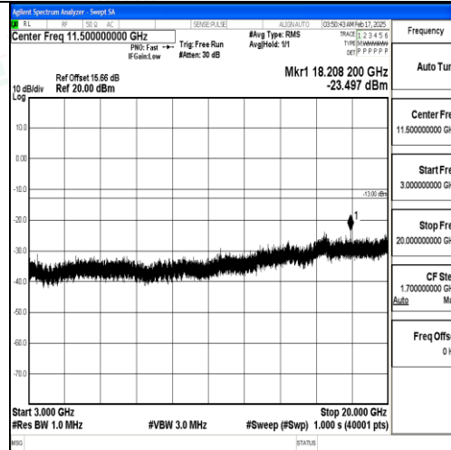
Band25_10MHz_QPSK_26640_1RB#0_3000~20000_3000~20000
