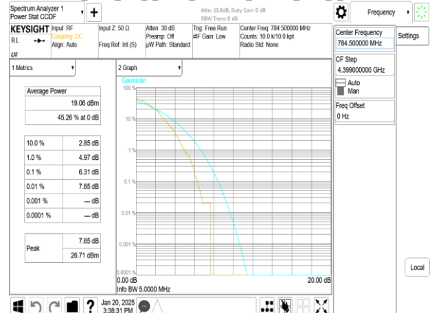
Band13_5MHz_DFT_s_OFDM_SCS15kHz_256QAM_RB25_0_CH156900
