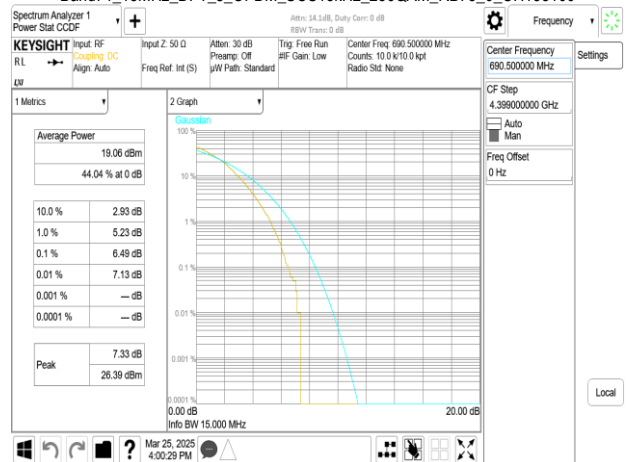
Band71_15MHz_DFT_s_OFDM_SCS15kHz_256QAM_RB75_0_CH138100
