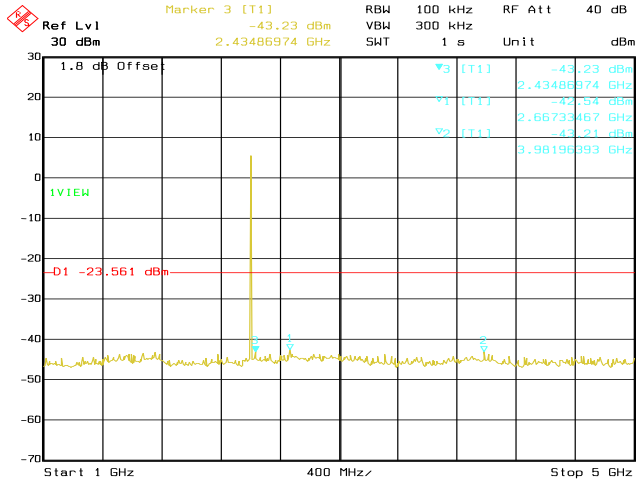
Date: 14.AUG.2020 03:01:45 Conducted Emissions. Bluetooth LE, Frequency 2402 MHz Emission Level, 1 GHz -> 5 GHz
