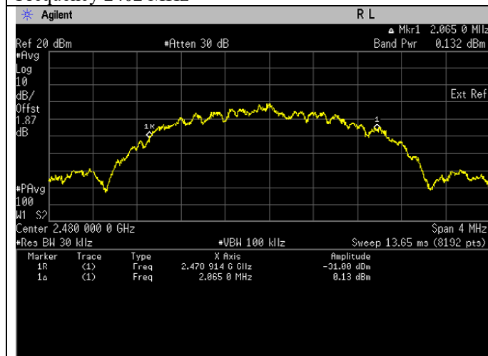
Frequency 2480 MHz
