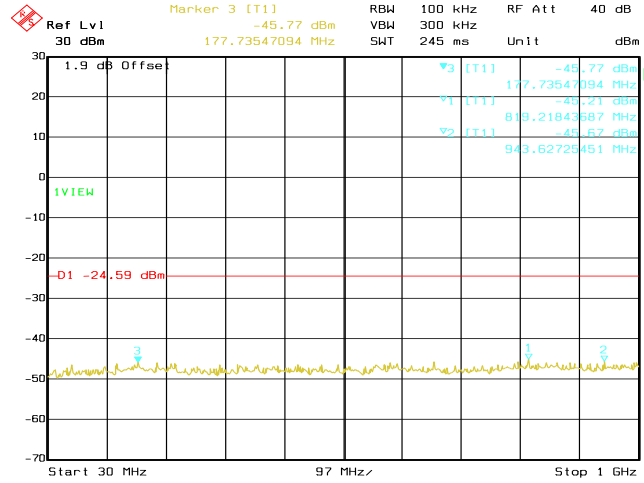
Date: 14.AUG.2020 02:52:12 Conducted Emissions. Bluetooth LE, Frequency 2480 MHz Emission Level, 30 MHz -> 1 GHz
