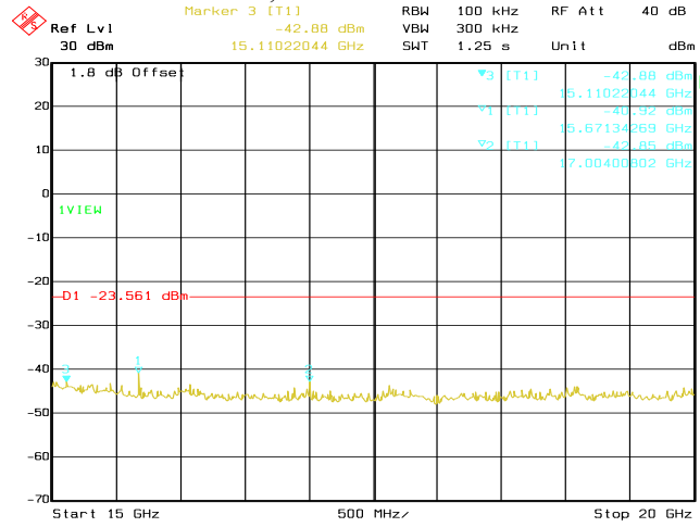
Date: 14.AUG.2020 03:04:24 Conducted Emissions. Bluetooth LE, Frequency 2402 MHz Emission Level, 15 GHz -> 20 GHz
