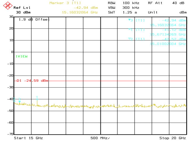
Date: 14.AUG.2020 02:55:46 Conducted Emissions. Bluetooth LE, Frequency 2480 MHz Emission Level, 15 GHz -> 20 GHz
