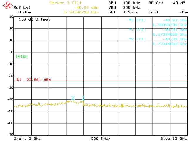
Date: 14.AUG.2020 03:02:38 Conducted Emissions. Bluetooth LE, Frequency 2402 MHz Emission Level, 5 GHz -> 10 GHz
