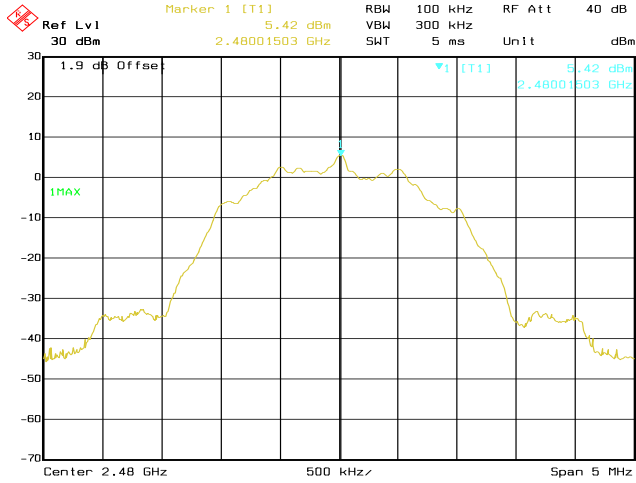
Date: 14.AUG.2020 02:51:19 Conducted Emissions. Bluetooth LE, Frequency 2480 MHz Reference Level
