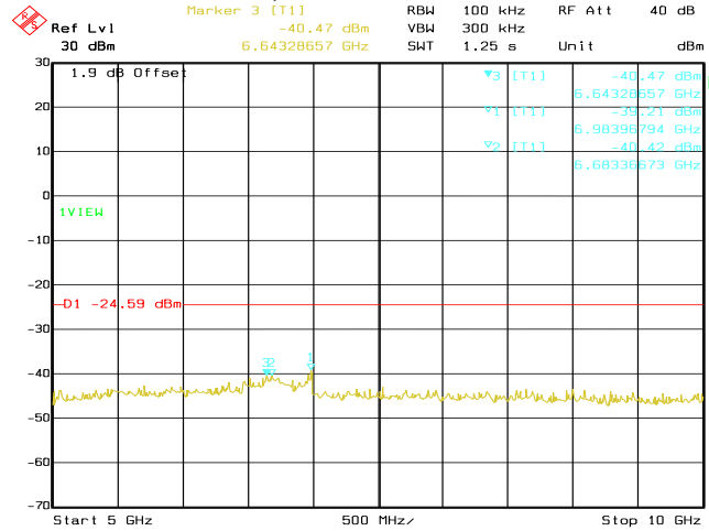
Date: 14.AUG.2020 02:53:59 Conducted Emissions. Bluetooth LE, Frequency 2480 MHz Emission Level, 5 GHz -> 10 GHz
