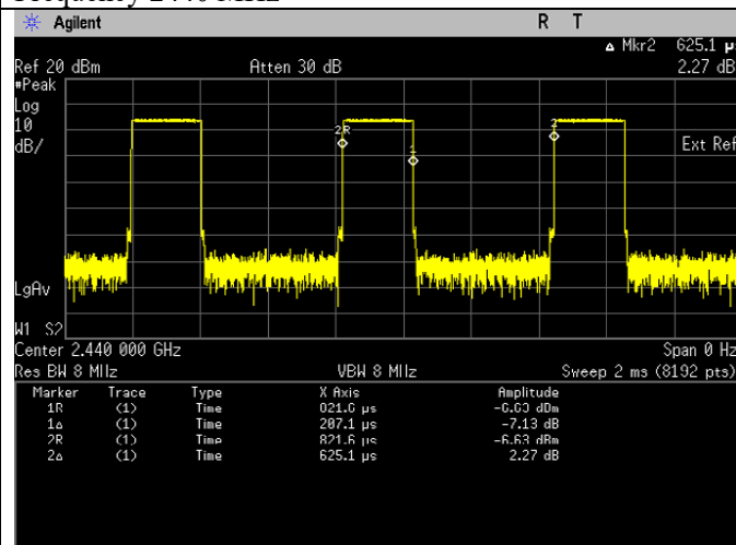
Duty Cycle
