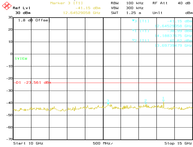
Date: 14.AUG.2020 03:03:31 Conducted Emissions. Bluetooth LE, Frequency 2402 MHz Emission Level, 10 GHz -> 15 GHz
