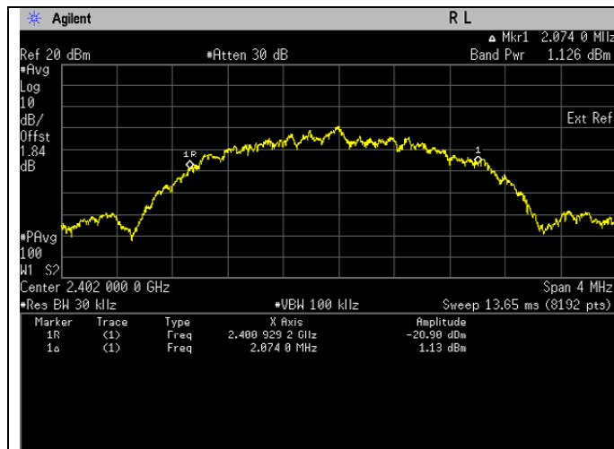
Frequency 2402 MHz
