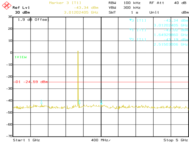
Date: 14.AUG.2020 02:53:06 Conducted Emissions. Bluetooth LE, Frequency 2480 MHz Emission Level, 1 GHz -> 5 GHz
