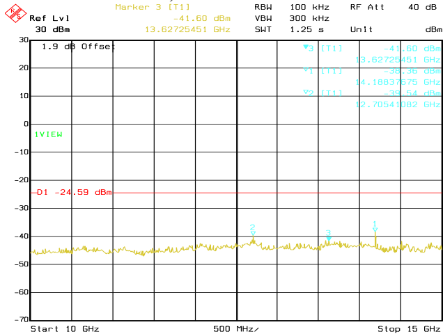
Date: 14.AUG.2020 02:54:52 Conducted Emissions. Bluetooth LE, Frequency 2480 MHz Emission Level, 10 GHz -> 15 GHz
