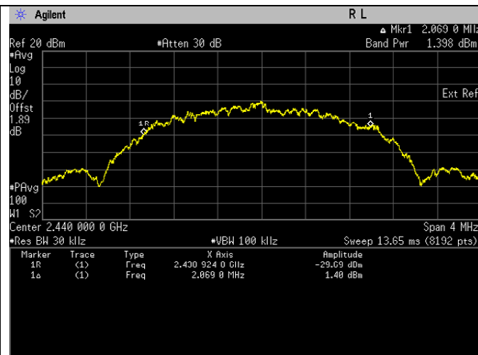
Frequency 2440 MHz
