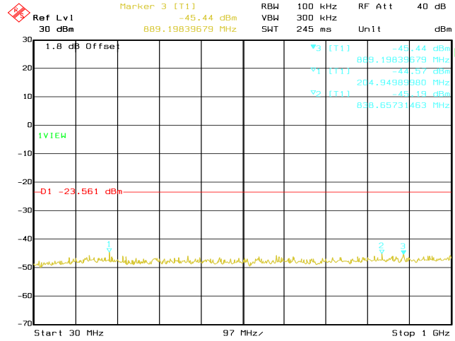
Date: 14.AUG.2020 03:00:51 Conducted Emissions. Bluetooth LE, Frequency 2402 MHz Emission Level, 30 MHz -> 1 GHz
