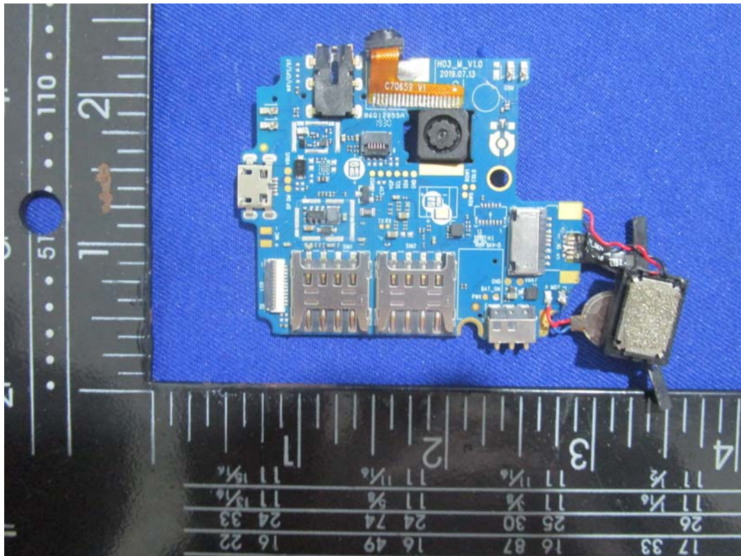
Main chip
