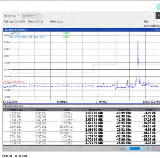
1-N48-30-30-H-2-DFT-PI2BPSK-Edge_1RB_Right-1@77-Ant0-1--PASS-see graph
