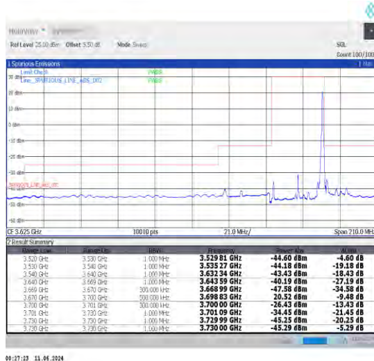
1-N48-30-30-H-5-CP-QPSK-Edge_1RB_Right-1@77-Ant0-1--PASS-see graph
