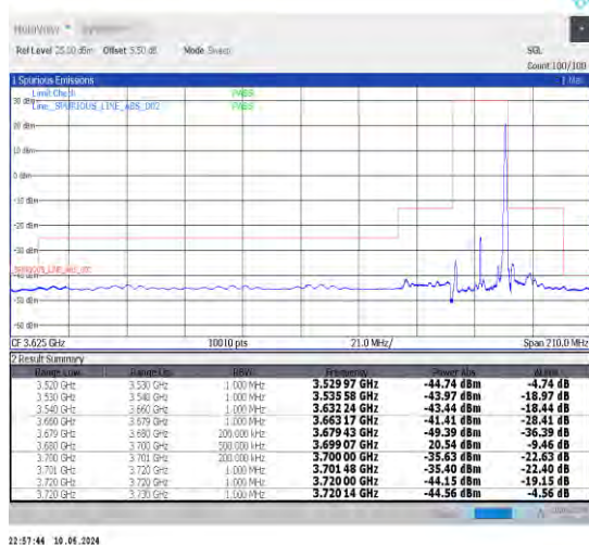
1-N48-30-20-H-5-CP-QPSK-Edge_1RB_Right-1@50-Ant0-1--PASS-see graph
