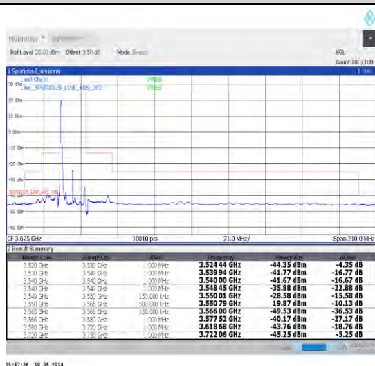
1-N48-30-15-L-4-CP-QPSK-Edge_1RB_Left-1@0-Ant0-1--PASS-see graph
