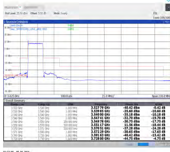
1-N48-30-20-L-3-DFT-PI2BPSK-Outer_Full-50@0-Ant0-1--PASS-see graph
