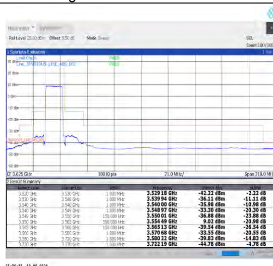
1-N48-30-15-L-3-DFT-PI2BPSK-Outer_Full-36@0-Ant0-1--PASS-see graph
