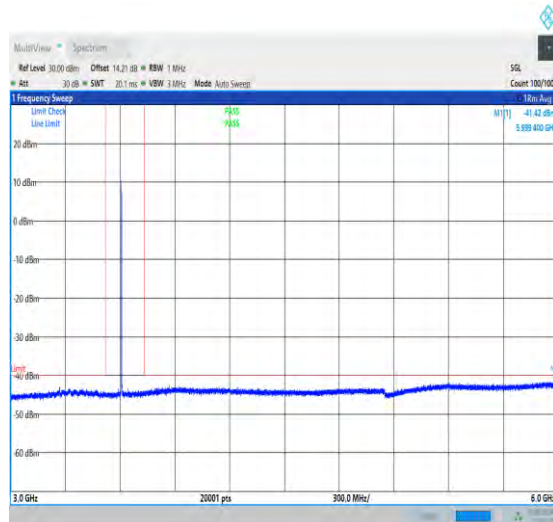
NTNV_N48_PC3_30_40_M_TID1_NS_01_3000_6000_#1
