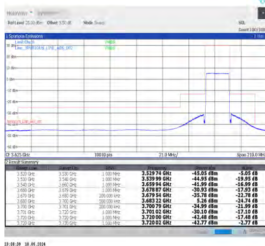
1-N48-30-20-H-6-CP-QPSK-Outer_Full-51@0-Ant0-1--PASS-see graph
