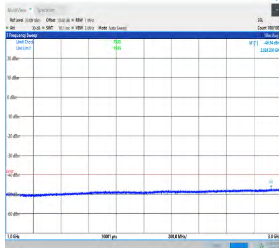
NTNV_N48_PC3_30_40_H_TID1_NS_01_1000_3000_#1
