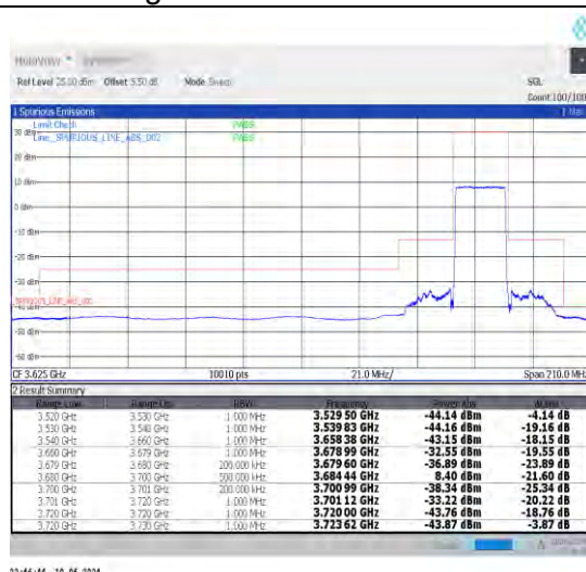
1-N48-30-20-H-3-DFT-PI2BPSK-Outer_Full-50@0-Ant0-1--PASS-see graph
