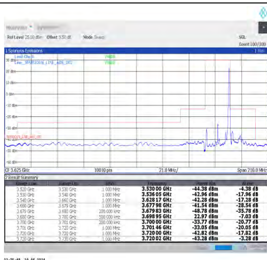
1-N48-30-20-H-2-DFT-PI2BPSK-Edge_1RB_Right-1@50-Ant0-1--PASS-see graph
