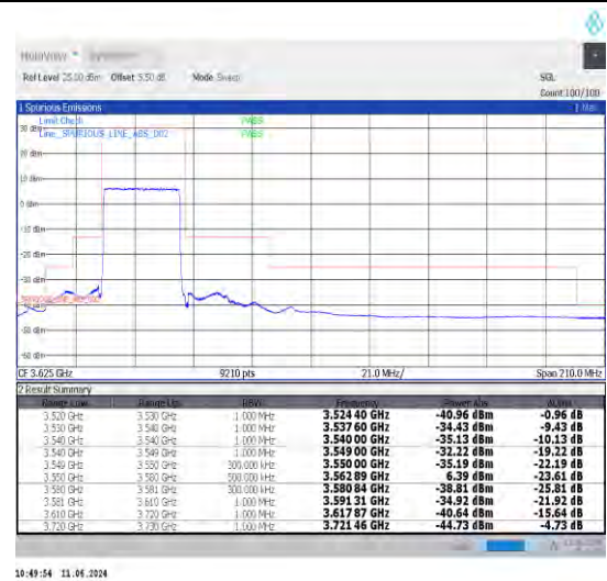
1-N48-30-30-L-3-DFT-PI2BPSK-Outer_Full-75@0-Ant0-1--PASS-see graph
