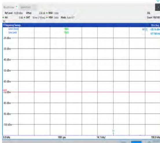
NTVN_N48_PC3_30_40_H_TID1_NS_01_0.009_0.15_#1
