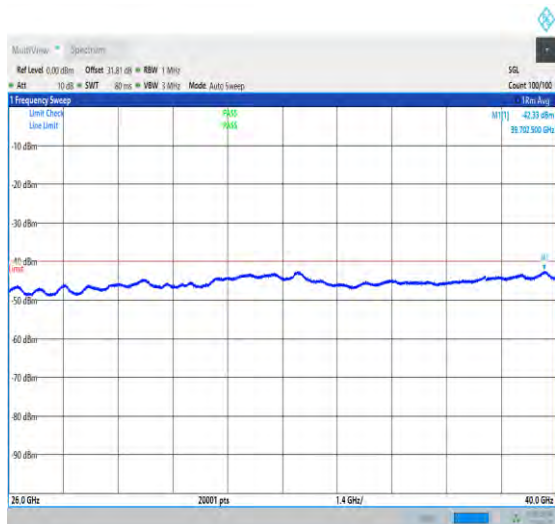
NTVN_N48_PC3_30_40_L_TID1_NS_01_26000_40000_#1
