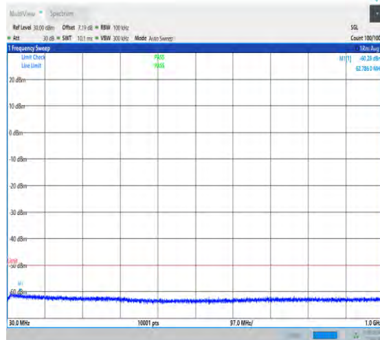
NTNV_N48_PC3_30_40_M_TID1_NS_01_30_1000_#1
