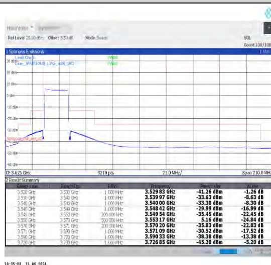
1-N48-30-20-L-6-CP-QPSK-Outer_Full-51@0-Ant0-1--PASS-see graph
