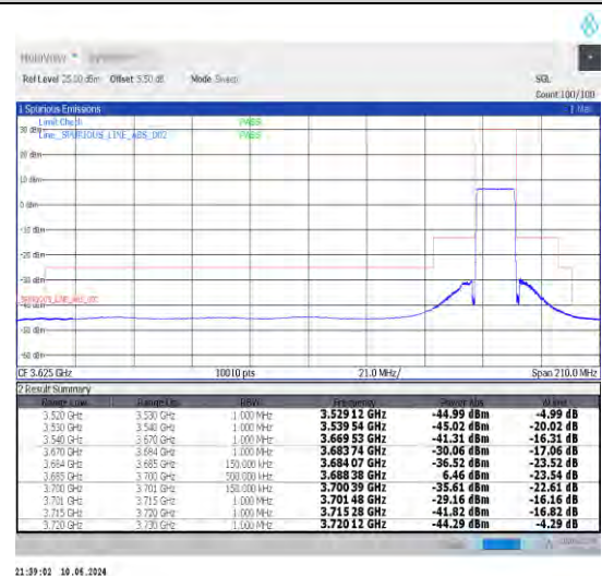
1-N48-30-15-H-6-CP-QPSK-Outer_Full-38@0-Ant0-1--PASS-see graph
