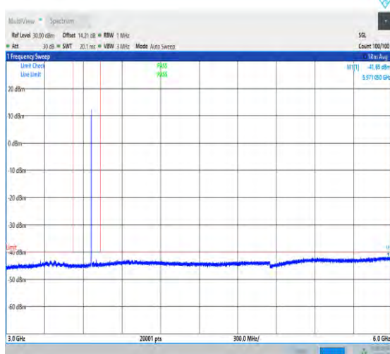
NTNV_N48_PC3_30_40_H_TID1_NS_01_3000_6000_#1
