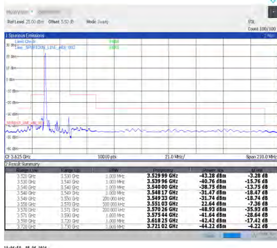
1-N48-30-20-L-1-DFT-PI2BPSK-Edge_1RB_Left-1@0-Ant0-1--PASS-see graph
