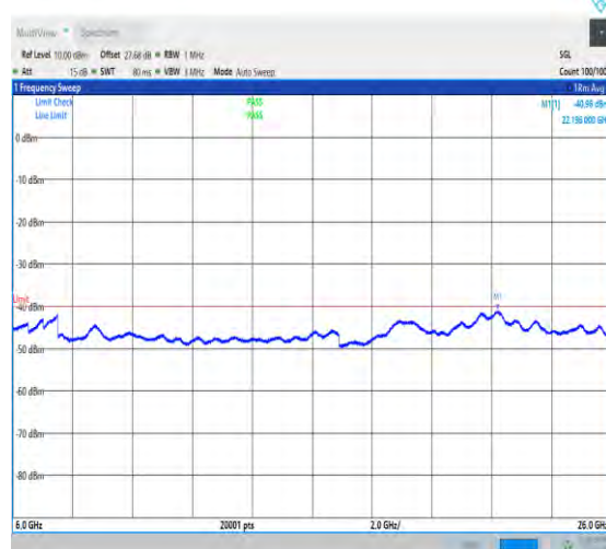
NTNV_N48_PC3_30_40_H_TID1_NS_01_6000_26000_#
