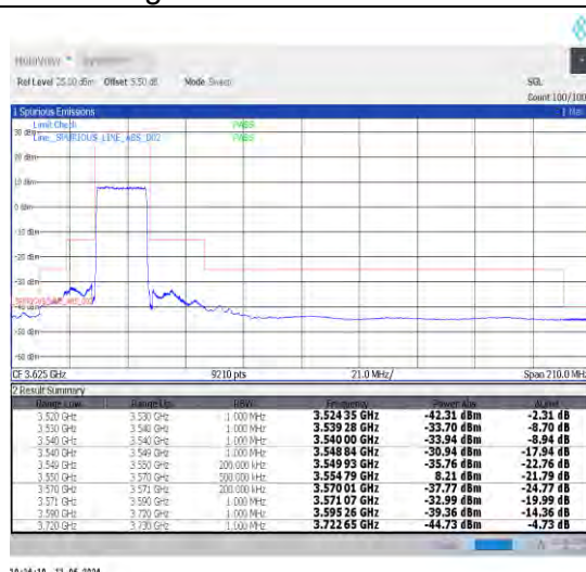
1-N48-30-20-L-3-DFT-PI2BPSK-Outer_Full-50@0-Ant0-1--PASS-see graph
