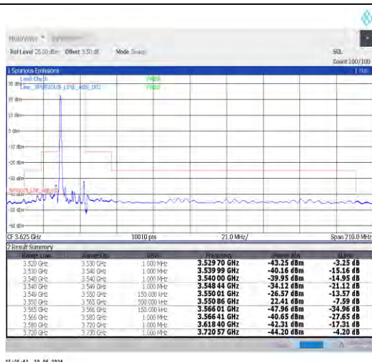
1-N48-30-15-L-1-DFT-PI2BPSK-Edge_1RB_Left-1@0-Ant0-1--PASS-see graph
