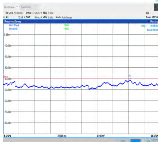
NTNV_N48_PC3_30_40_H_TID1_NS_01_6000_26000_#
