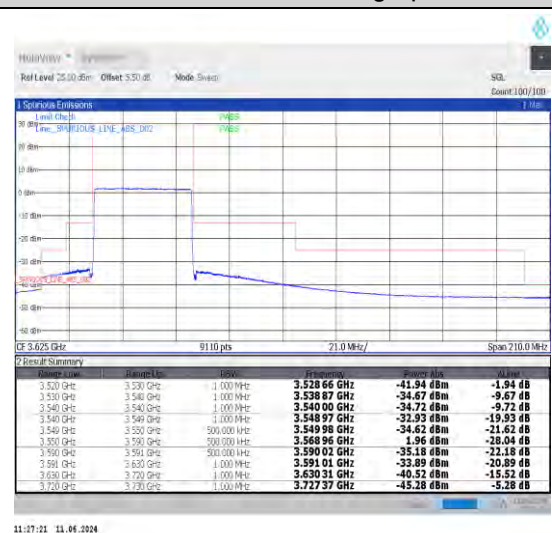
1-N48-30-40-L-6-CP-QPSK-Outer_Full-106@0-Ant0-1--PASS-see graph
