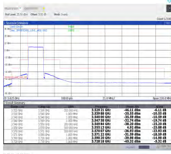
1-N48-30-20-L-6-CP-QPSK-Outer_Full-51@0-Ant0-1--PASS-see graph
