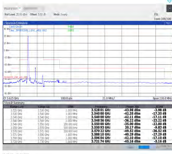
1-N48-30-20-L-4-CP-QPSK-Edge_1RB_Left-1@0-Ant0-1--PASS-see graph
