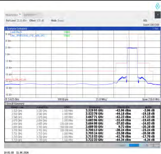
1-N48-30-15-H-3-DFT-PI2BPSK-Outer_Full-36@0-Ant0-1--PASS-see graph
