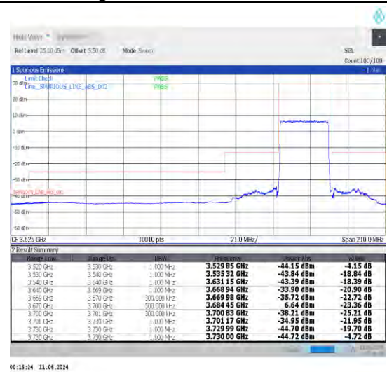
1-N48-30-30-H-3-DFT-PI2BPSK-Outer_Full-75@0-Ant0-1--PASS-see graph
