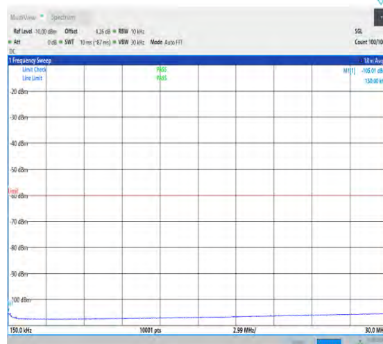
NTVN_N48_PC3_30_40_H_TID1_NS_01_0.15_30_#1
