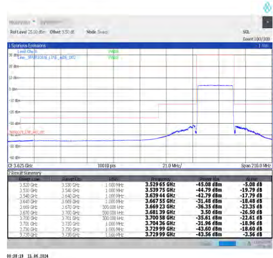
1-N48-30-30-H-6-CP-QPSK-Outer_Full-78@0-Ant0-1--PASS-see graph
