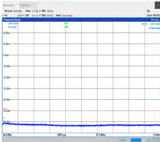
NTNV_N48_PC3_30_40_H_TID1_NS_01_30_1000_#1
