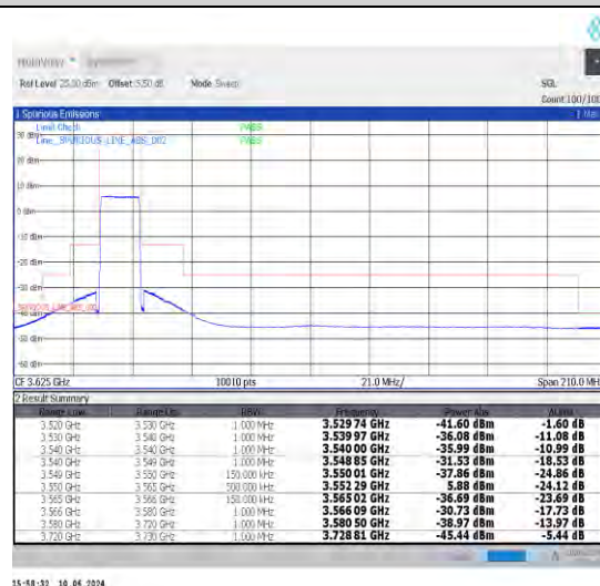
1-N48-30-15-L-6-CP-QPSK-Outer_Full-38@0-Ant0-1--PASS-see graph
