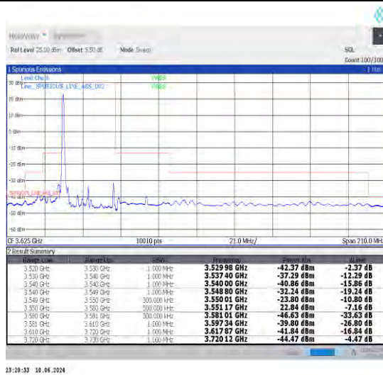
1-N48-30-30-L-1-DFT-PI2BPSK-Edge_1RB_Left-1@0-Ant0-1--PASS-see graph
