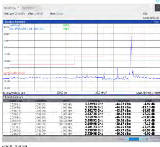
1-N48-30-40-H-5-CP-QPSK-Edge_1RB_Right-1@105- Ant0-1--PASS-see graph
