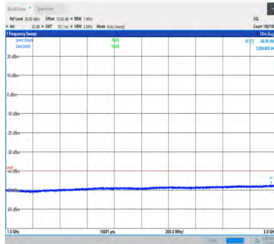
NTNV_N48_PC3_30_40_H_TID1_NS_01_1000_3000_#1
