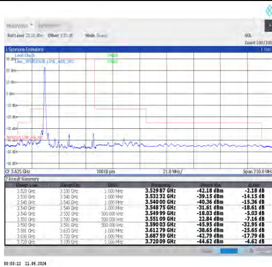
1-N48-30-40-L-1-DFT-PI2BPSK-Edge_1RB_Left-1@0-Ant0-1--PASS-see graph
