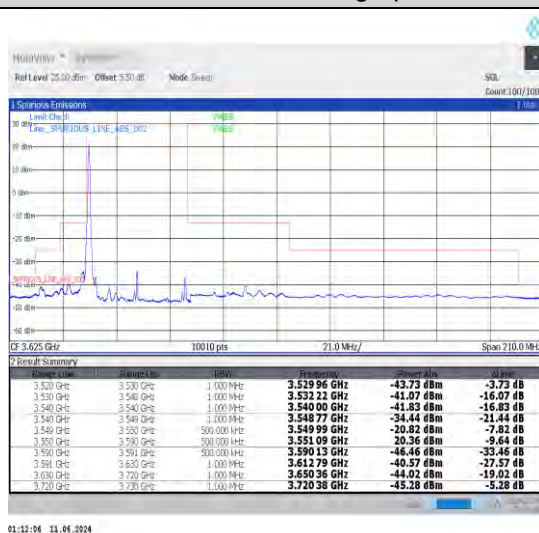
1-N48-30-40-L-4-CP-QPSK-Edge_1RB_Left-1@0-Ant0-1--PASS-see graph
