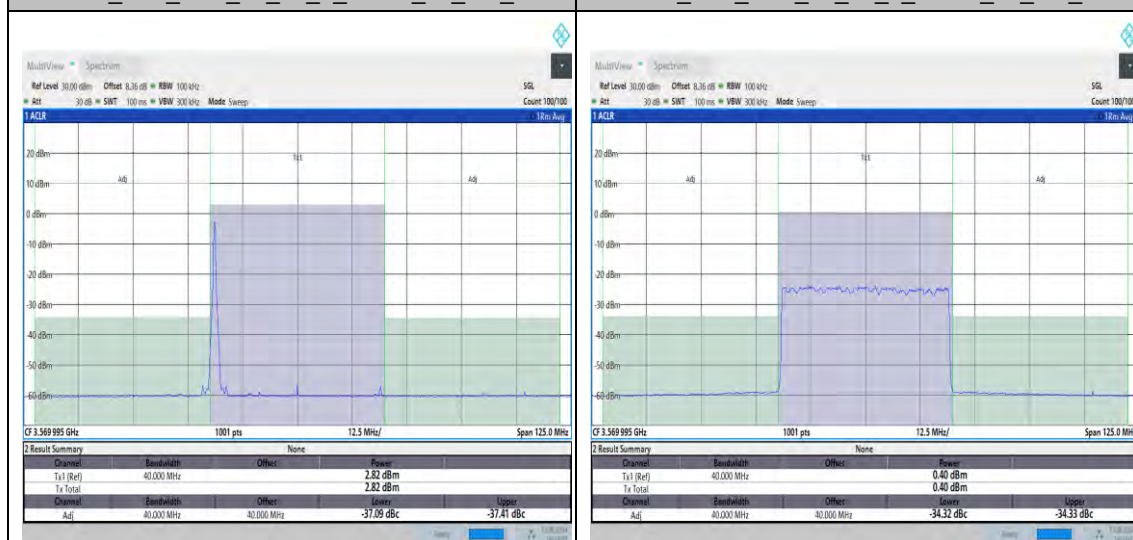
NTNV_N48_PC3_30_40_L_TID23_#1_-40_40
