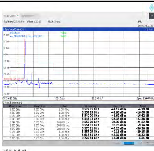
1-N48-30-20-L-4-CP-QPSK-Edge_1RB_Left-1@0-Ant0-1--PASS-see graph
