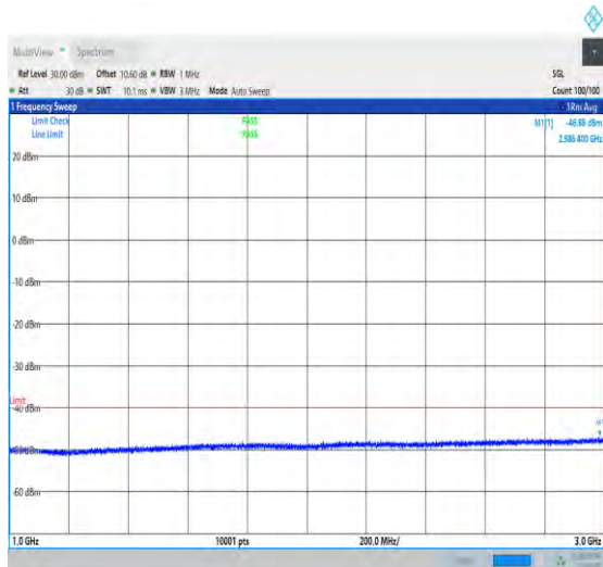
NTNV_N48_PC3_30_40_M_TID1_NS_01_1000_3000_#1
