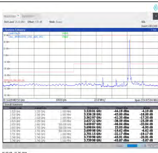
1-N48-30-40-H-2-DFT-PI2BPSK-Edge_1RB_Right-1@ 105-Ant0-1--PASS-see graph
