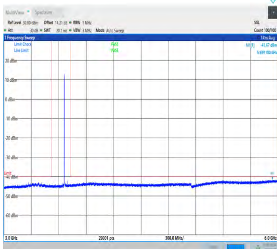
NTNV_N48_PC3_30_40_H_TID1_NS_01_3000_6000_#1
