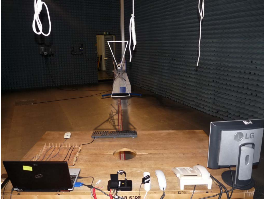
Photo 2: Test setup for radiated measurements (computer peripheral setup, EUT supplied by AC/DC Adaptor @ 120v/60Hz, unintentional radiator §15)
