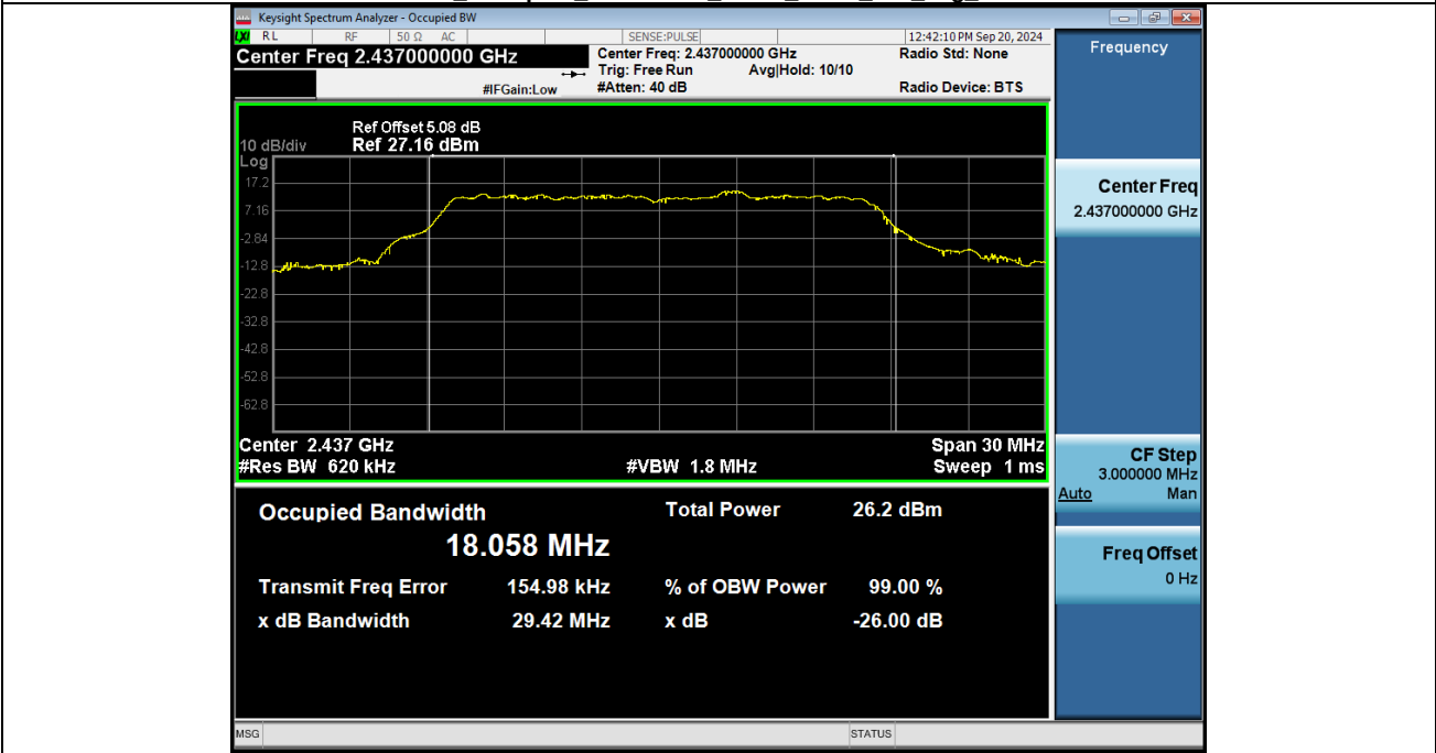
99% Occupied_Bandwidth_NVNT_ANT2_802_11g_2437
