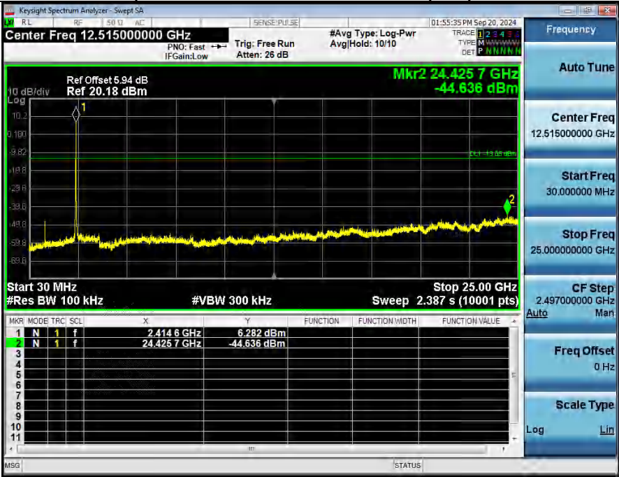
2 Spurious Emission_NVNT_ANT2_802_11n(HT20)_2412
