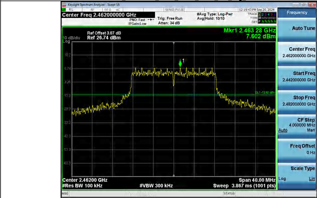
2_Bandedge_NVNT_ANT1_802_11g_2462
