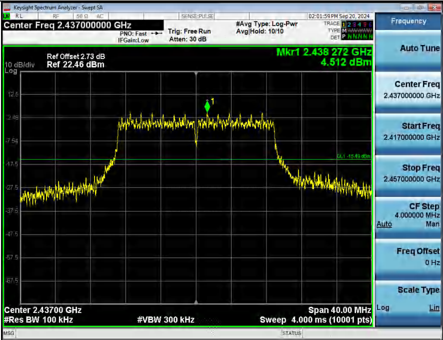
2 Spurious Emission NVNT_ANT1_802_11n(HT20)_2437
