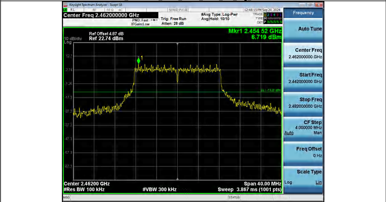
2 Spurious_Emission_NVNT_ANT2_802_11g_2462
