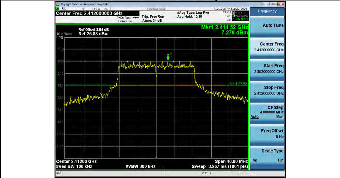
2 Spurious Emission_NVNT_ANT1_802_11g_2412
