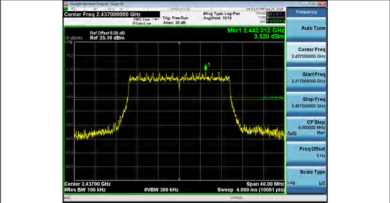
1 Reference_Level_NVNT_ANT2_802_11ax(HE20)_2437
