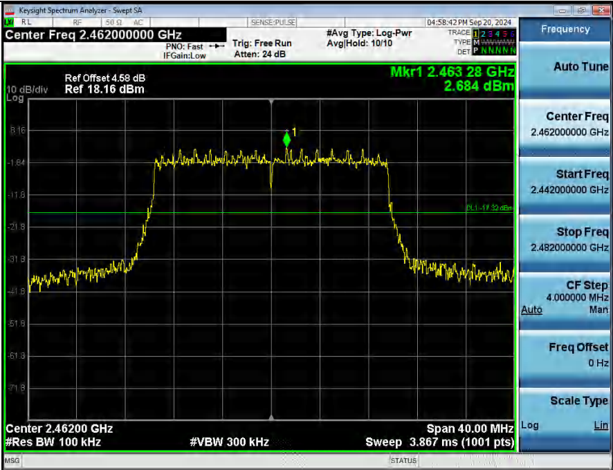
2_Spurious_Emission_NVNT_ANT1_802_11ax(HE20)_2462
