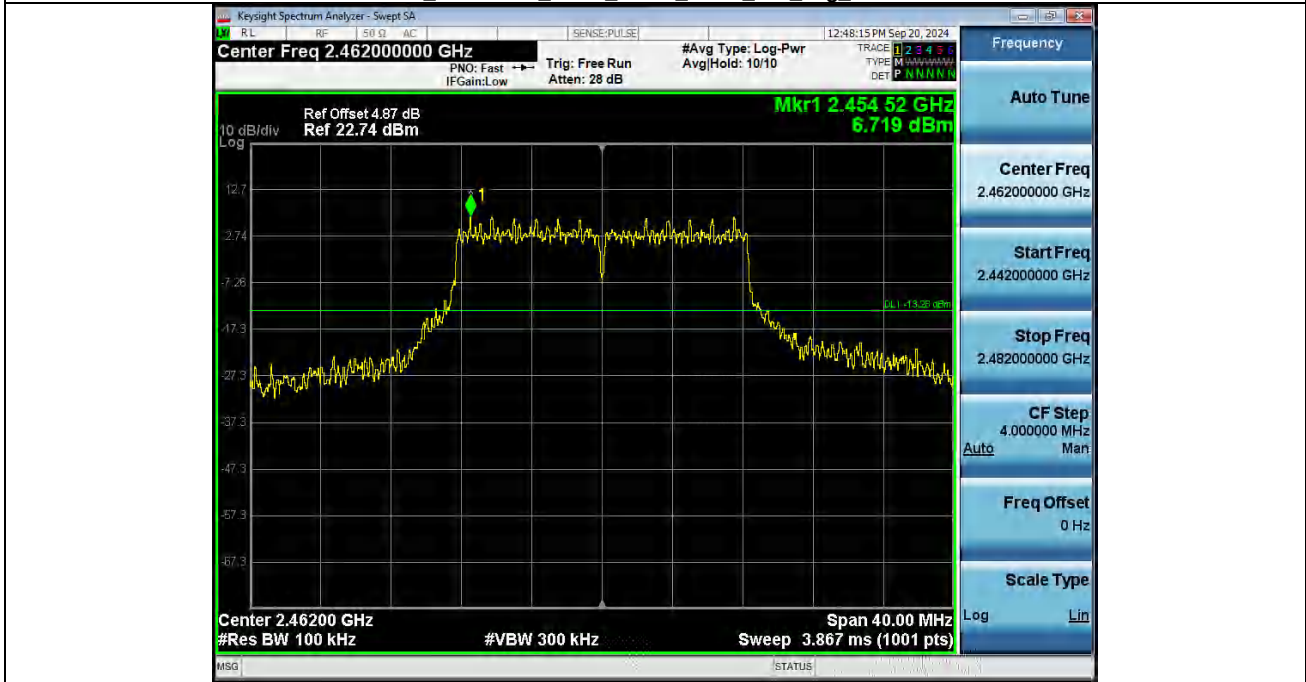
2_Bandedge_NVNT_ANT2_802_11g_2462
