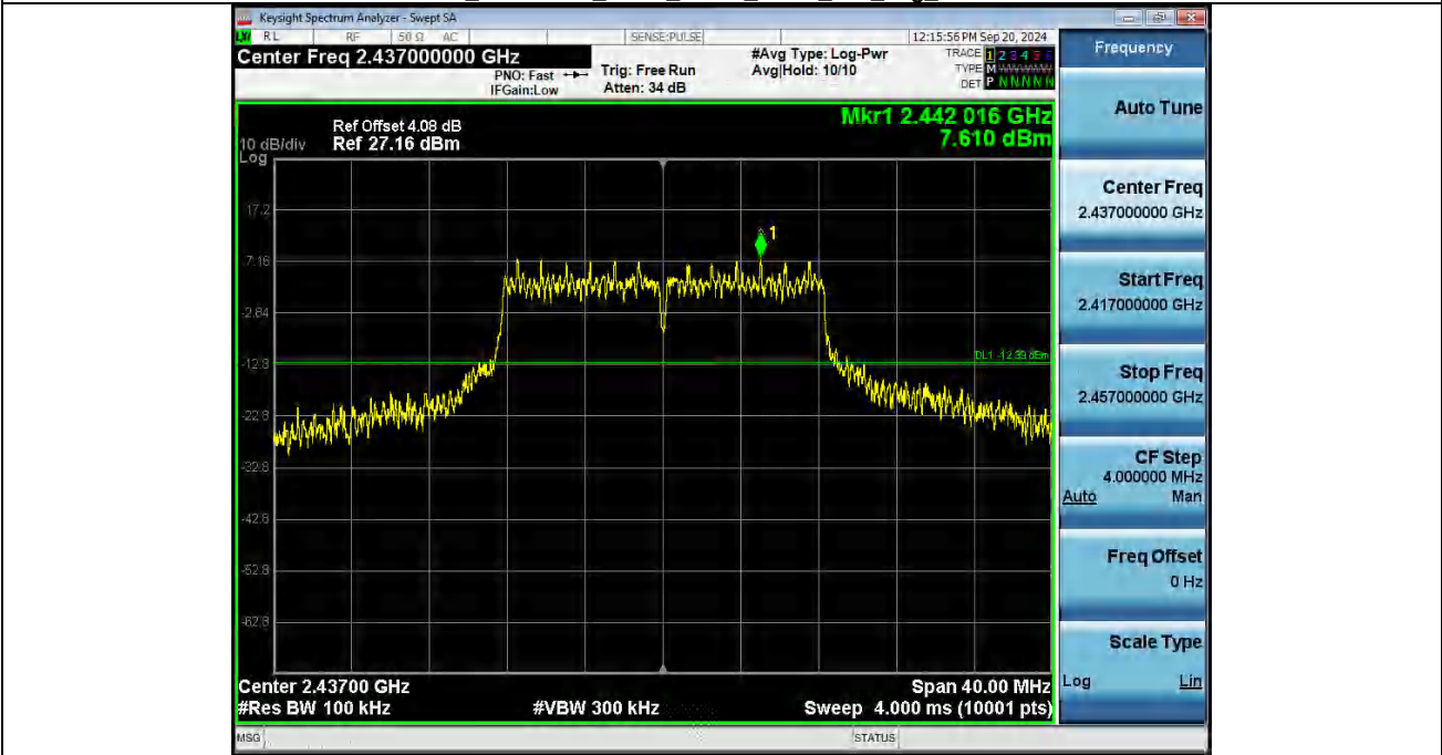
2 Spurious Emission NVNT ANT1 802 11g 2437
