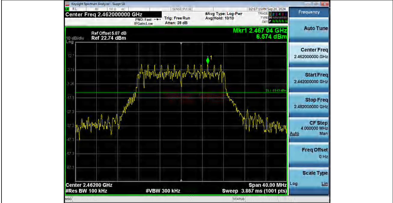
1 Reference_Level_NVNT_ANT2_802_11n(HT20)_2462
