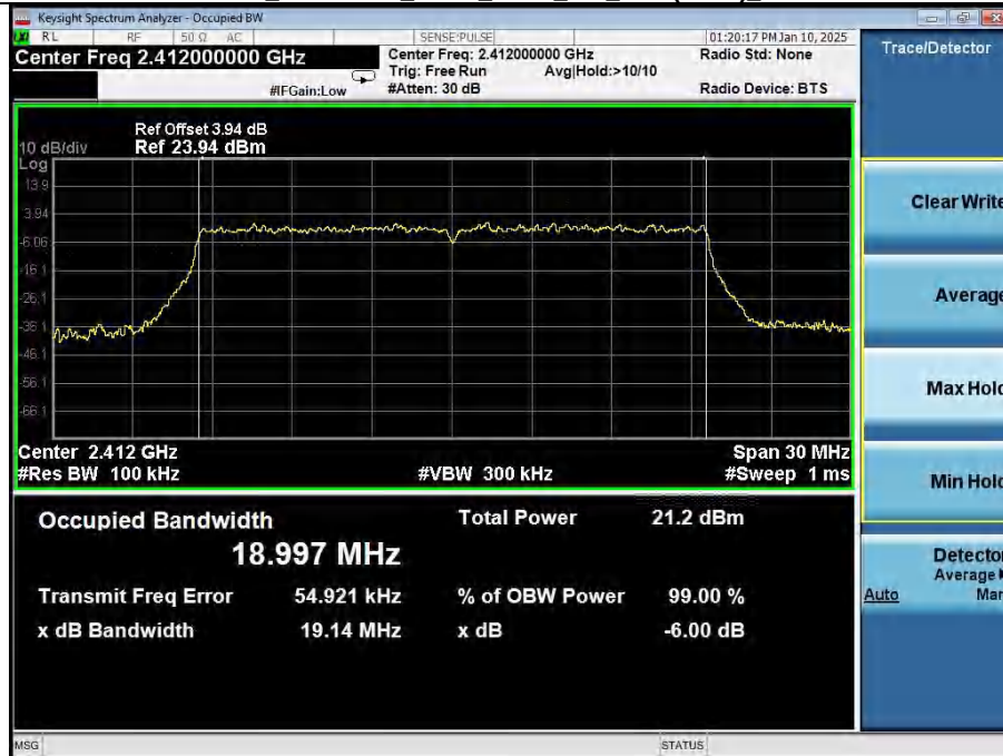
-6dB Bandwidth NVNT_ANT2_802_11ax(HE20)_2412
