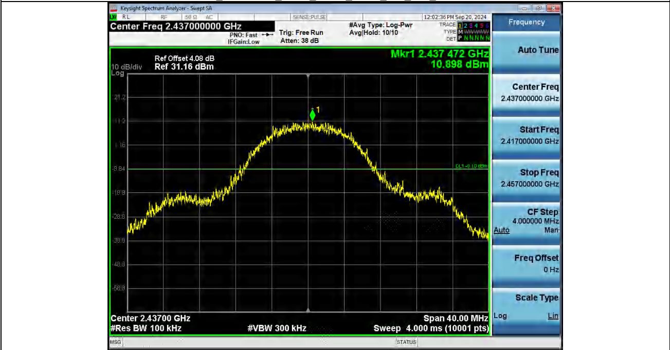
2 Spurious_Emission_NVNT_ANT1_802_11b_2437
