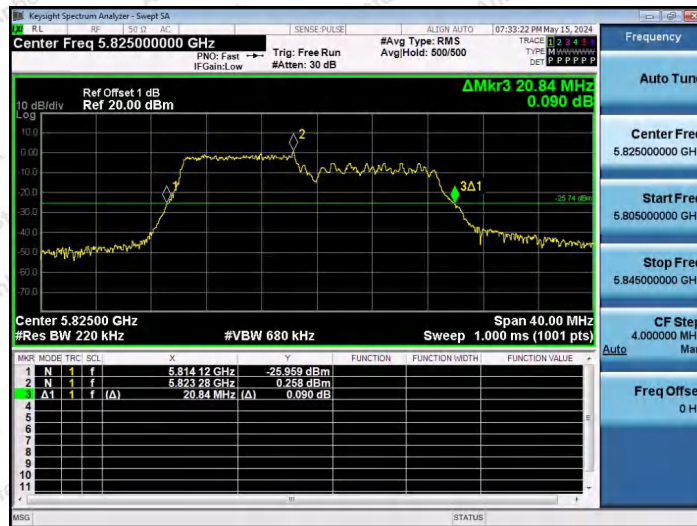
11AX20SISO-Ant1-5825-106Tone-RU53
