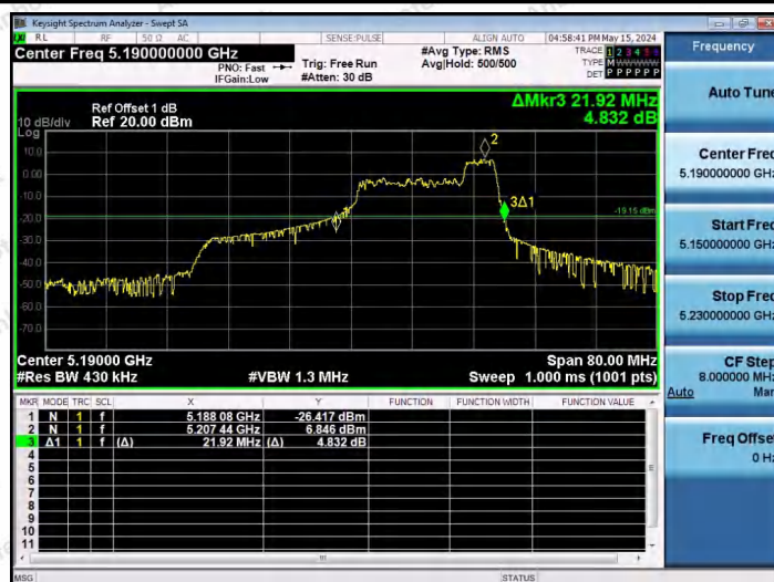
11AX40SISO-Ant1-5190-52Tone-RU44
