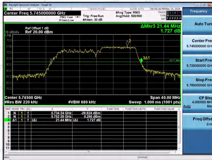
11AX20SISO-Ant1-5745-106Tone-RU54
