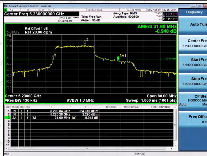
11AX40SISO-Ant1-5230-242Tone-RU61
