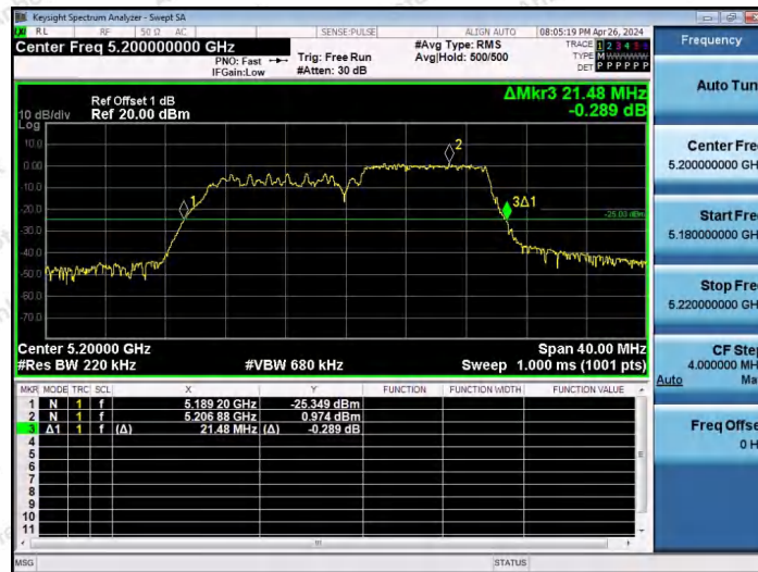
11AX20SISO-Ant1-5200-106Tone-RU54
