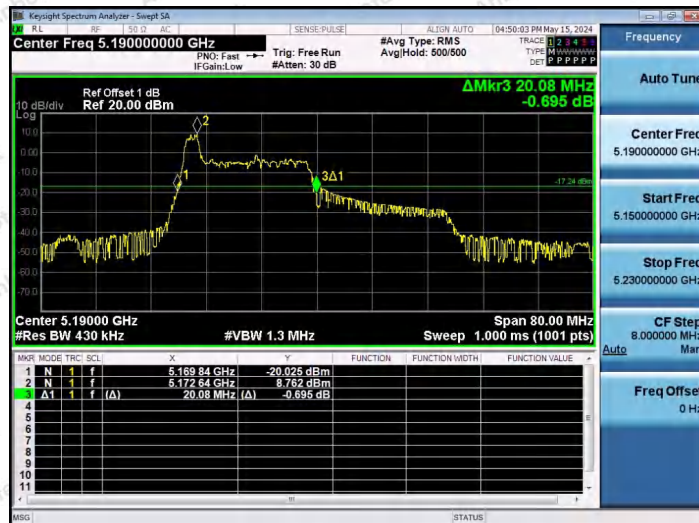
11AX40SISO-Ant1-5190-26Tone-RU0
