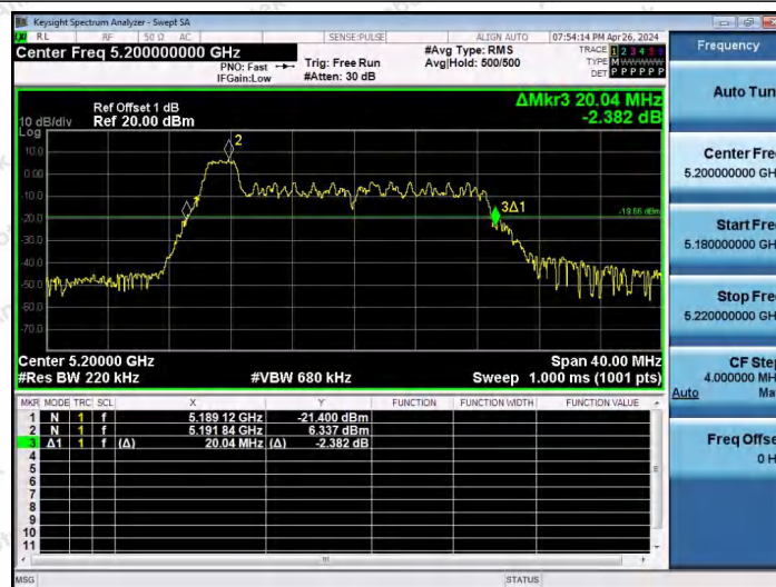
11AX20SISO-Ant1-5200-26Tone-RU0
