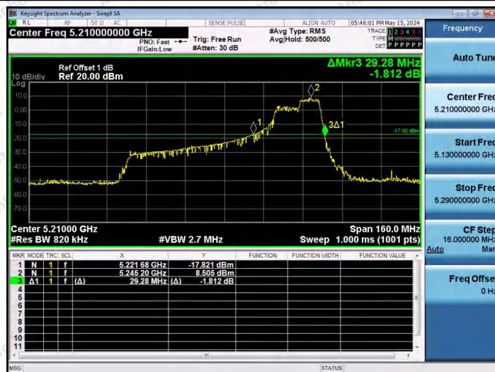
11AX80SISO-Ant1-5210-106Tone-RU60
