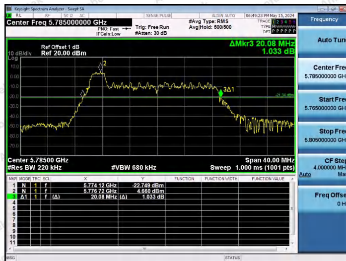
11AX20SISO-Ant1-5785-26Tone-RU0
