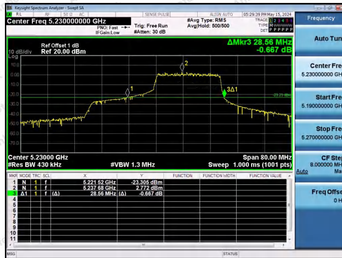
11AX40SISO-Ant1-5230-242Tone-RU62
