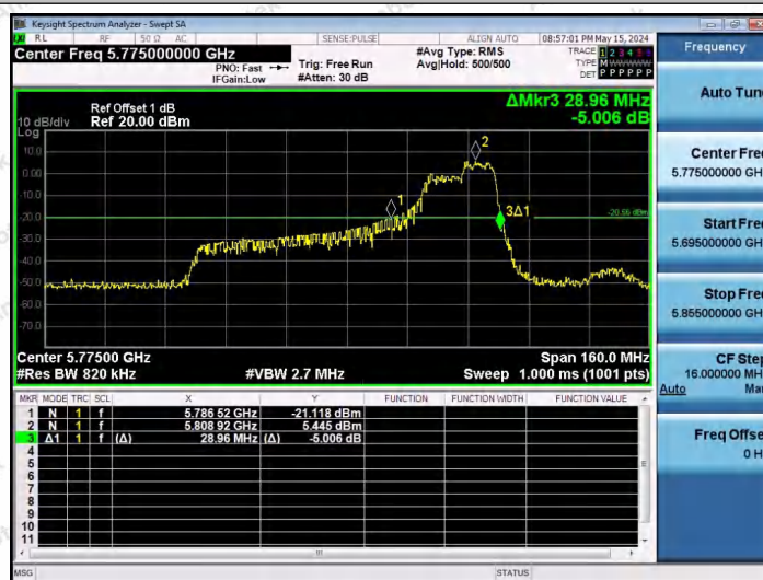
11AX80SISO-Ant1-5775-106Tone-RU60
