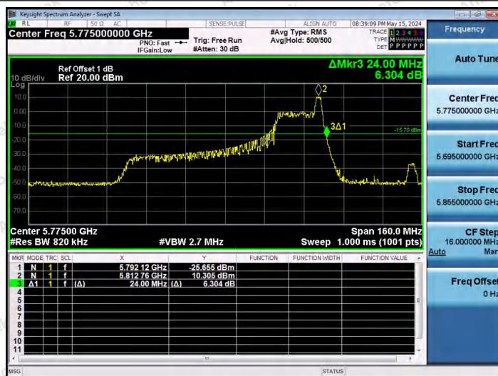
11AX80SISO-Ant1-5775-26Tone-RU36
