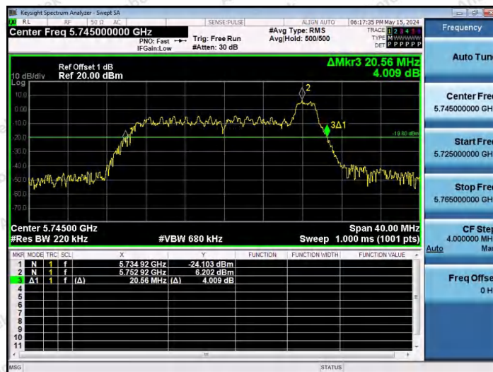
11AX20SISO-Ant1-5745-26Tone-RU8
