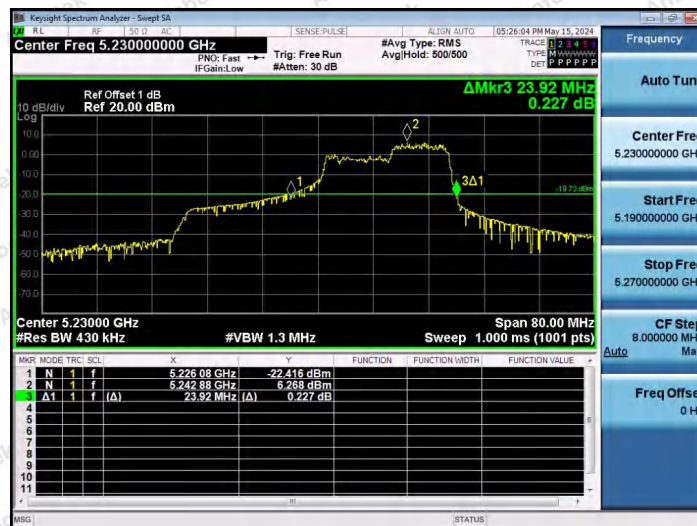
11AX40SISO-Ant1-5230-106Tone-RU56
