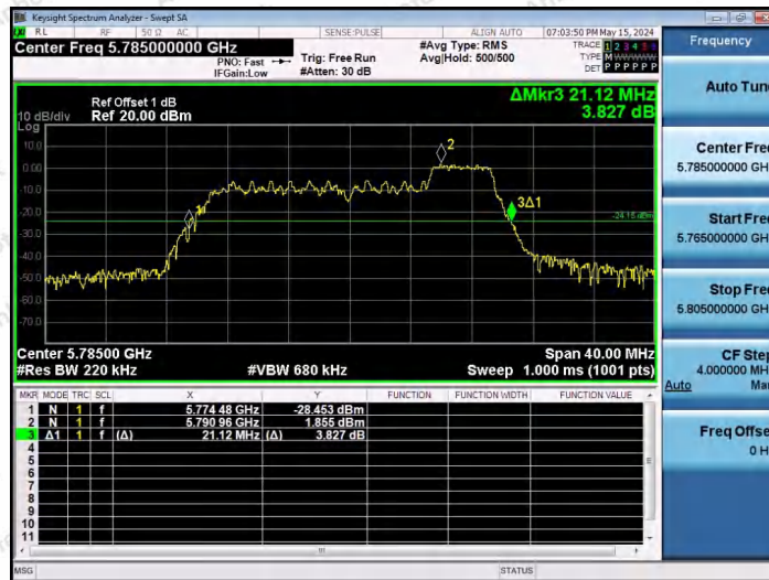
11AX20SISO-Ant1-5785-52Tone-RU40
