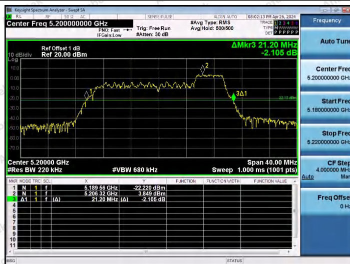
11AX20SISO-Ant1-5200-52Tone-RU40
