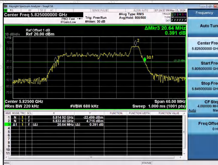
11AX20SISO-Ant1-5825-26Tone-RU8
