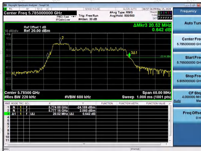
11AX20SISO-Ant1-5785-52Tone-RU37
