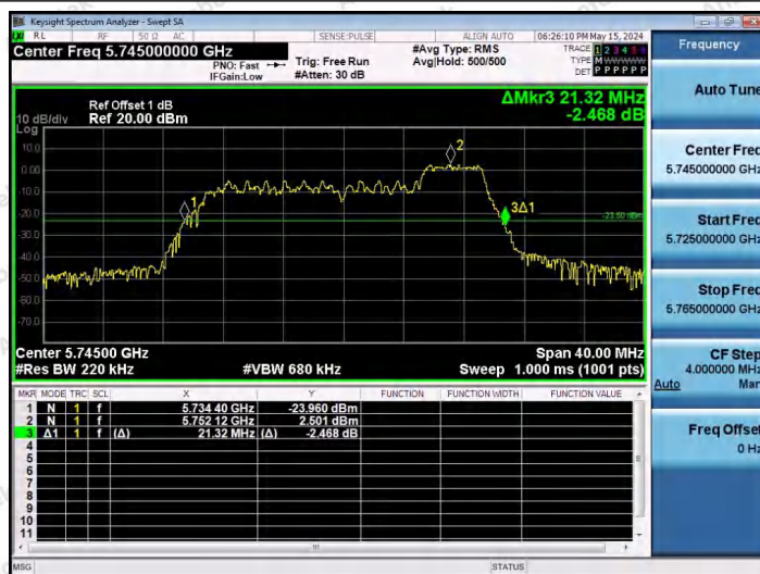
11AX20SISO-Ant1-5745-52Tone-RU40
