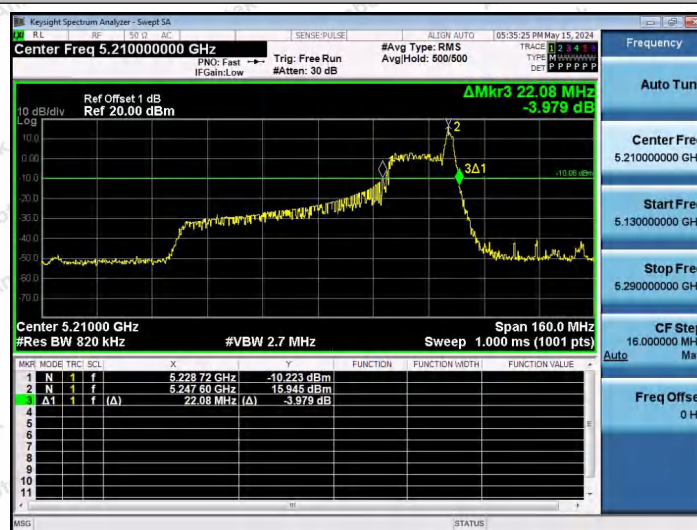
11AX80SISO-Ant1-5210-26Tone-RU36
