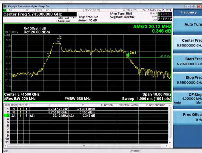
11AX20SISO-Ant1-5745-26Tone-RU0
