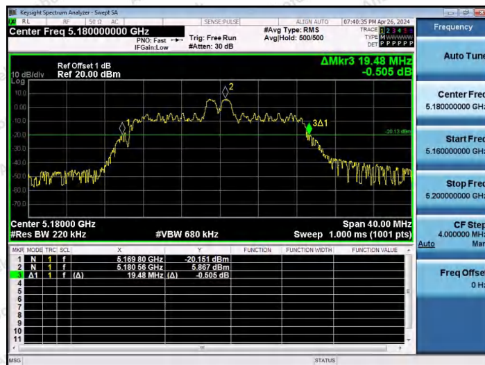
11AX20SISO-Ant1-5180-26Tone-RU4
