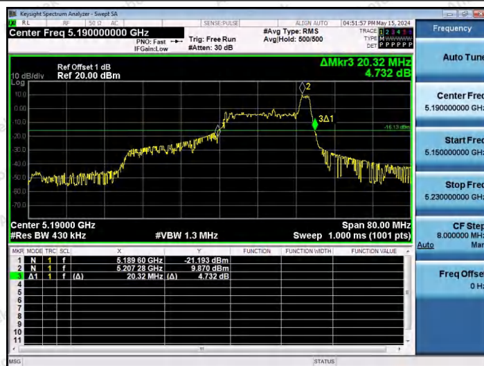
11AX40SISO-Ant1-5190-26Tone-RU17
