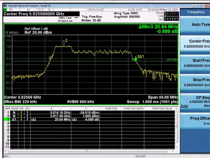
11AX20SISO-Ant1-5825-52Tone-RU37
