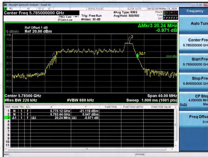
11AX20SISO-Ant1-5785-26Tone-RU8
