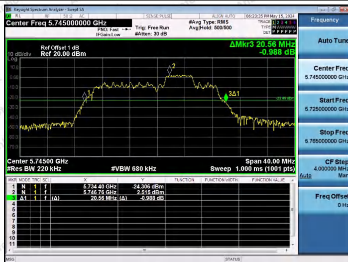
11AX20SISO-Ant1-5745-52Tone-RU39
