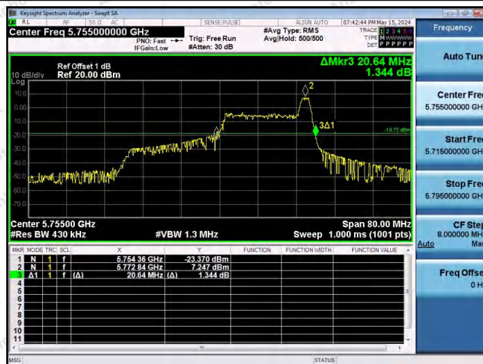
11AX40SISO-Ant1-5755-26Tone-RU17
