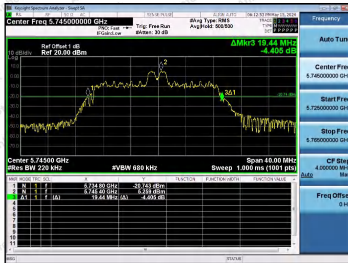
11AX20SISO-Ant1-5745-26Tone-RU4
