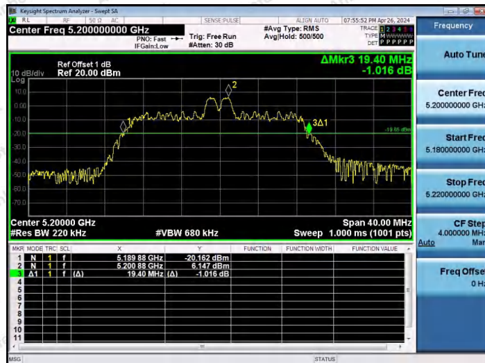
11AX20SISO-Ant1-5200-26Tone-RU4
