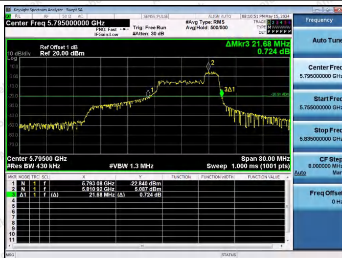
11AX40SISO-Ant1-5795-52Tone-RU44
