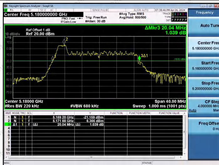
11AX20SISO-Ant1-5180-26Tone-RU0
