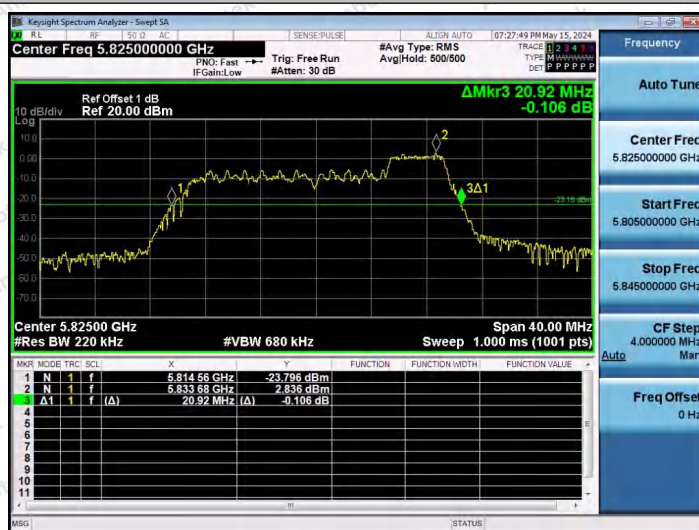
11AX20SISO-Ant1-5825-52Tone-RU40
