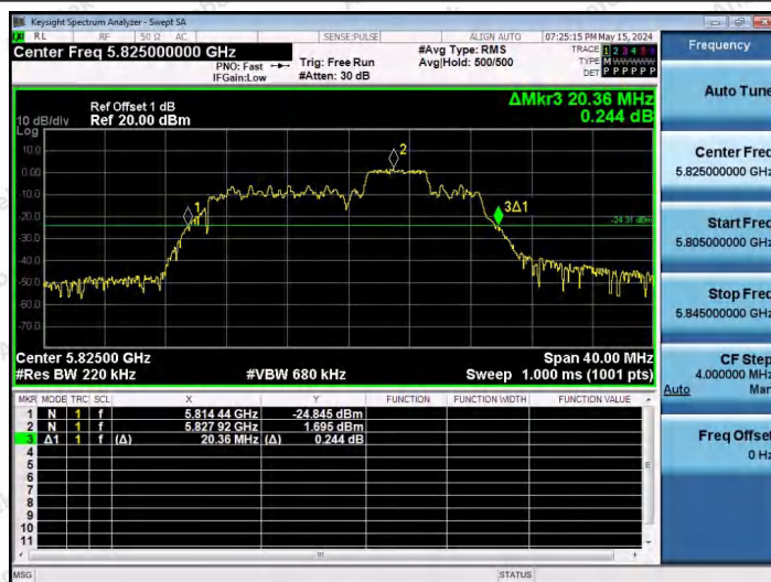
11AX20SISO-Ant1-5825-52Tone-RU39
