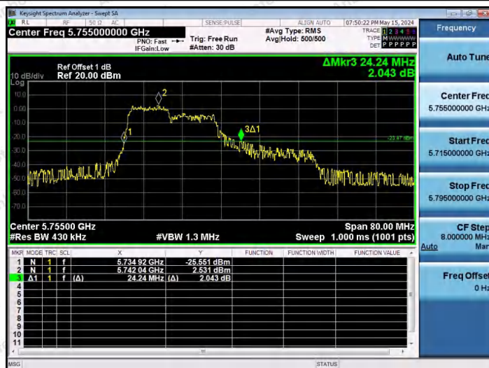
11AX40SISO-Ant1-5755-106Tone-RU53
