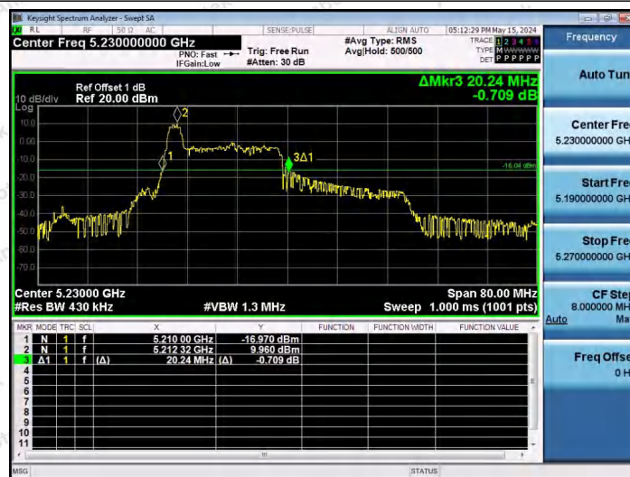
11AX40SISO-Ant1-5230-26Tone-RU0
