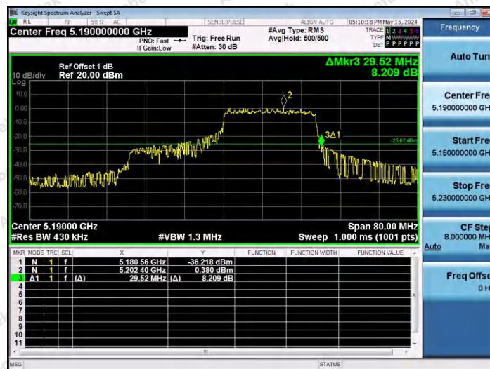
11AX40SISO-Ant1-5190-242Tone-RU62
