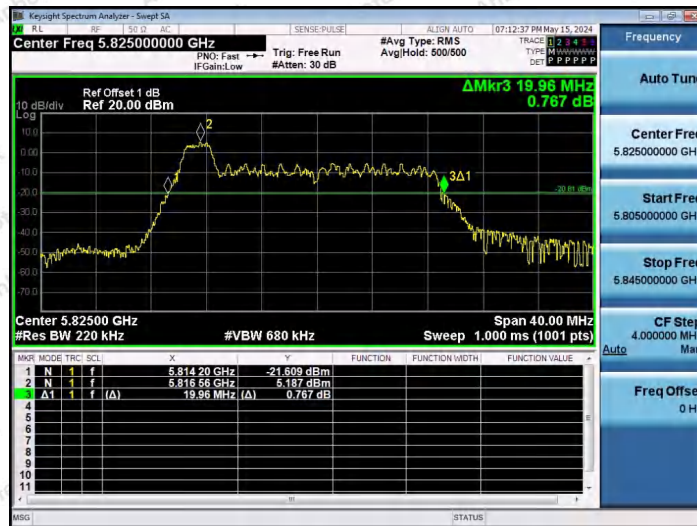
11AX20SISO-Ant1-5825-26Tone-RU0
