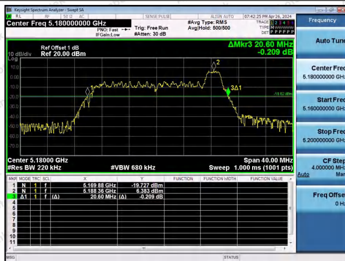
11AX20SISO-Ant1-5180-26Tone-RU8
