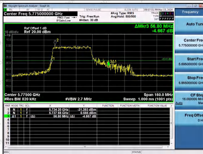
11AX80SISO-Ant1-5775-484Tone-RU65
