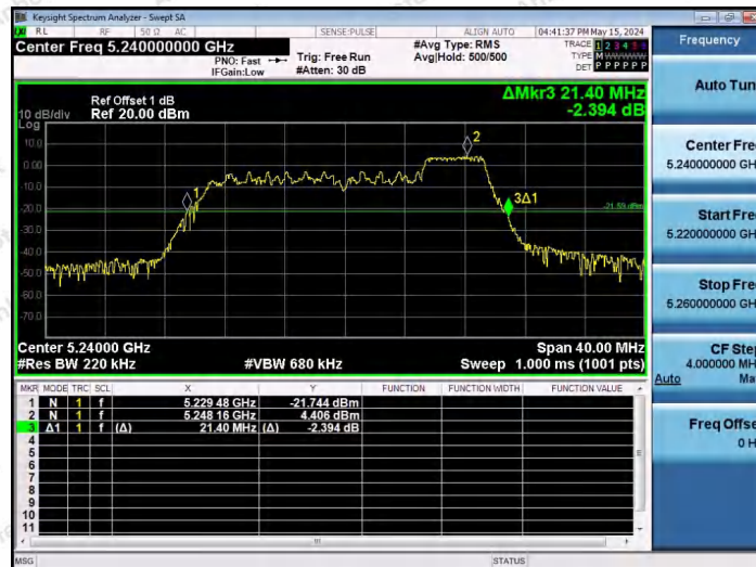
11AX20SISO-Ant1-5240-52Tone-RU40
