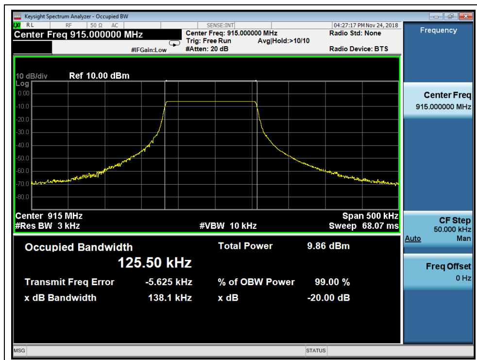
(Channel 13, 915 MHz)
