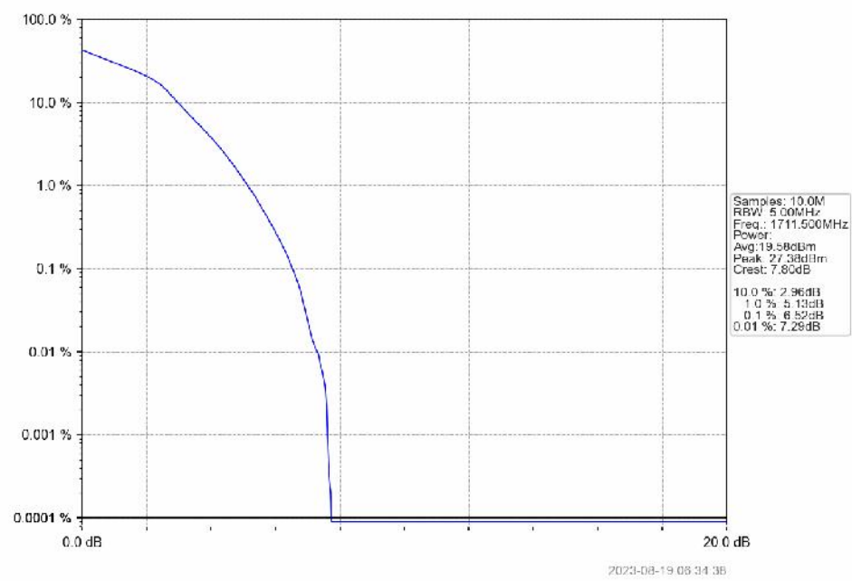
Band4_3MHz_16QAM_LCH_1711.5MHz_RB_15_0_NTNV
