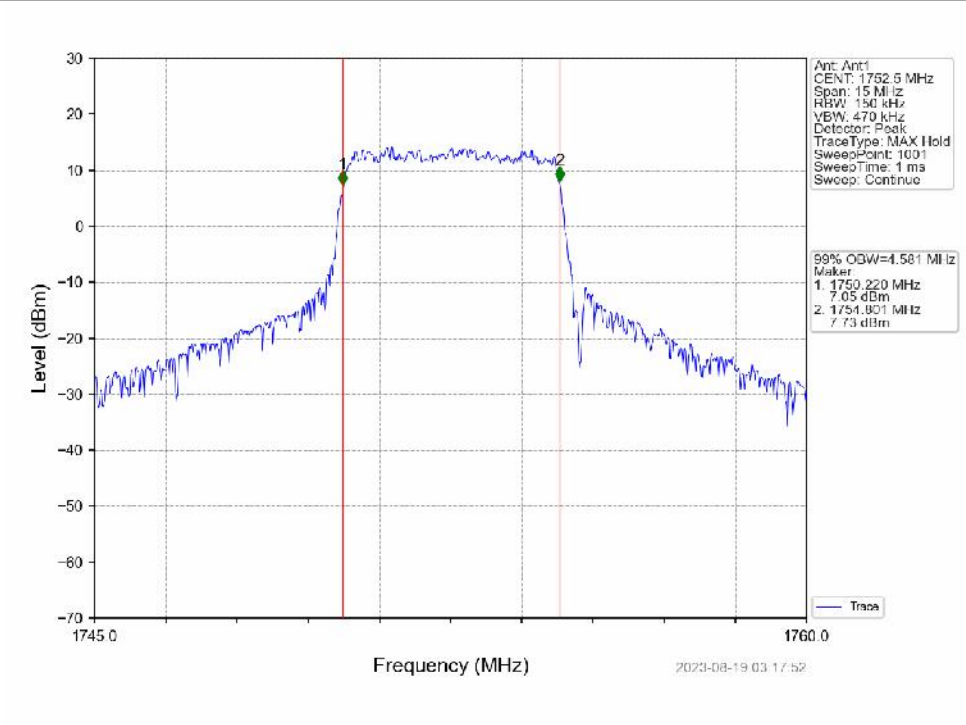
Band4_5MHz_16QAM_HCH_1752.5MHz_RB_25_0_NTNV
