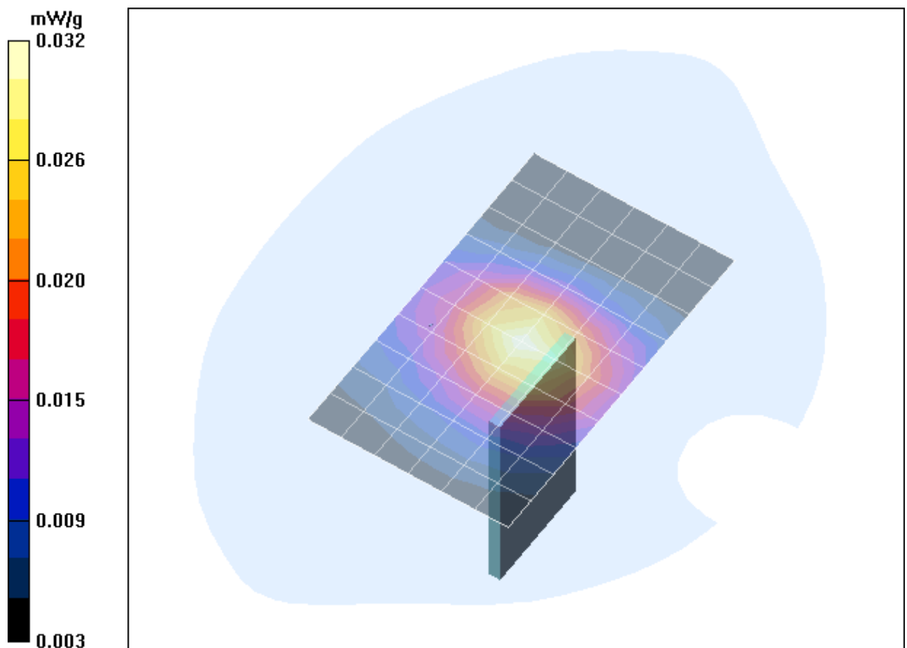
Fig. 33: SAR distribution for WCDMA V (FDD), channel 4183, position 3 (Packard Bell Easy Note , January 16, 2006; Ambient Temperature: 21.4° C; Liquid Temperature: 20.5° C).
