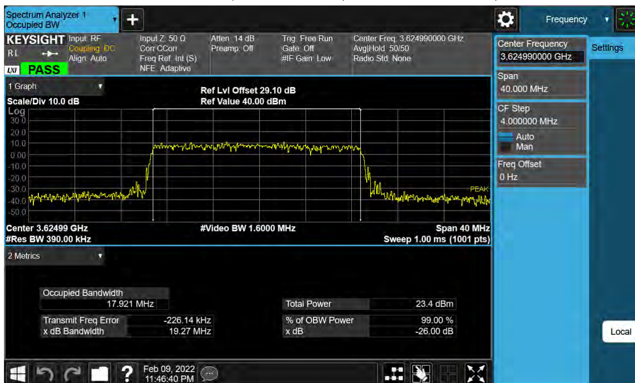
Sub6 n48. Occupied Bandwidth Plot (20 MHz Ch.641666 16-QAM)
