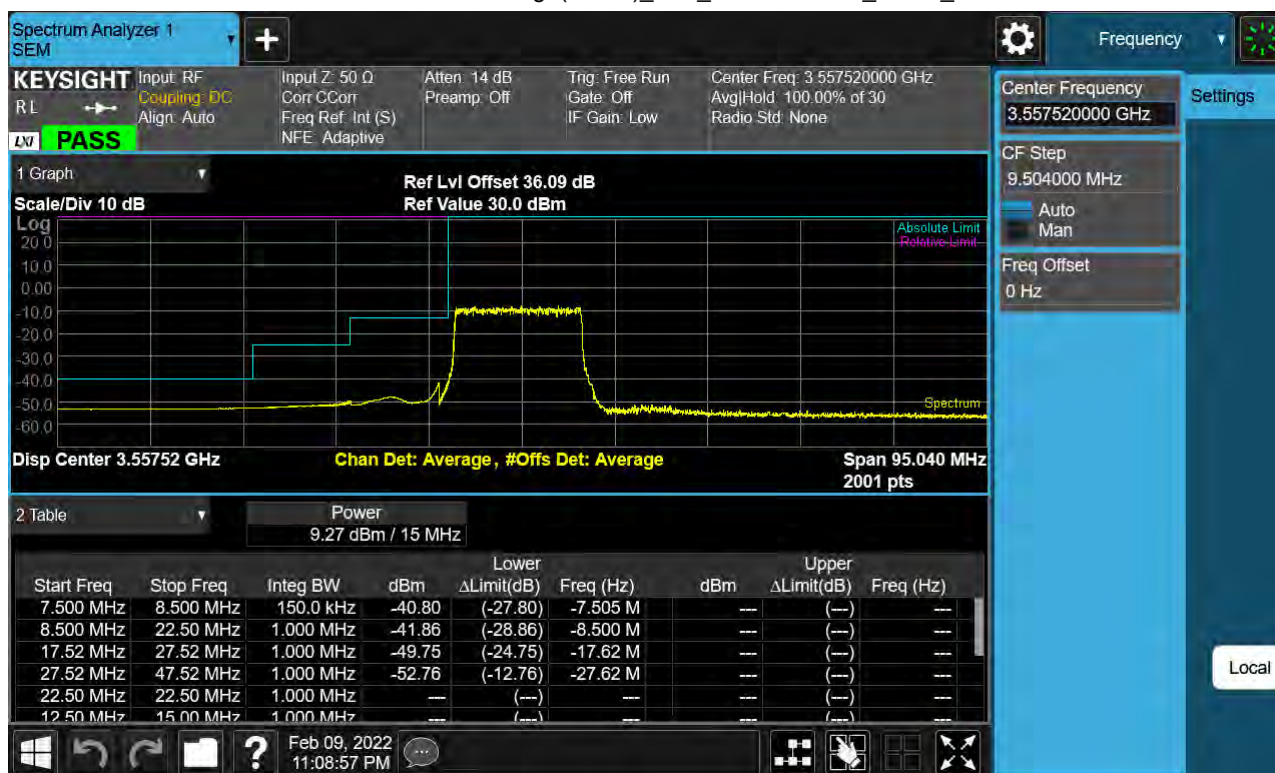
Sub6 n48. 15 M BandEdge(Lower)_Low_ 3557.52 MHz_BPSK_FullRB
