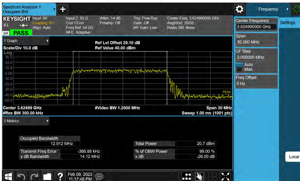
Sub6 n48. Occupied Bandwidth Plot (15 MHz Ch.641666 256-QAM)
