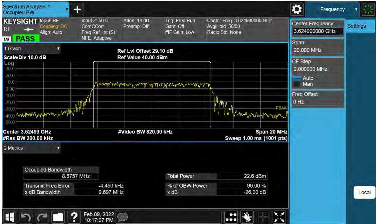
Sub6 n48. Occupied Bandwidth Plot (10 MHz Ch.641666 64-QAM)
