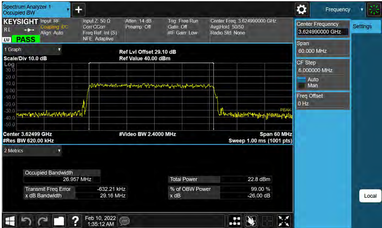
Sub6 n48. Occupied Bandwidth Plot (30 MHz Ch.641666 64-QAM)
