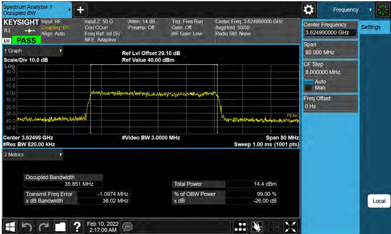
Sub6 n48. Occupied Bandwidth Plot (40 MHz Ch.641666 64-QAM)
