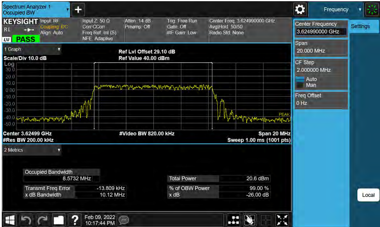
Sub6 n48. Occupied Bandwidth Plot (10 MHz Ch.641666 256-QAM)
