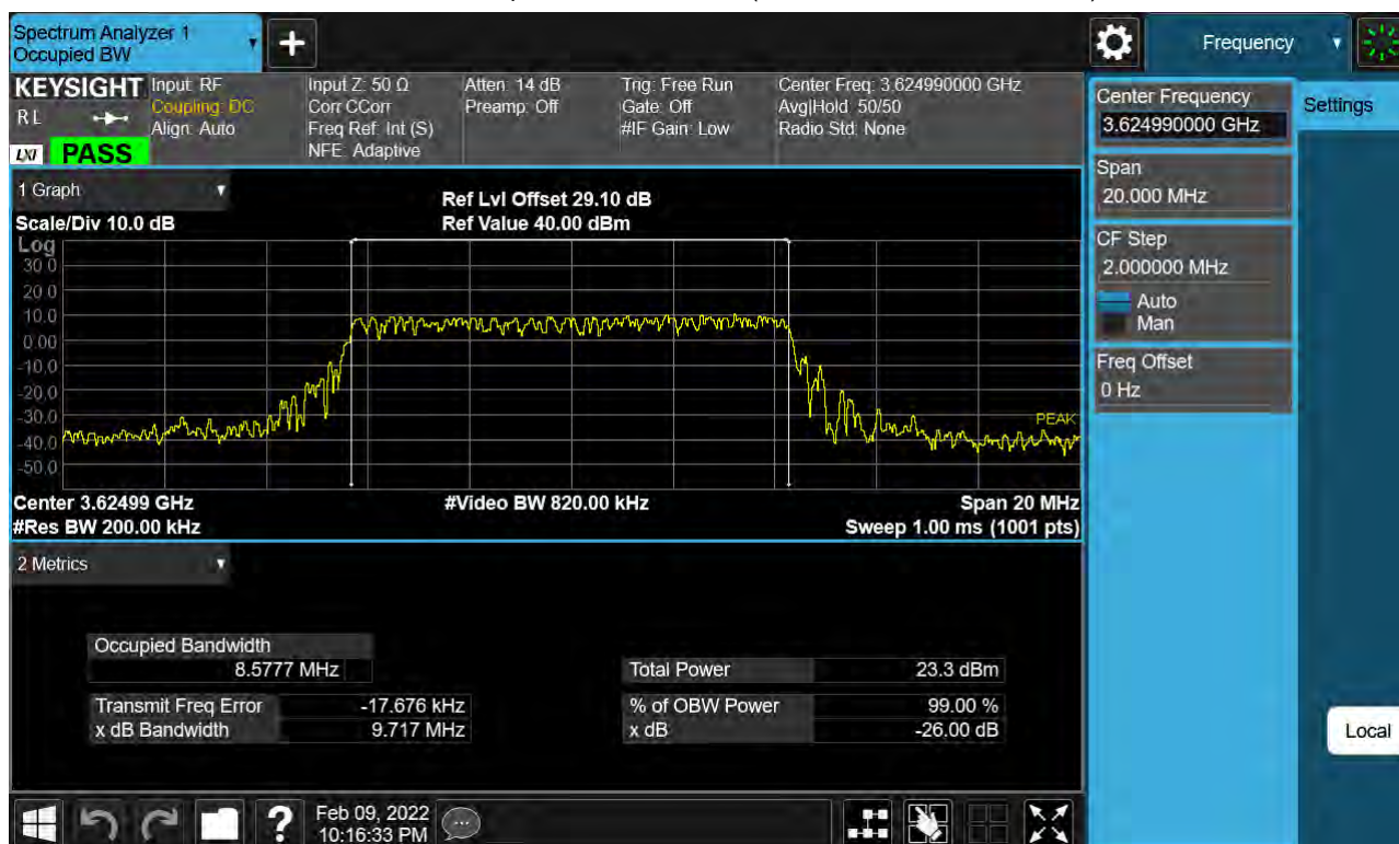
Sub6 n48. Occupied Bandwidth Plot (10 MHz Ch.641666 16-QAM)
