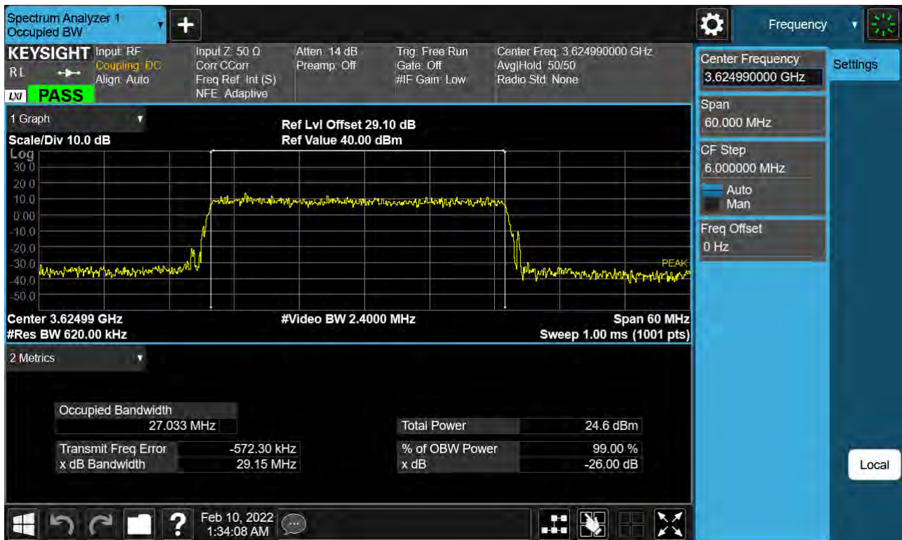
Sub6 n48. Occupied Bandwidth Plot (30 MHz Ch. 641666 QPSK)
