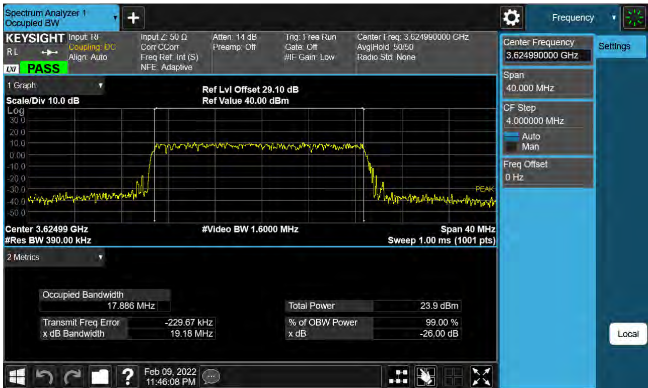
Sub6 n48. Occupied Bandwidth Plot (20 MHz Ch. 641666 QPSK)
