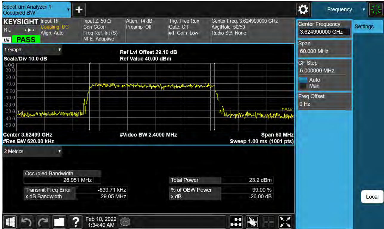
Sub6 n48. Occupied Bandwidth Plot (30 MHz Ch.641666 16-QAM)
