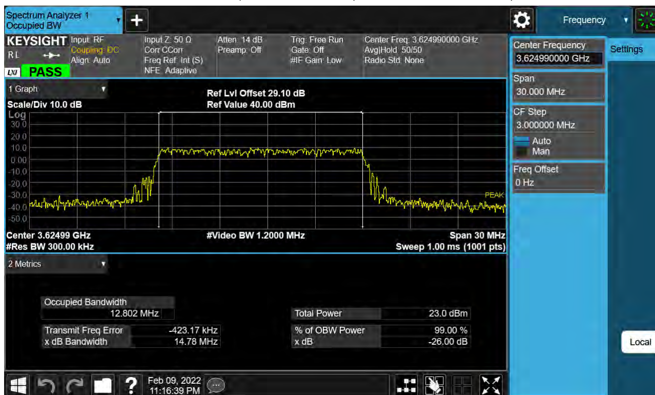
Sub6 n48. Occupied Bandwidth Plot (15 MHz Ch.641666 16-QAM)
