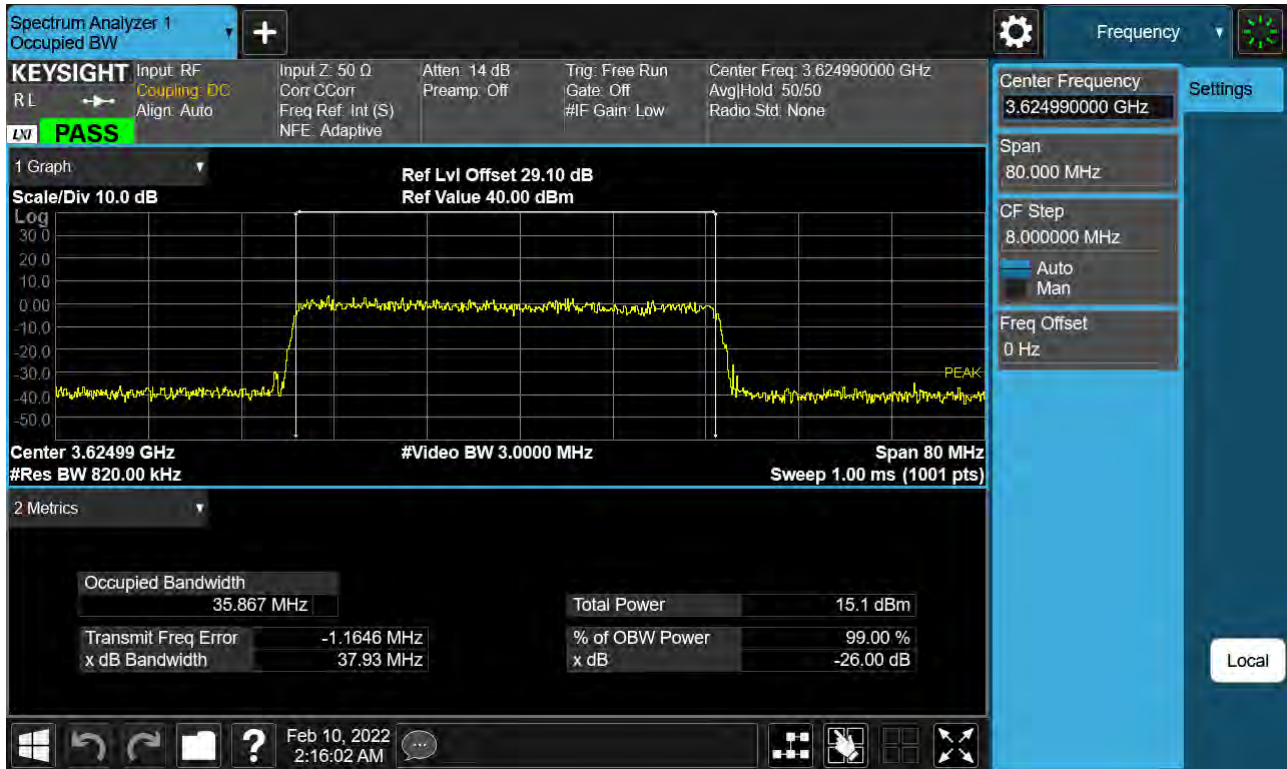
Sub6 n48. Occupied Bandwidth Plot (40 MHz Ch. 641666 QPSK)
