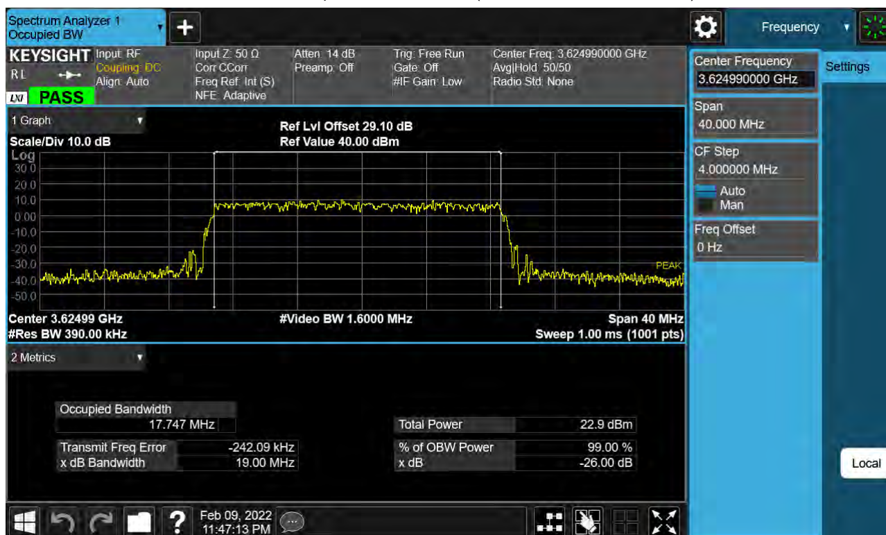
Sub6 n48. Occupied Bandwidth Plot (20 MHz Ch.641666 64-QAM)
