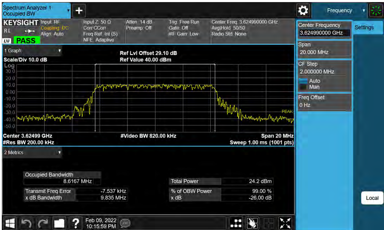
Sub6 n48. Occupied Bandwidth Plot (10 MHz Ch. 641666 QPSK)
