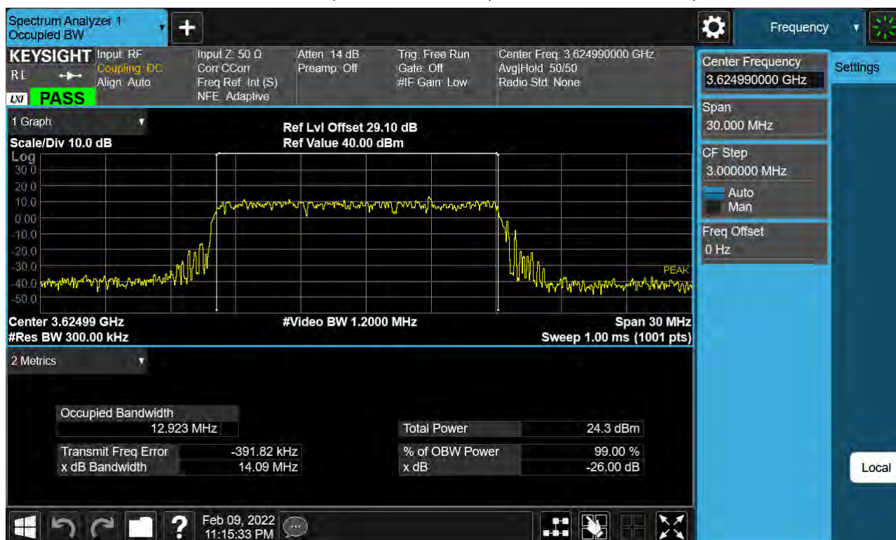
Sub6 n48. Occupied Bandwidth Plot (15 MHz Ch. 641666 BPSK)
