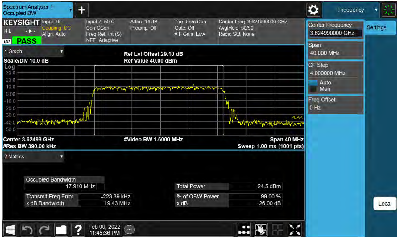
Sub6 n48. Occupied Bandwidth Plot (20 MHz Ch. 641666 BPSK)
