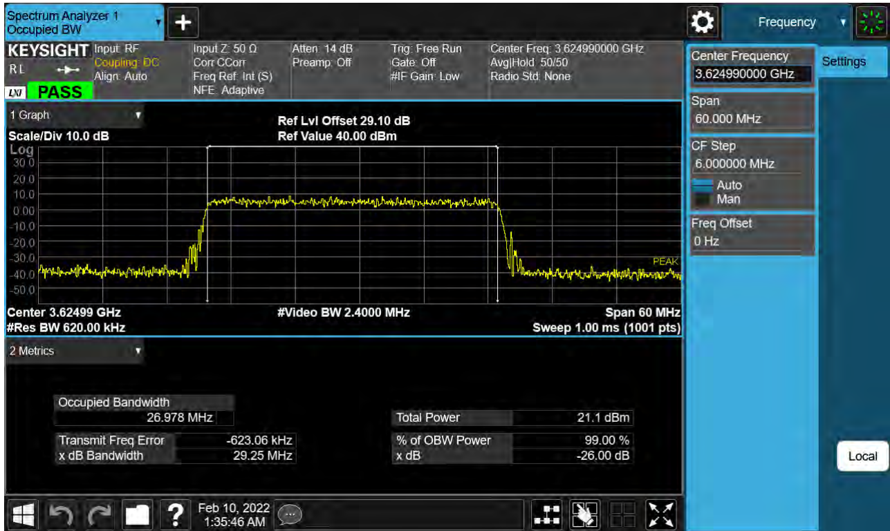
Sub6 n48. Occupied Bandwidth Plot (30 MHz Ch.641666 256-QAM)
