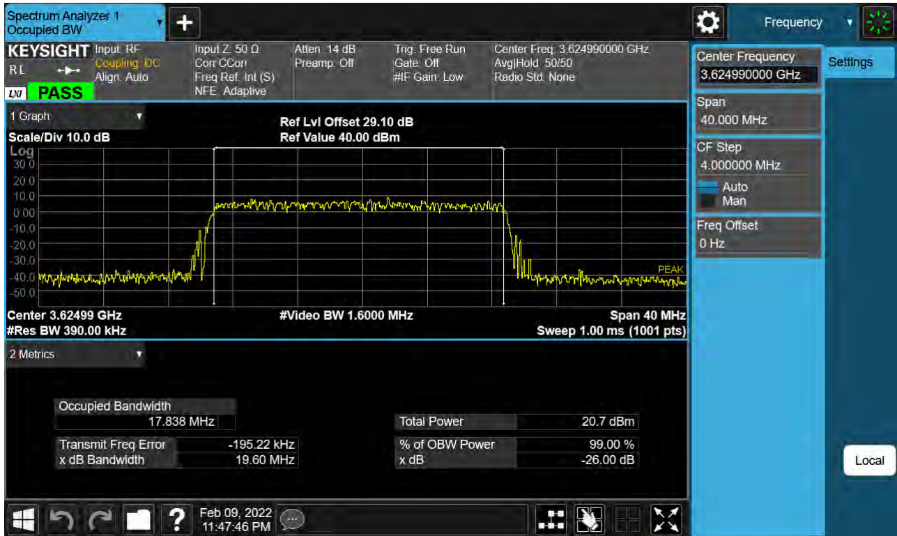
Sub6 n48. Occupied Bandwidth Plot (20 MHz Ch.641666 256-QAM)
