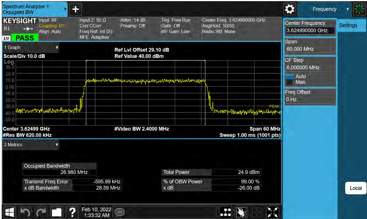
Sub6 n48. Occupied Bandwidth Plot (30 MHz Ch. 641666 BPSK)
