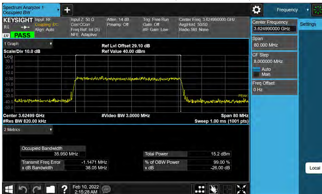
Sub6 n48. Occupied Bandwidth Plot (40 MHz Ch. 641666 BPSK)
