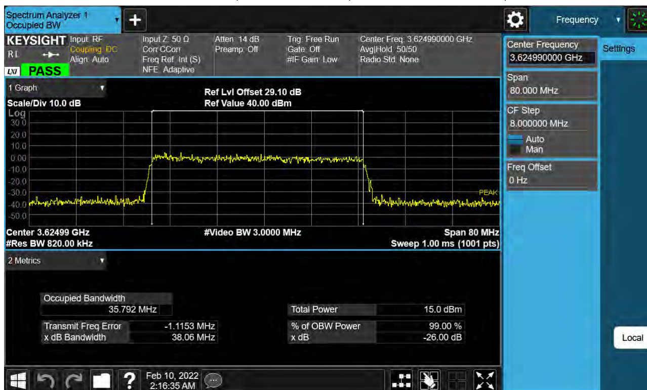
Sub6 n48. Occupied Bandwidth Plot (40 MHz Ch.641666 16-QAM)
