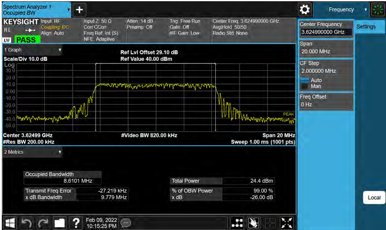
Sub6 n48. Occupied Bandwidth Plot (10 MHz Ch. 641666 BPSK)
