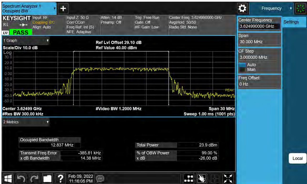
Sub6 n48. Occupied Bandwidth Plot (15 MHz Ch. 641666 QPSK)
