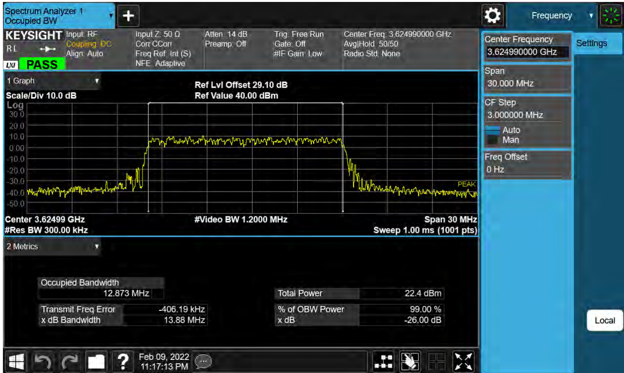
Sub6 n48. Occupied Bandwidth Plot (15 MHz Ch.641666 64-QAM)
